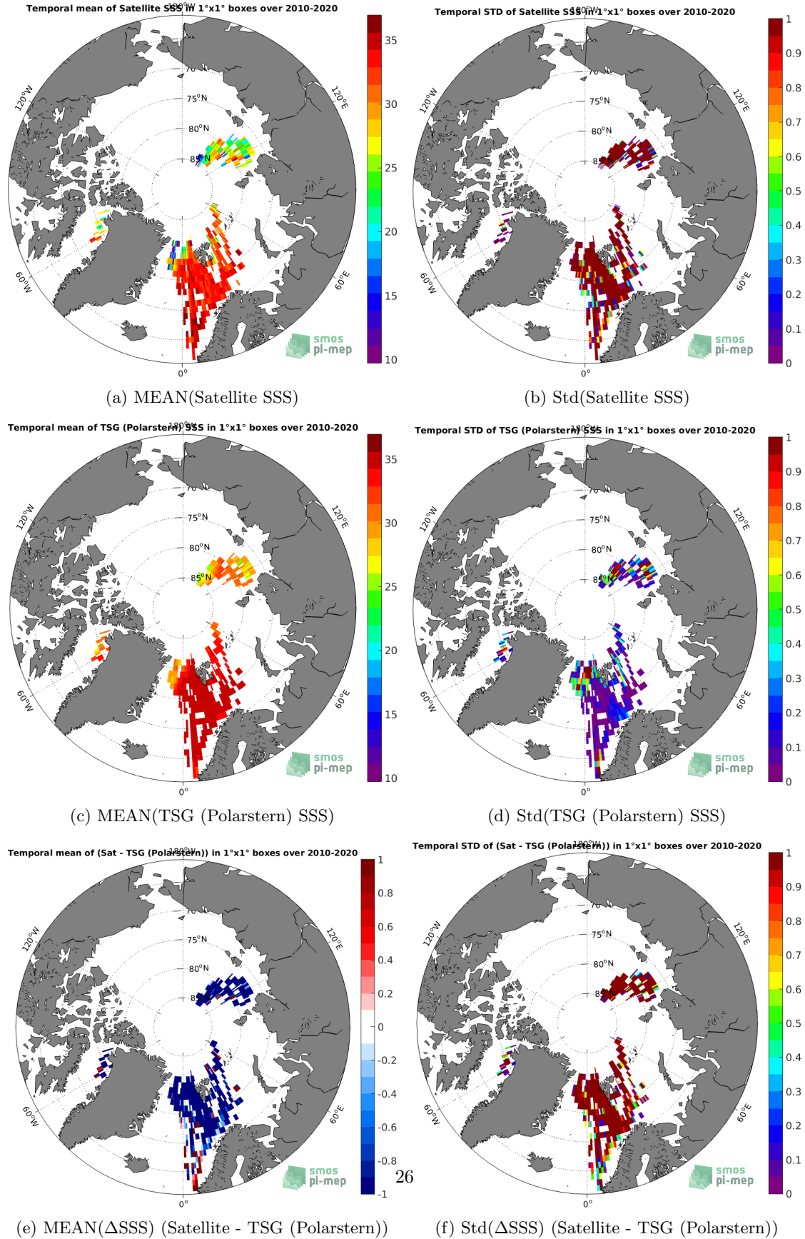
Figure 6: Temporal mean (left) and Std (right) of SSS from SMOS SSS L2 v700 (ESA) (top), TSG (Polarstern) (middle), and of \Delta SSS (Satellite - TSG (Polarstern)). Only match-up pairs are used to generate these maps.
