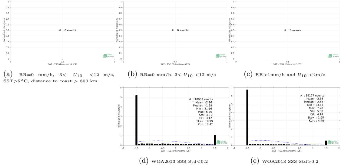
Figure 13: Normalized histogram of \Delta\text{SSS} (SMOS SSS L2 v700 (ESA) - TSG (Polarstern)) for 5 different subdatasets corresponding to: RR=0 mm/h, 3 < U_{10} < 12 m/s, SST > 5^\circ\text{C} , distance to coast > 800 km (a), RR=0 mm/h, 3 < U_{10} < 12 m/s (b), RR > 1 mm/h and U_{10} < 4 m/s (c), WOA2013 SSS Std < 0.2 (d), WOA2013 SSS Std > 0.2 (e).
