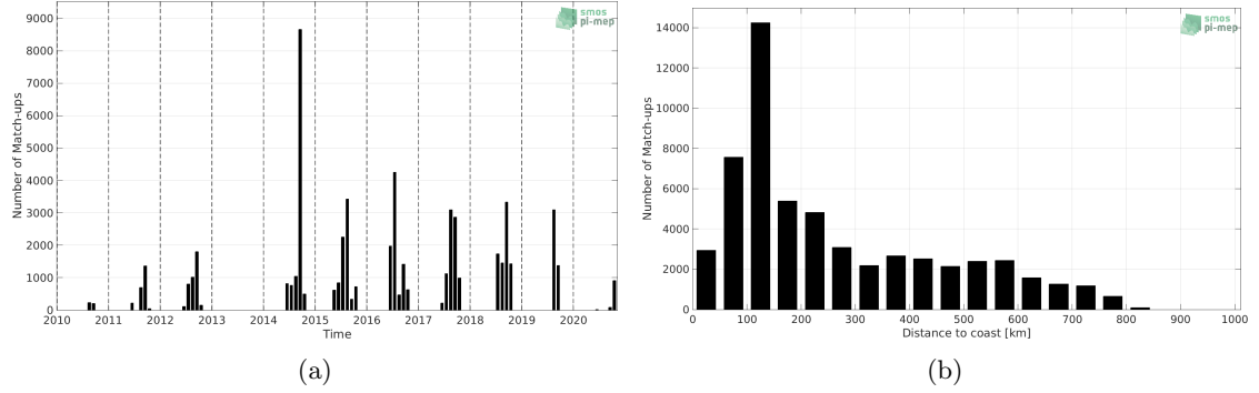
Figure 1: Number of match-ups between TSG (Polarstern) and SMOS SSS L2 v700 (ESA) SSS as a function of time (a) and as function of the distance to coast (b) over the Arctic Ocean Pi-MEP region and for the full satellite product period.
