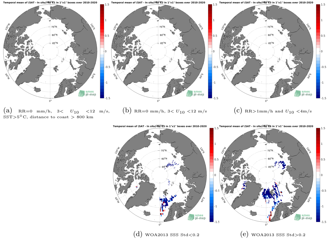
Figure 12: Temporal mean gridded over spatial boxes of size 1^{\circ}\times 1^{\circ} of \Delta\text{SSS} (SMOS SSS L2 v700 (ESA) - TSG (Polarstern)) for 5 different subdatasets corresponding to:RR=0 mm/h, 3 < U_{10} < 12 m/s, SST >5^{\circ}\text{C} , distance to coast > 800 km (a), RR=0 mm/h, 3 < U_{10} < 12 m/s (b), RR >1 mm/h and U_{10} < 4 m/s (c), WOA2013 SSS Std <0.2 (d), WOA2013 SSS Std >0.2 (e).
