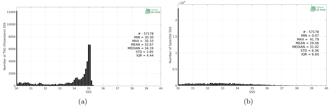
Figure 2: Histograms of SSS from TSG (Polarstern) (a) and SMOS SSS L2 v700 (ESA) (b) considering all match-up pairs per bins of 0.1 over the Arctic Ocean Pi-MEP region and for the full satellite product period.
