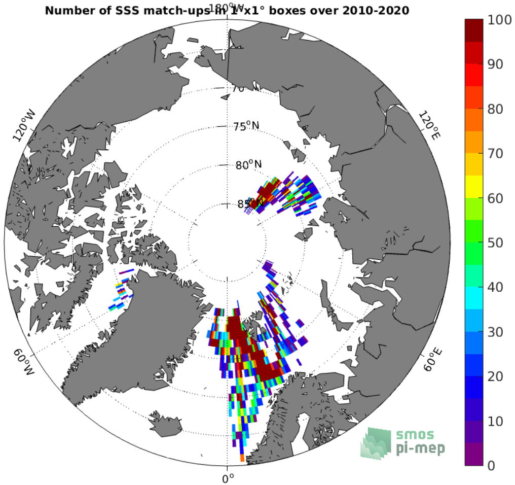
Figure 4: Number of SSS match-ups between TSG (Polarstern) SSS and the SMOS SSS L2 v700 (ESA) SSS product for the Arctic Ocean Pi-MEP region over 1^\circ \times 1^\circ boxes and for the full satellite product period.
