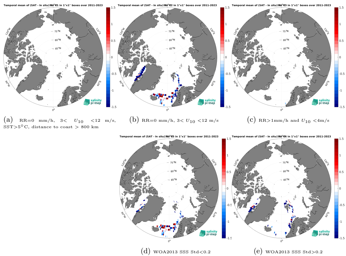
Figure 14: Temporal mean gridded over spatial boxes of size 1^\circ \times 1^\circ of \Delta\text{SSS} (SMOS SSS L2 v700 (ESA) - TSG (LEGOS-DM)) for 5 different subdatasets corresponding to:RR=0 mm/h, 3 < U_{10} < 12 m/s, SST>5°C, distance to coast > 800 km (a), RR=0 mm/h, 3 < U_{10} < 12 m/s (b), RR>1mm/h and U_{10} < 4 m/s (c), WOA2013 SSS Std<0.2 (d), WOA2013 SSS Std>0.2 (e).
