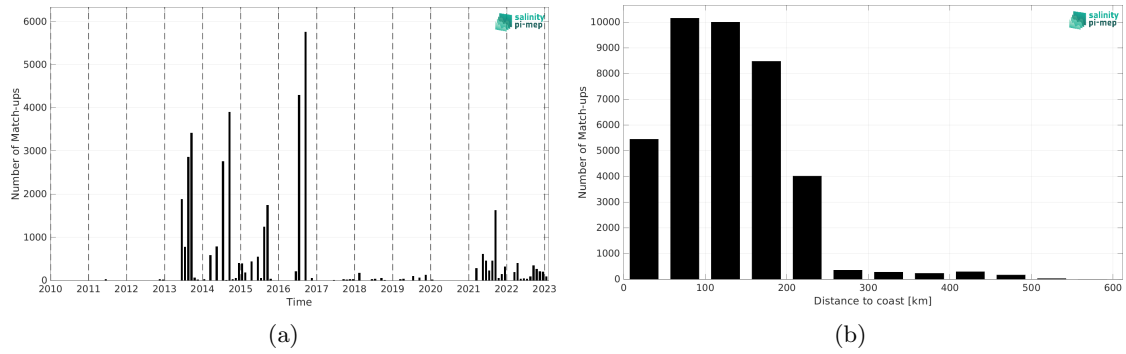
Figure 2: Number of match-ups between TSG (LEGOS-DM) and SMOS SSS L2 v700 (ESA) SSS as a function of time (a) and as function of the distance to coast (b) over the Arctic Ocean Pi-MEP region and for the full satellite product period.
