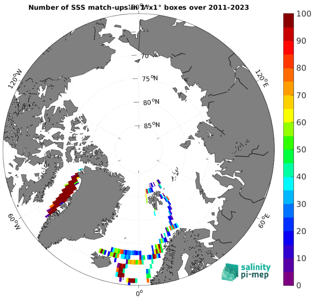
Figure 5: Number of SSS match-ups between TSG (LEGOS-DM) SSS and the SMOS SSS L2 v700 (ESA) SSS product for the Arctic Ocean Pi-MEP region over 1^\circ \times 1^\circ boxes and for the full satellite product period.
