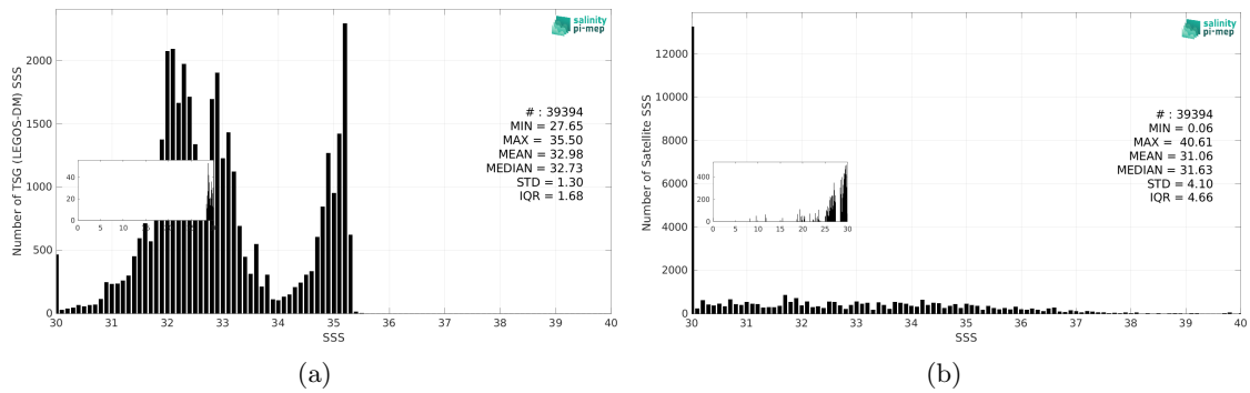
Figure 3: Histograms of SSS from TSG (LEGOS-DM) (a) and SMOS SSS L2 v700 (ESA) (b) considering all match-up pairs per bins of 0.1 over the Arctic Ocean Pi-MEP region and for the full satellite product period.
