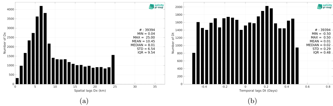
Figure 6: Histograms of the spatial (a) and temporal (b) lags between the location/time of the TSG (LEGOS-DM) measurement and the date of the corresponding SMOS SSS L2 v700 (ESA) SSS pixel.
