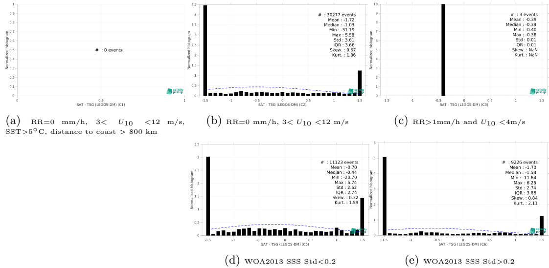
Figure 15: Normalized histogram of \Delta SSS (SMOS SSS L2 v700 (ESA) - TSG (LEGOS-DM)) for 5 different subdatasets corresponding to: RR=0 mm/h, 3 < U_{10} < 12 m/s, SST > 5°C, distance to coast > 800 km (a), RR=0 mm/h, 3 < U_{10} < 12 m/s (b), RR > 1mm/h and U_{10} < 4 m/s (c), WOA2013 SSS Std < 0.2 (d), WOA2013 SSS Std > 0.2 (e).
