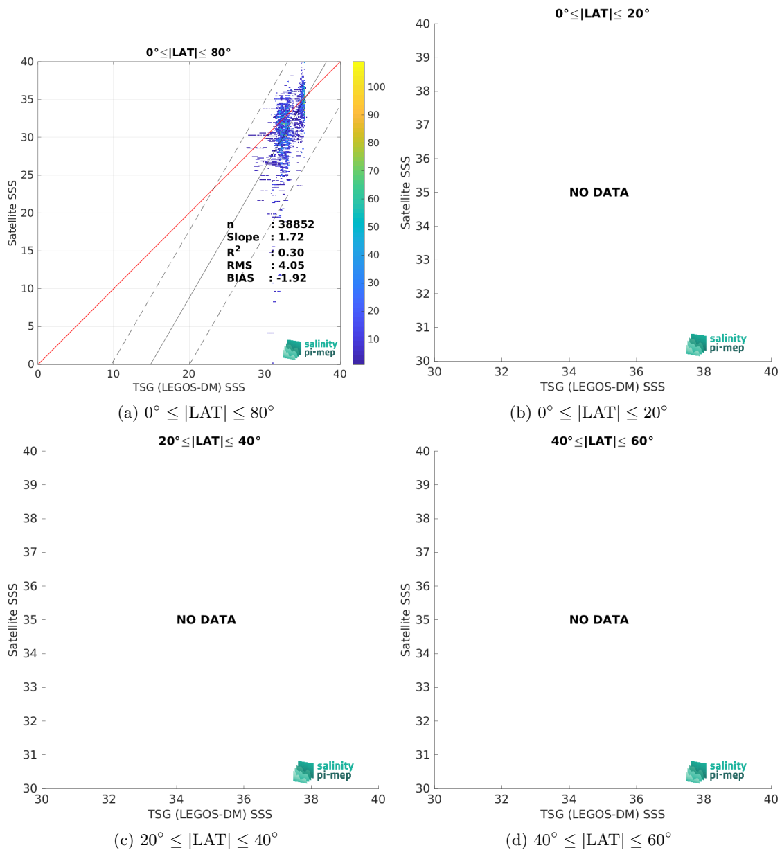
Figure 10: Contour maps of the concentration of SMOS SSS L2 v700 (ESA) SSS (y-axis) versus TSG (LEGOS-DM) SSS (x-axis) at match-up pairs for different latitude bands. For each plot, the red line shows x=y . The black thin and dashed lines indicate a linear fit through the data cloud and the \pm 95\% confidence levels, respectively. The number match-up pairs n , the slope and R^2 coefficient of the linear fit, the root mean square (RMS) and the mean bias between satellite and in situ data are indicated for each latitude band in each plots.
