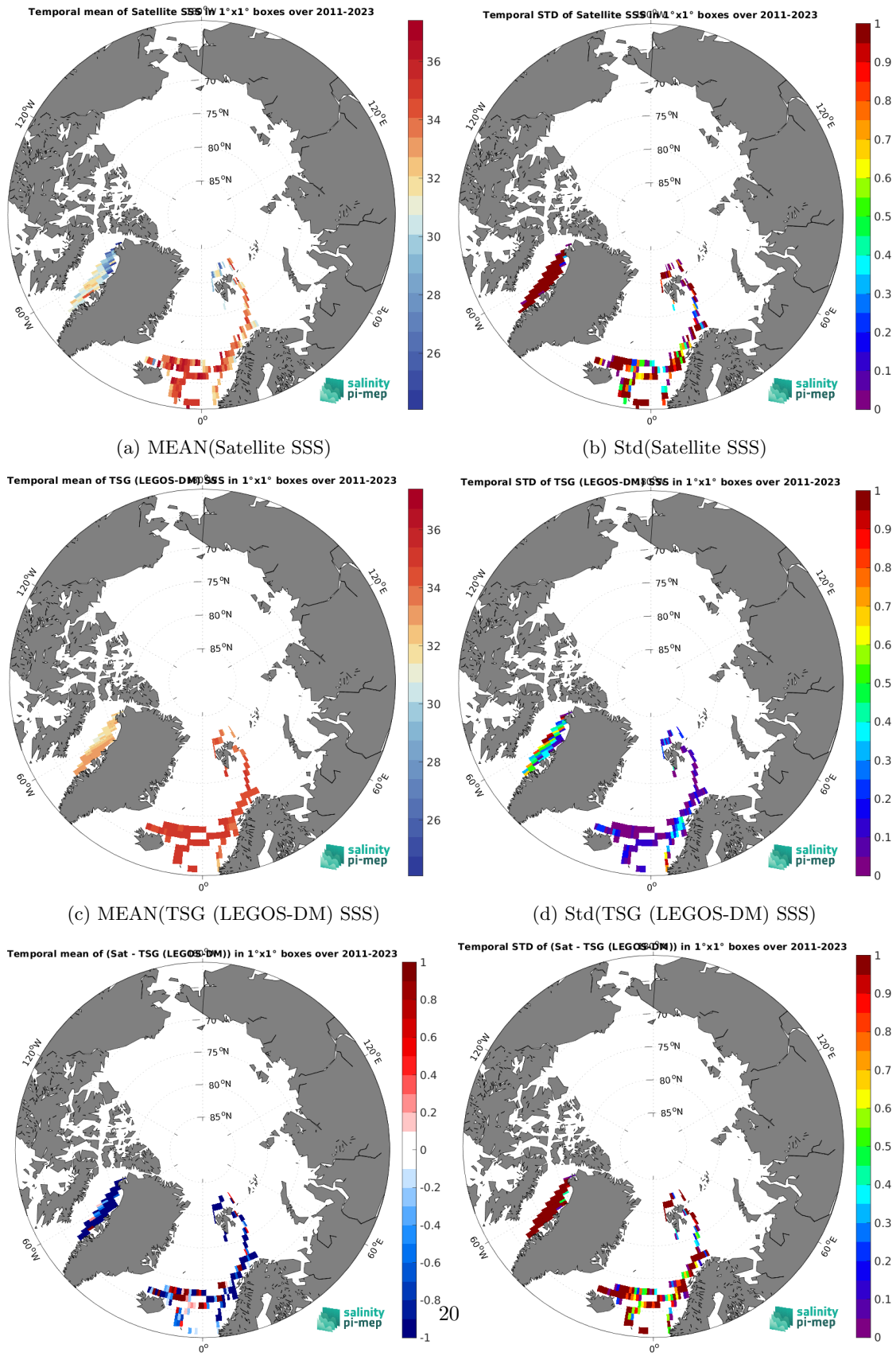
Figure 7: Temporal mean (left) and Std (right) of SSS from SMOS SSS L2 v700 (ESA) (top), TSG (LEGOS-DM) (middle), and of \Delta SSS (Satellite - TSG (LEGOS-DM)). Only match-up pairs are used to generate these maps.
