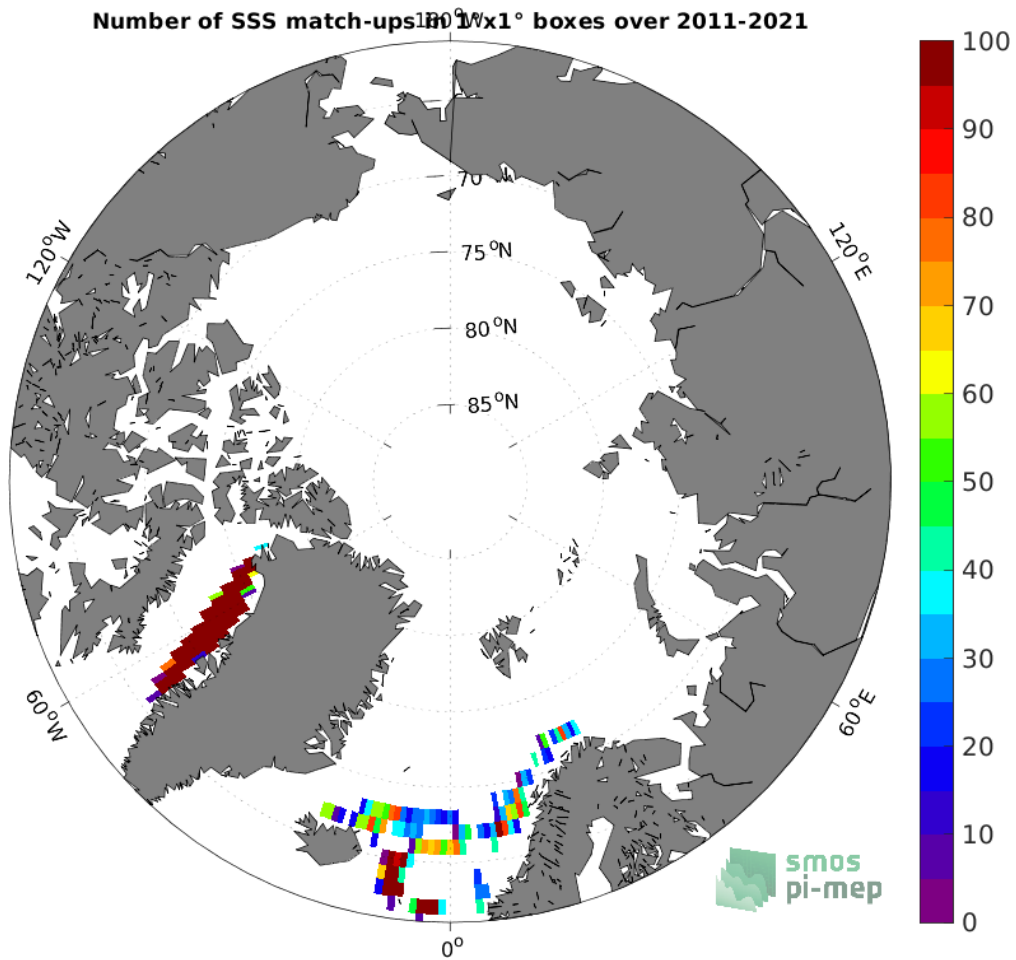
Figure 4: Number of SSS match-ups between TSG (LEGOS-DM) SSS and the SMOS SSS L2 v700 (ESA) SSS product for the Arctic Ocean Pi-MEP region over 1^{\circ} \times 1^{\circ} boxes and for the full satellite product period.
