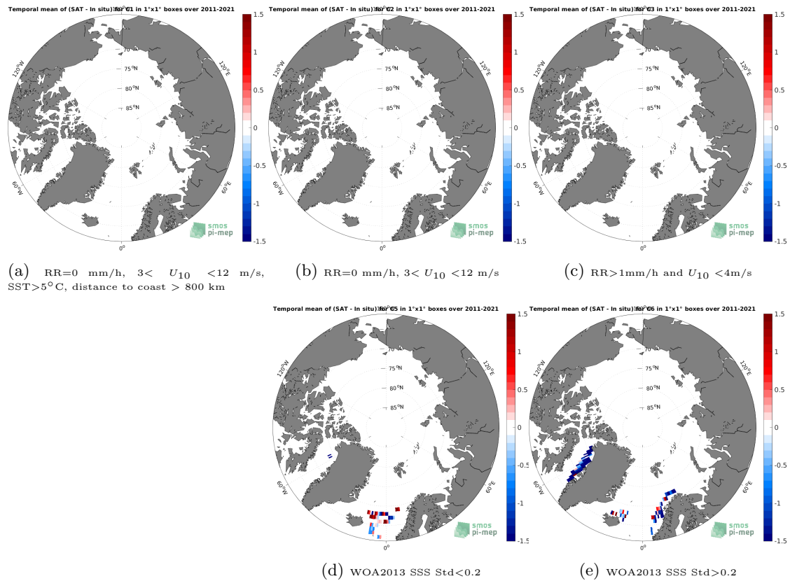
Figure 12: Temporal mean gridded over spatial boxes of size 1^{\circ}\times 1^{\circ} of \Delta\text{SSS} (SMOS SSS L2 v700 (ESA) - TSG (LEGOS-DM)) for 5 different subdatasets corresponding to:RR=0 mm/h, 3 < U_{10} < 12 m/s, SST >5^{\circ}\text{C} , distance to coast > 800 km (a), RR=0 mm/h, 3 < U_{10} < 12 m/s (b), RR >1 mm/h and U_{10} < 4 m/s (c), WOA2013 SSS Std <0.2 (d), WOA2013 SSS Std >0.2 (e).
