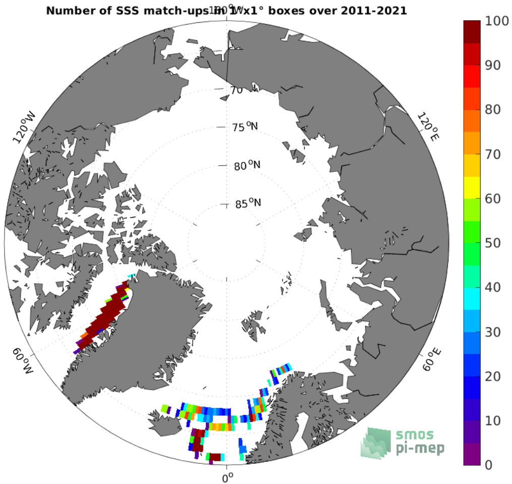
Figure 4: Number of SSS match-ups between TSG (LEGOS-DM) SSS and the SMOS SSS L2 v700 (ESA) SSS product for the Arctic Ocean Pi-MEP region over 1^\circ \times 1^\circ boxes and for the full satellite product period.
