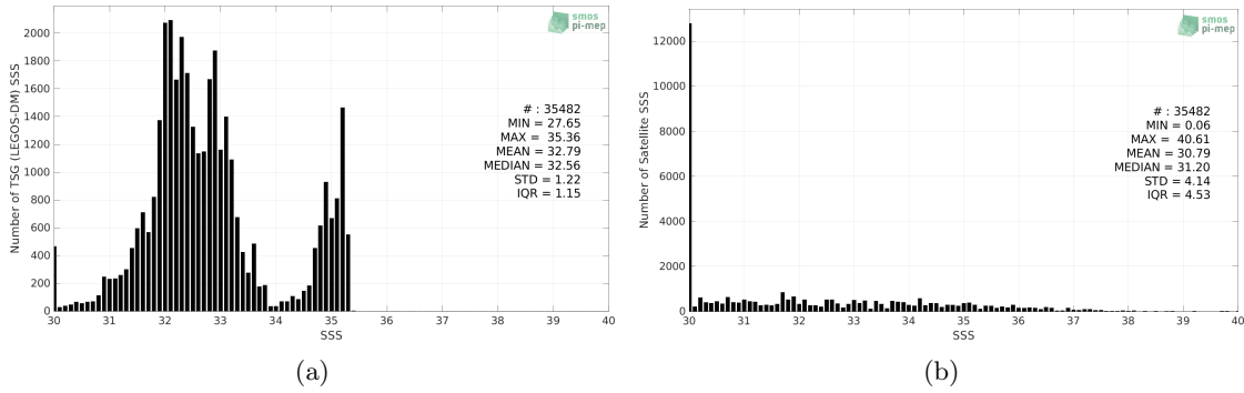
Figure 2: Histograms of SSS from TSG (LEGOS-DM) (a) and SMOS SSS L2 v700 (ESA) (b) considering all match-up pairs per bins of 0.1 over the Arctic Ocean Pi-MEP region and for the full satellite product period.
