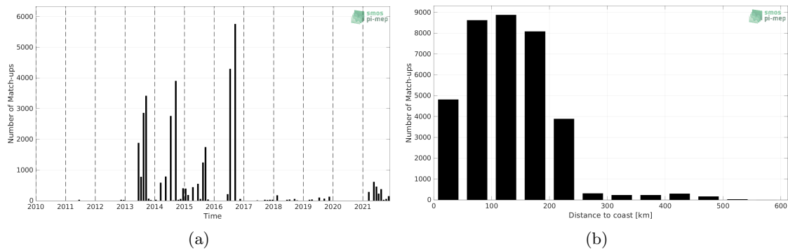
Figure 1: Number of match-ups between TSG (LEGOS-DM) and SMOS SSS L2 v700 (ESA) SSS as a function of time (a) and as function of the distance to coast (b) over the Arctic Ocean Pi-MEP region and for the full satellite product period.
