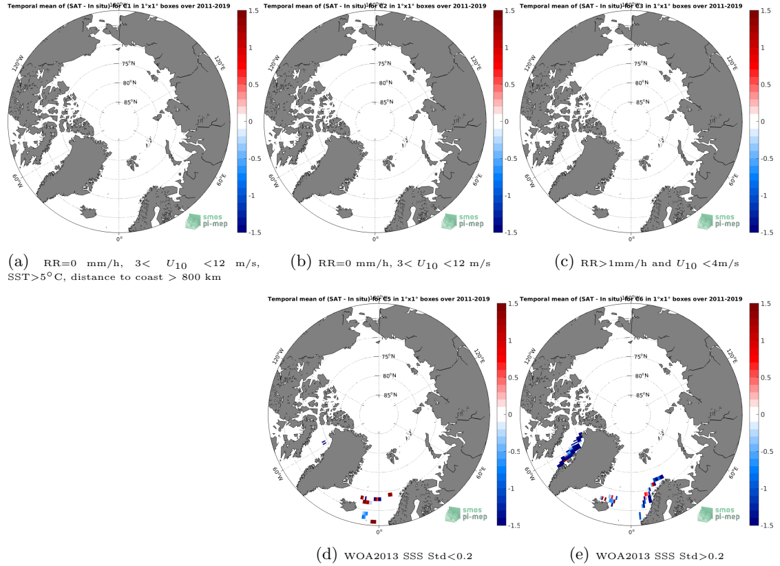
Figure 12: Temporal mean gridded over spatial boxes of size 1^{\circ}\times 1^{\circ} of \Delta\text{SSS} (SMOS SSS L2 v700 (ESA) - TSG (LEGOS-DM)) for 5 different subdatasets corresponding to: RR=0 mm/h, 3 < U_{10} < 12 m/s, SST > 5^{\circ}\text{C} , distance to coast > 800 km (a), RR=0 mm/h, 3 < U_{10} < 12 m/s (b), RR > 1 mm/h and U_{10} < 4 m/s (c), WOA2013 SSS Std < 0.2 (d), WOA2013 SSS Std > 0.2 (e).
