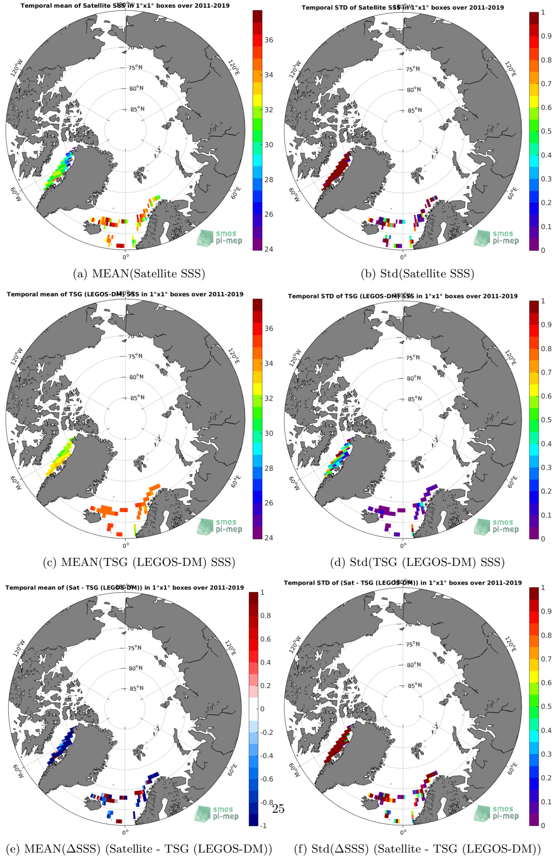
Figure 6: Temporal mean (left) and Std (right) of SSS from SMOS SSS L2 v700 (ESA) (top), TSG (LEGOS-DM) (middle), and of \Delta SSS (Satellite - TSG (LEGOS-DM)). Only match-up pairs are used to generate these maps.
