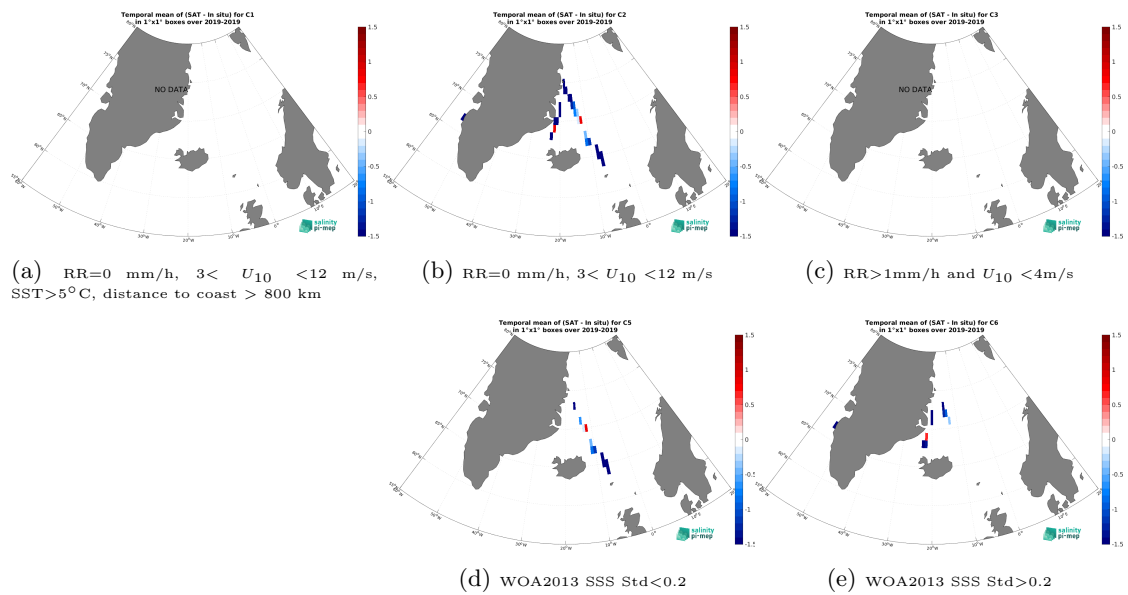
Figure 14: Temporal mean gridded over spatial boxes of size 1^\circ \times 1^\circ of \Delta SSS (SMOS SSS L2 v700 (ESA) - TSG (Lauge-Koch)) for 5 different subdatasets corresponding to: RR=0 mm/h, 3 < U_{10} < 12 m/s, SST > 5°C, distance to coast > 800 km (a), RR=0 mm/h, 3 < U_{10} < 12 m/s (b), RR > 1mm/h and U_{10} < 4 m/s (c), WOA2013 SSS Std < 0.2 (d), WOA2013 SSS Std > 0.2 (e).
