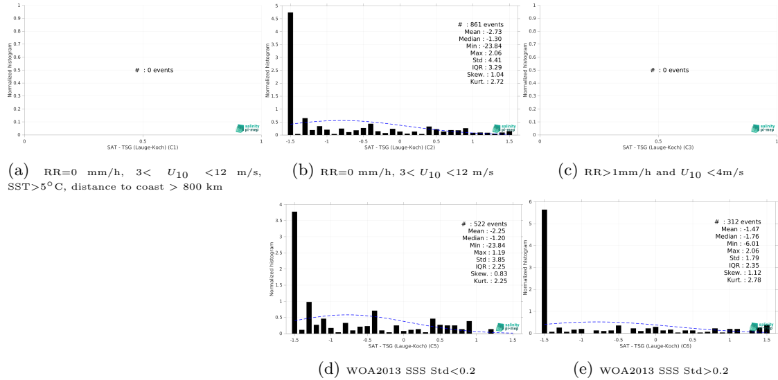
Figure 15: Normalized histogram of \Delta SSS (SMOS SSS L2 v700 (ESA) - TSG (Lauge-Koch)) for 5 different subdatasets corresponding to: RR=0 mm/h, 3 < U_{10} < 12 m/s, SST > 5°C, distance to coast > 800 km (a), RR=0 mm/h, 3 < U_{10} < 12 m/s (b), RR > 1mm/h and U_{10} < 4 m/s (c), WOA2013 SSS Std < 0.2 (d), WOA2013 SSS Std > 0.2 (e).
