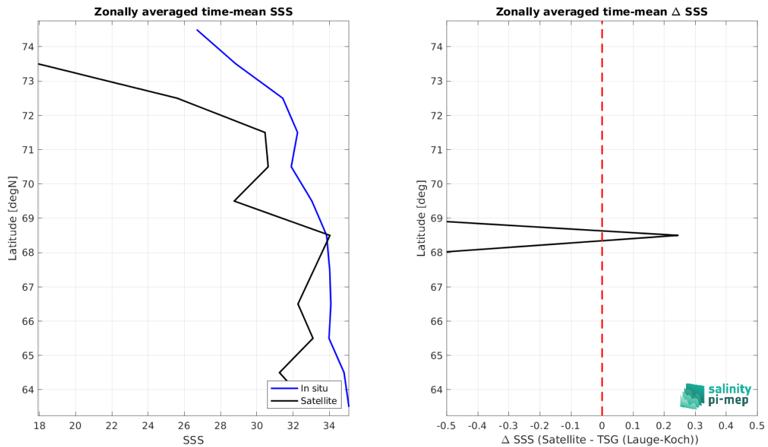
Figure 9: Left panel: Zonal mean SSS from SMOS SSS L2 v700 (ESA) satellite product (black) and from TSG (Lauge-Koch) (blue). Right panel: Zonal mean of \Delta SSS (Satellite - TSG (Lauge-Koch)) for all the collected Pi-MEP match-up pairs estimated over the full satellite product period.
