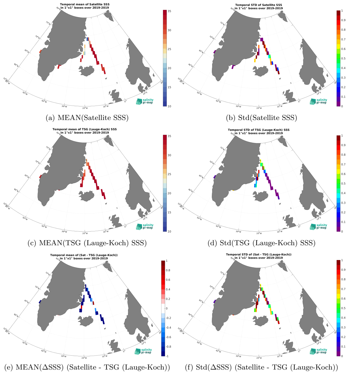
Figure 7: Temporal mean (left) and Std (right) of SSS from SMOS SSS L2 v700 (ESA) (top), TSG (Lauge-Koch) (middle), and of \Delta SSS (Satellite - TSG (Lauge-Koch)). Only match-up pairs are used to generate these maps.
