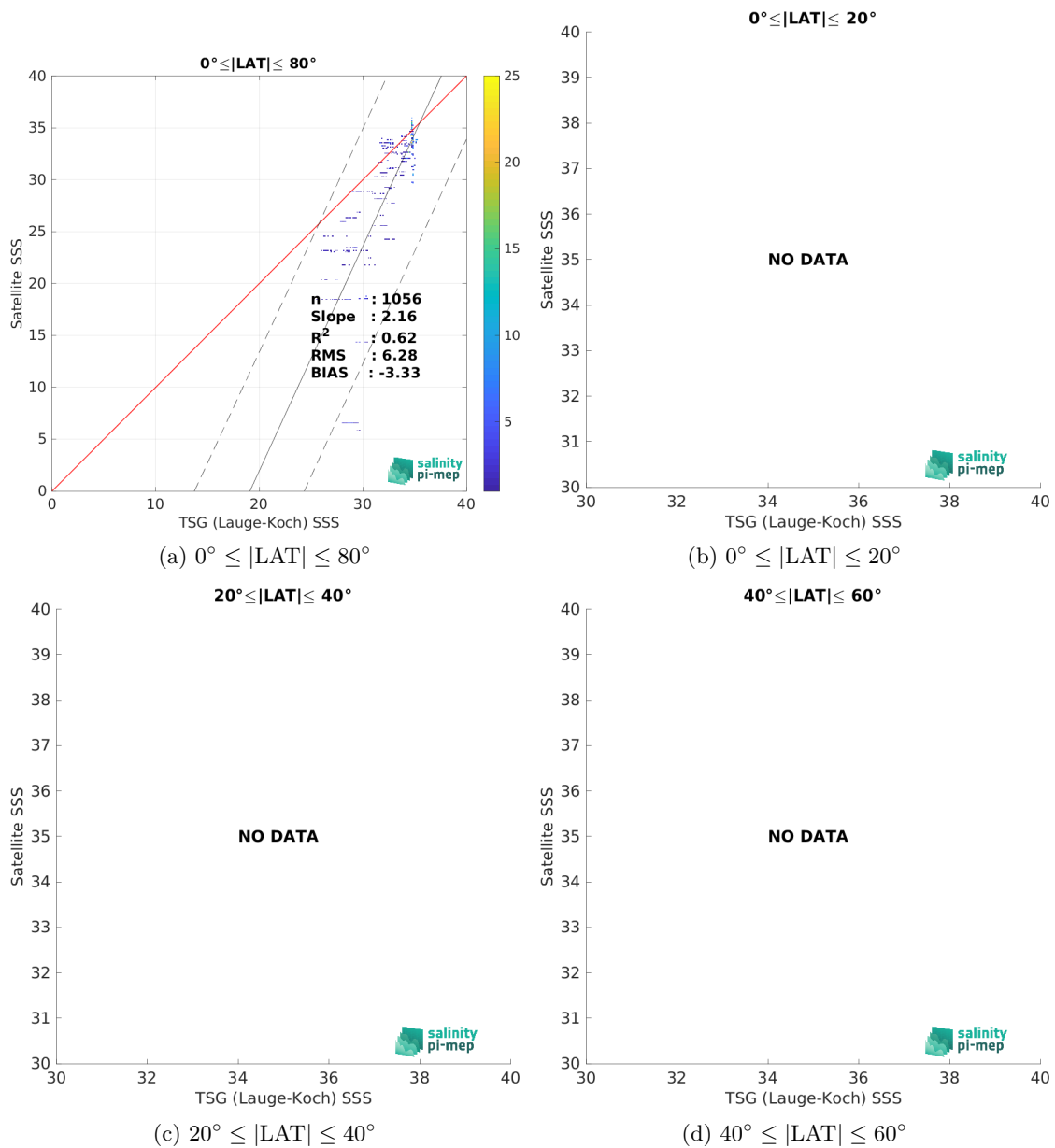
Figure 10: Contour maps of the concentration of SMOS SSS L2 v700 (ESA) SSS (y-axis) versus TSG (Laue-Koch) SSS (x-axis) at match-up pairs for different latitude bands. For each plot, the red line shows x=y . The black thin and dashed lines indicate a linear fit through the data cloud and the \pm 95\% confidence levels, respectively. The number match-up pairs n , the slope and R^2 coefficient of the linear fit, the root mean square (RMS) and the mean bias between satellite and in situ data are indicated for each latitude band in each plots.
