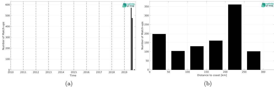
Figure 2: Number of match-ups between TSG (Lauge-Koch) and SMOS SSS L2 v700 (ESA) SSS as a function of time (a) and as function of the distance to coast (b) over the Arctic Ocean Pi-MEP region and for the full satellite product period.
