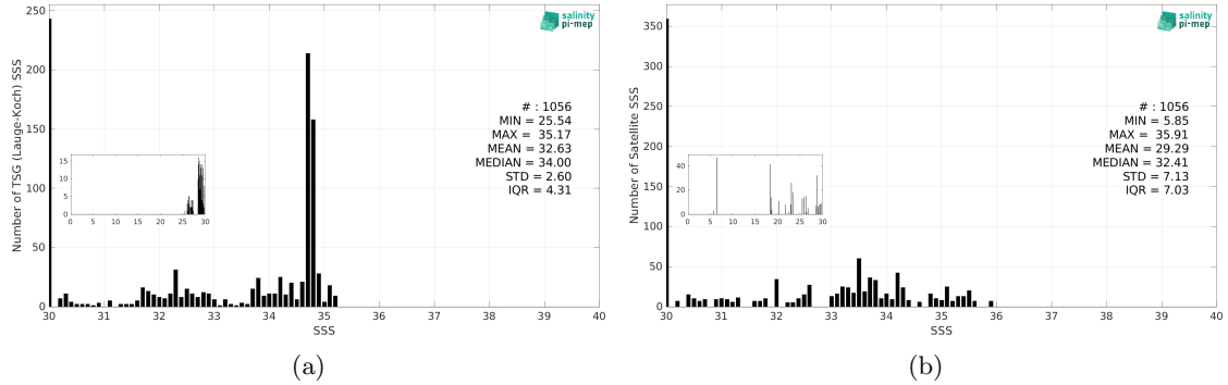
Figure 3: Histograms of SSS from TSG (Lauge-Koch) (a) and SMOS SSS L2 v700 (ESA) (b) considering all match-up pairs per bins of 0.1 over the Arctic Ocean Pi-MEP region and for the full satellite product period.
