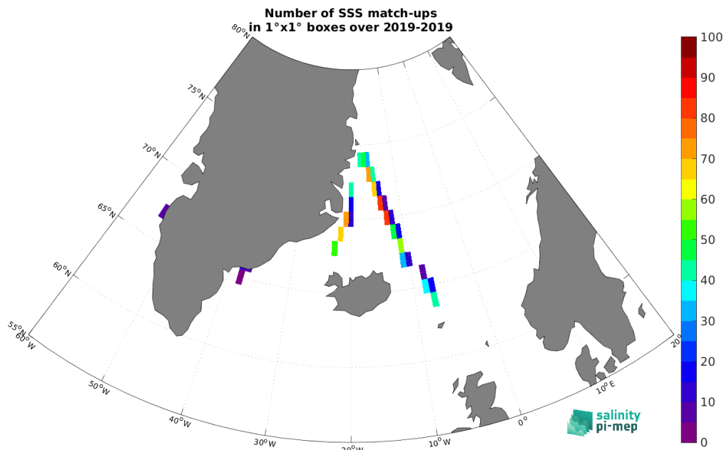
Figure 4: Number of SSS match-ups between TSG (Lauge-Koch) SSS and the SMOS SSS L2 v700 (ESA) SSS product for the Arctic Ocean Pi-MEP region over 1^\circ \times 1^\circ boxes and for the full satellite product period.
