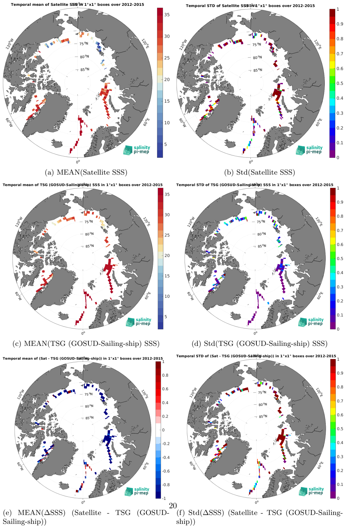
Figure 6: Temporal mean (left) and Std (right) of SSS from SMOS SSS L2 v700 (ESA) (top), TSG (GOSUD-Sailing-ship) (middle), and of \Delta SSS (Satellite - TSG (GOSUD-Sailing-ship)). Only match-up pairs are used to generate these maps.
