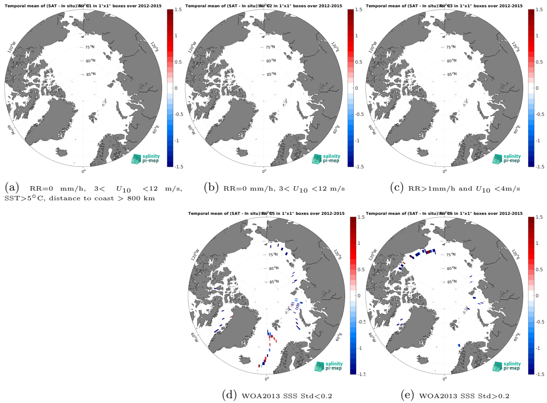
Figure 12: Temporal mean gridded over spatial boxes of size 1^\circ \times 1^\circ of \Delta SSS (SMOS SSS L2 v700 (ESA) - TSG (GOSUD-Sailing-ship)) for 5 different subdatasets corresponding to: RR=0 mm/h, 3 < U_{10} < 12 m/s, SST > 5°C, distance to coast > 800 km (a), RR=0 mm/h, 3 < U_{10} < 12 m/s (b), RR > 1mm/h and U_{10} < 4 m/s (c), WOA2013 SSS Std < 0.2 (d), WOA2013 SSS Std > 0.2 (e).
