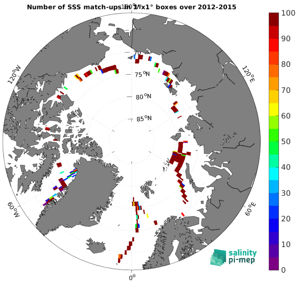
Figure 4: Number of SSS match-ups between TSG (GOSUD-Sailing-ship) SSS and the SMOS SSS L2 v700 (ESA) SSS product for the Arctic Ocean Pi-MEP region over 1^\circ \times 1^\circ boxes and for the full satellite product period.
