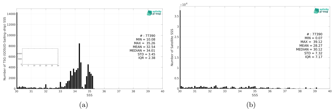
Figure 2: Histograms of SSS from TSG (GOSUD-Sailing-ship) (a) and SMOS SSS L2 v700 (ESA) (b) considering all match-up pairs per bins of 0.1 over the Arctic Ocean Pi-MEP region and for the full satellite product period.
