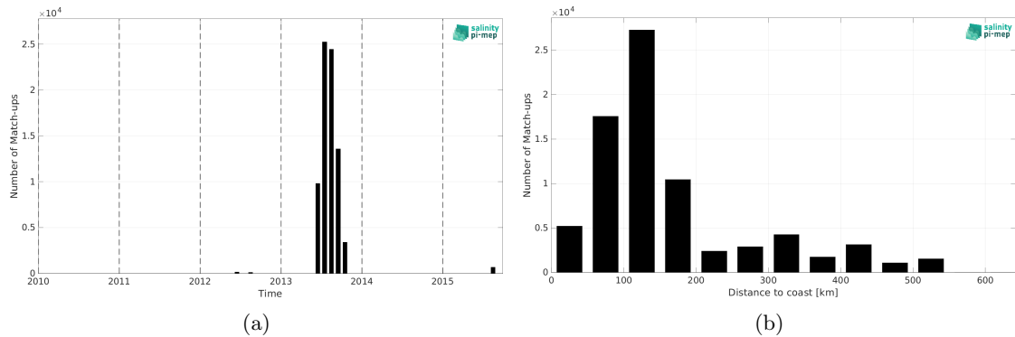
Figure 1: Number of match-ups between TSG (GOSUD-Sailing-ship) and SMOS SSS L2 v700 (ESA) SSS as a function of time (a) and as function of the distance to coast (b) over the Arctic Ocean Pi-MEP region and for the full satellite product period.
