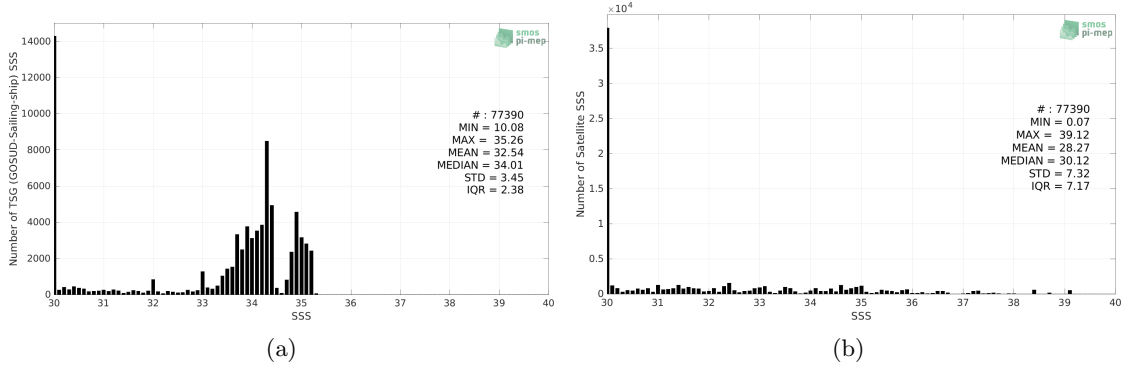
Figure 2: Histograms of SSS from TSG (GOSUD-Sailing-ship) (a) and SMOS SSS L2 v700 (ESA) (b) considering all match-up pairs per bins of 0.1 over the Arctic Ocean Pi-MEP region and for the full satellite product period.
