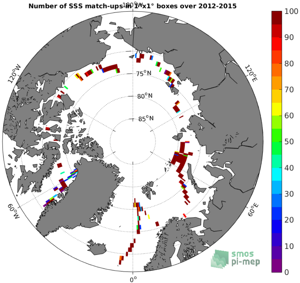
Figure 4: Number of SSS match-ups between TSG (GOSUD-Sailing-ship) SSS and the SMOS SSS L2 v700 (ESA) SSS product for the Arctic Ocean Pi-MEP region over 1°x1° boxes and for the full satellite product period.
