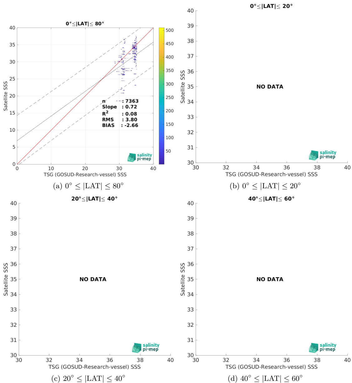
Figure 10: Contour maps of the concentration of SMOS SSS L2 v700 (ESA) SSS (y-axis) versus TSG (GOSUD-Research-vessel) SSS (x-axis) at match-up pairs for different latitude bands. For each plot, the red line shows x=y . The black thin and dashed lines indicate a linear fit through the data cloud and the \pm 95\% confidence levels, respectively. The number match-up pairs n , the slope and R^2 coefficient of the linear fit, the root mean square (RMS) and the mean bias between satellite and in situ data are indicated for each latitude band in each plots.
