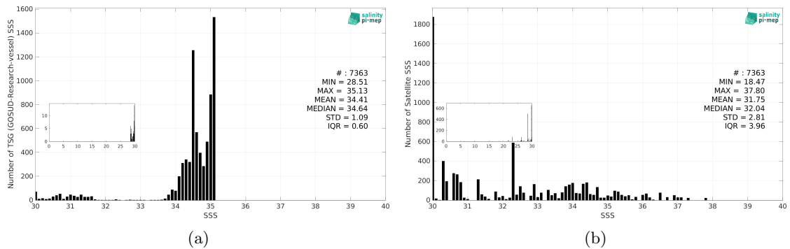
Figure 3: Histograms of SSS from TSG (GOSUD-Research-vessel) (a) and SMOS SSS L2 v700 (ESA) (b) considering all match-up pairs per bins of 0.1 over the Arctic Ocean Pi-MEP region and for the full satellite product period.
