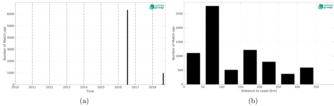
Figure 2: Number of match-ups between TSG (GOSUD-Research-vessel) and SMOS SSS L2 v700 (ESA) SSS as a function of time (a) and as function of the distance to coast (b) over the Arctic Ocean Pi-MEP region and for the full satellite product period.
