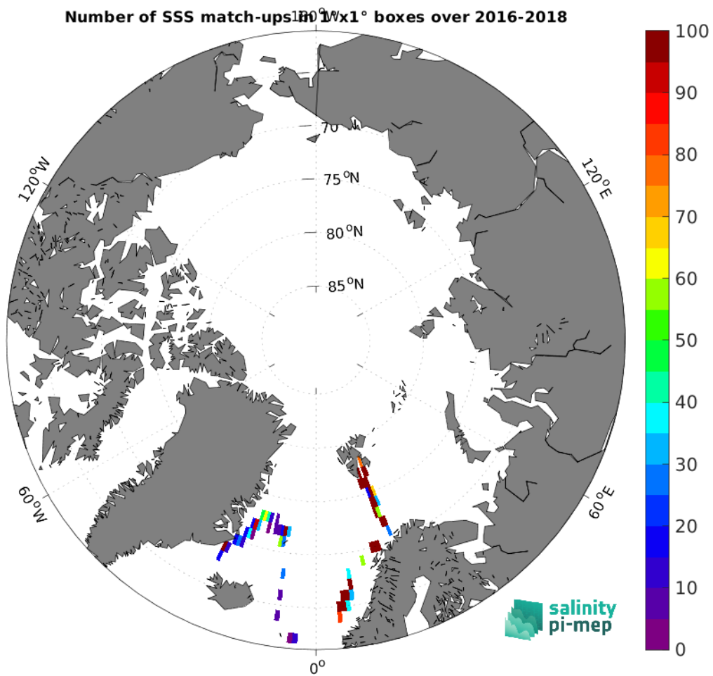
Figure 5: Number of SSS match-ups between TSG (GOSUD-Research-vessel) SSS and the SMOS SSS L2 v700 (ESA) SSS product for the Arctic Ocean Pi-MEP region over 1^\circ \times 1^\circ boxes and for the full satellite product period.
