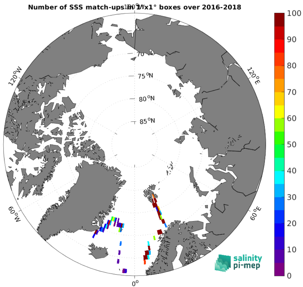
Figure 4: Number of SSS match-ups between TSG (GOSUD-Research-vessel) SSS and the SMOS SSS L2 v700 (ESA) SSS product for the Arctic Ocean Pi-MEP region over 1^\circ \times 1^\circ boxes and for the full satellite product period.
