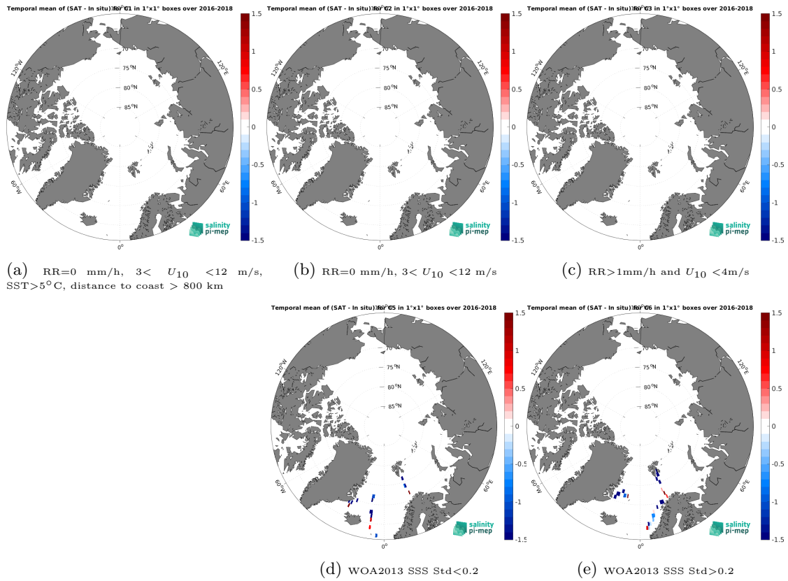
Figure 12: Temporal mean gridded over spatial boxes of size 1^\circ \times 1^\circ of \Delta SSS (SMOS SSS L2 v700 (ESA) - TSG (GOSUD-Research-vessel)) for 5 different subdatasets corresponding to:RR=0 mm/h, 3 < U_{10} < 12 m/s, SST>5°C, distance to coast > 800 km (a), RR=0 mm/h, 3 < U_{10} < 12 m/s (b), RR>1mm/h and U_{10} < 4 m/s (c), WOA2013 SSS Std<0.2 (d), WOA2013 SSS Std>0.2 (e).
