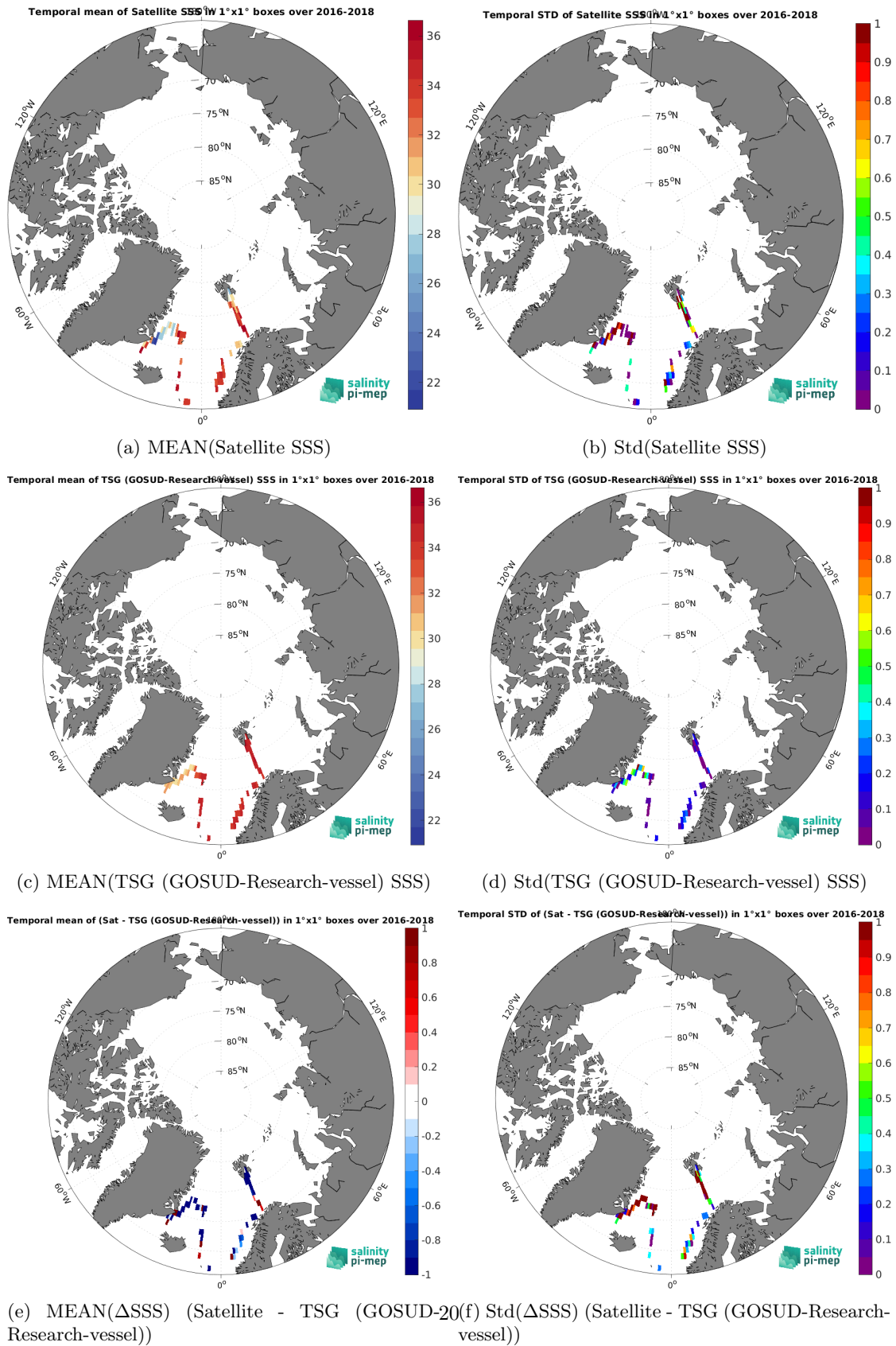
Figure 6: Temporal mean (left) and Std (right) of SSS from SMOS SSS L2 v700 (ESA) (top), TSG (GOSUD-Research-vessel) (middle), and of \Delta SSS (Satellite - TSG (GOSUD-Research-vessel)). Only match-up pairs are used to generate these maps.
