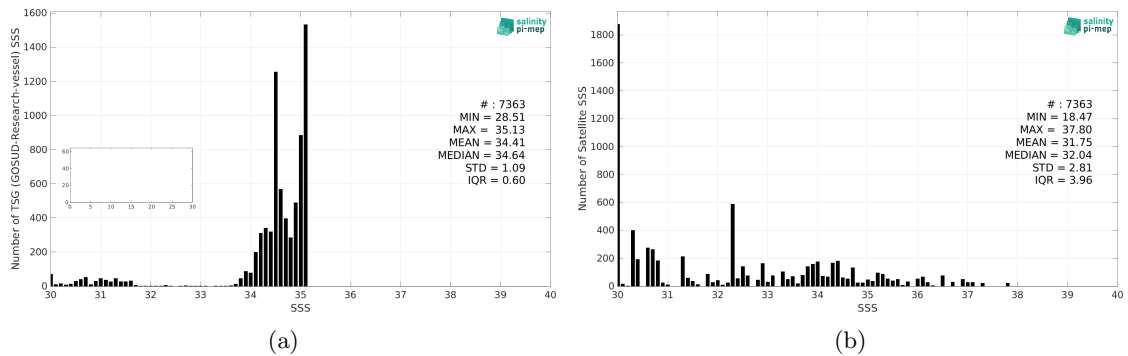
Figure 2: Histograms of SSS from TSG (GOSUD-Research-vessel) (a) and SMOS SSS L2 v700 (ESA) (b) considering all match-up pairs per bins of 0.1 over the Arctic Ocean Pi-MEP region and for the full satellite product period.
