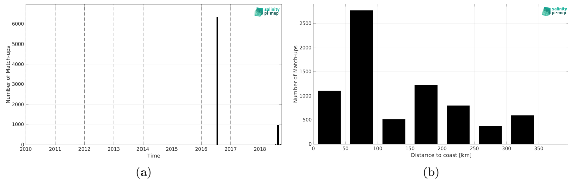
Figure 1: Number of match-ups between TSG (GOSUD-Research-vessel) and SMOS SSS L2 v700 (ESA) SSS as a function of time (a) and as function of the distance to coast (b) over the Arctic Ocean Pi-MEP region and for the full satellite product period.
