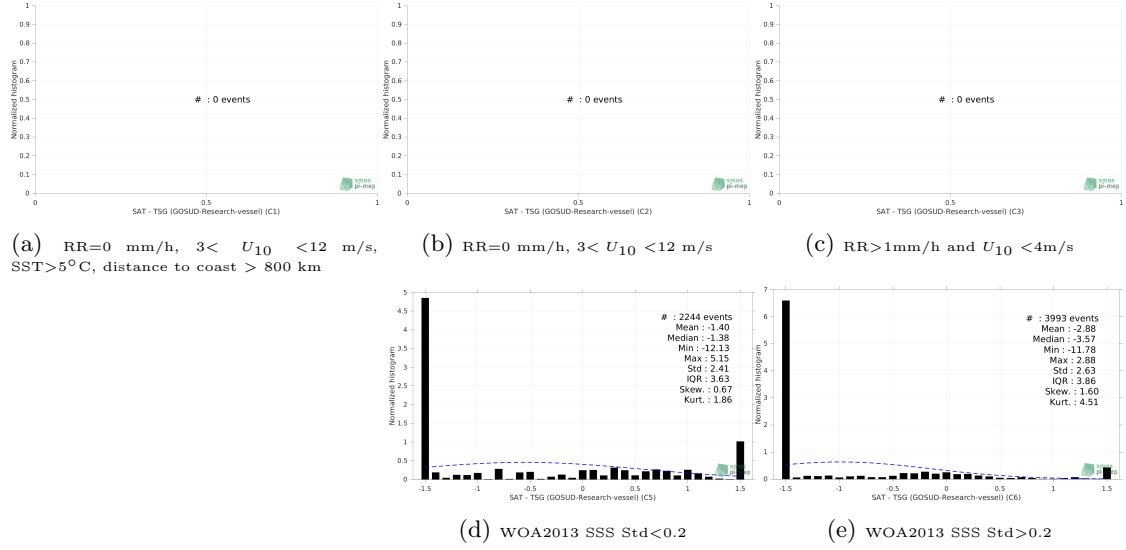
Figure 13: Normalized histogram of \Delta\text{SSS} (SMOS SSS L2 v700 (ESA) - TSG (GOSUD-Research-vessel)) for 5 different subdatasets corresponding to: RR=0 mm/h, 3 < U_{10} < 12 m/s, SST > 5^\circ\text{C} , distance to coast > 800 km (a), RR=0 mm/h, 3 < U_{10} < 12 m/s (b), RR > 1\text{mm/h} and U_{10} < 4\text{m/s} (c), WOA2013 SSS Std < 0.2 (d), WOA2013 SSS Std > 0.2 (e).
