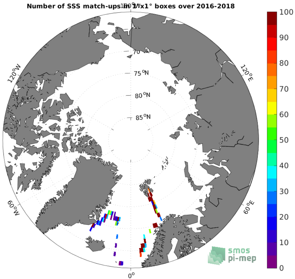
Figure 4: Number of SSS match-ups between TSG (GOSUD-Research-vessel) SSS and the SMOS SSS L2 v700 (ESA) SSS product for the Arctic Ocean Pi-MEP region over 1^{\circ} \times 1^{\circ} boxes and for the full satellite product period.
