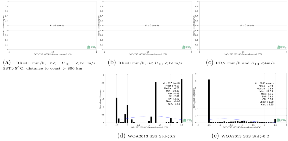
Figure 13: Normalized histogram of \Delta\text{SSS} (SMOS SSS L2 v700 (ESA) - TSG (GOSUD-Research-vessel)) for 5 different subdatasets corresponding to: RR=0 mm/h, 3 < U_{10} < 12 m/s, SST > 5^{\circ}\text{C} , distance to coast > 800 km (a), RR=0 mm/h, 3 < U_{10} < 12 m/s (b), RR > 1\text{mm/h} and U_{10} < 4\text{m/s} (c), WOA2013 SSS Std < 0.2 (d), WOA2013 SSS Std > 0.2 (e).
