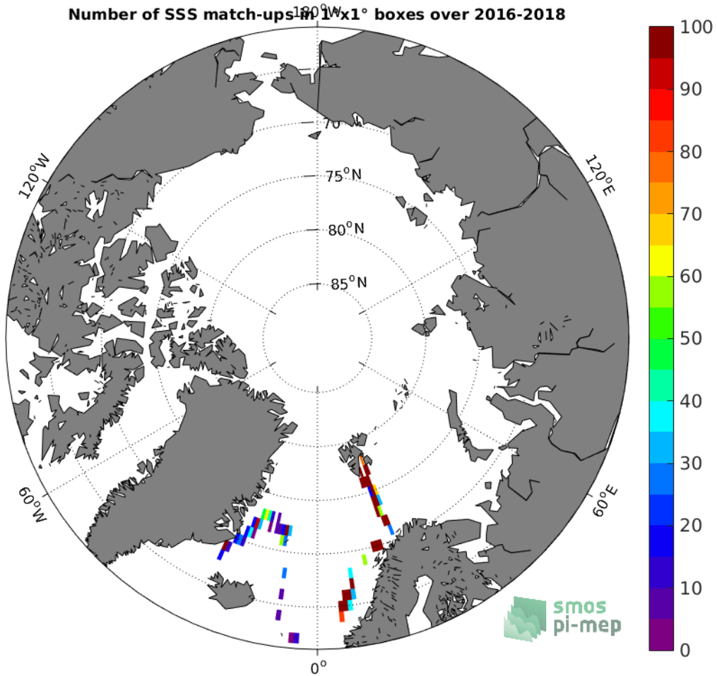
Figure 4: Number of SSS match-ups between TSG (GOSUD-Research-vessel) SSS and the SMOS SSS L2 v700 (ESA) SSS product for the Arctic Ocean Pi-MEP region over 1°x1° boxes and for the full satellite product period.
