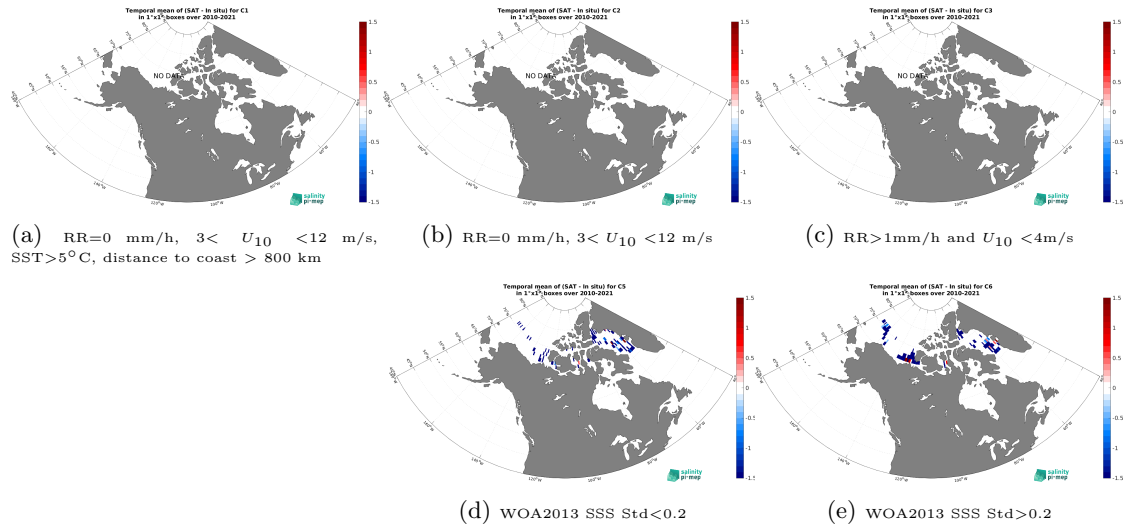
Figure 12: Temporal mean gridded over spatial boxes of size 1^{\circ}\times 1^{\circ} of \Delta\text{SSS} (SMOS SSS L2 v700 (ESA) - TSG (Amundsen)) for 5 different subdatasets corresponding to:RR=0 mm/h, 3 < U_{10} < 12 m/s, SST >5^{\circ}\text{C} , distance to coast > 800 km (a), RR=0 mm/h, 3 < U_{10} < 12 m/s (b), RR >1 mm/h and U_{10} < 4 m/s (c), WOA2013 SSS Std <0.2 (d), WOA2013 SSS Std >0.2 (e).
