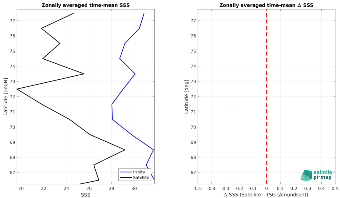
Figure 8: Left panel: Zonal mean SSS from SMOS SSS L2 v700 (ESA) satellite product (black) and from TSG (Amundsen) (blue). Right panel: Zonal mean of \Delta SSS (Satellite - TSG (Amundsen)) for all the collected Pi-MEP match-up pairs estimated over the full satellite product period.
