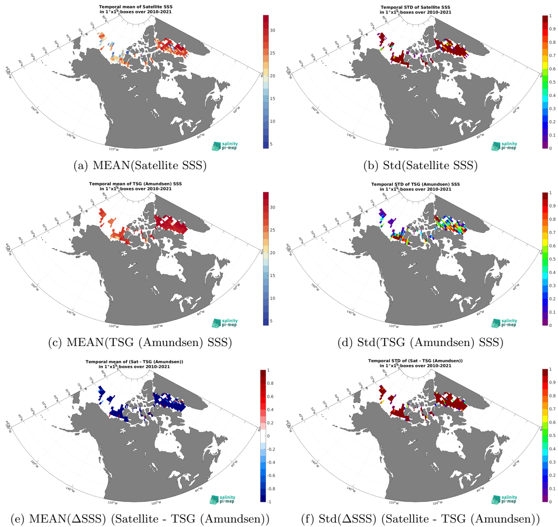
Figure 6: Temporal mean (left) and Std (right) of SSS from SMOS SSS L2 v700 (ESA) (top), TSG (Amundsen) (middle), and of \Delta SSS (Satellite - TSG (Amundsen)). Only match-up pairs are used to generate these maps.
