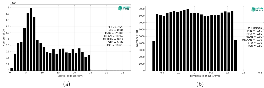
Figure 5: Histograms of the spatial (a) and temporal (b) lags between the location/time of the TSG (Amundsen) measurement and the date of the corresponding SMOS SSS L2 v700 (ESA) SSS pixel.
