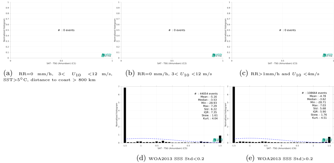
Figure 13: Normalized histogram of \Delta SSS (SMOS SSS L2 v700 (ESA) - TSG (Amundsen)) for 5 different subdatasets corresponding to: RR=0 mm/h, 3 < U_{10} < 12 m/s, SST > 5°C, distance to coast > 800 km (a), RR=0 mm/h, 3 < U_{10} < 12 m/s (b), RR > 1mm/h and U_{10} < 4 m/s (c), WOA2013 SSS Std < 0.2 (d), WOA2013 SSS Std > 0.2 (e).
