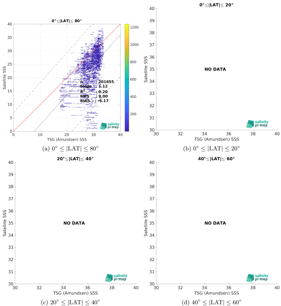
Figure 9: Contour maps of the concentration of SMOS SSS L2 v700 (ESA) SSS (y-axis) versus TSG (Amundsen) SSS (x-axis) at match-up pairs for different latitude bands. For each plot, the red line shows x=y . The black thin and dashed lines indicate a linear fit through the data cloud and the \pm 95\% confidence levels, respectively. The number match-up pairs n , the slope and R^2 coefficient of the linear fit, the root mean square (RMS) and the mean bias between satellite and in situ data are indicated for each latitude band in each plots.
