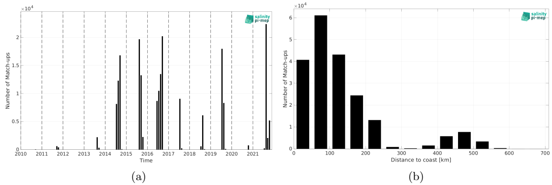
Figure 1: Number of match-ups between TSG (Amundsen) and SMOS SSS L2 v700 (ESA) SSS as a function of time (a) and as function of the distance to coast (b) over the Arctic Ocean Pi-MEP region and for the full satellite product period.
