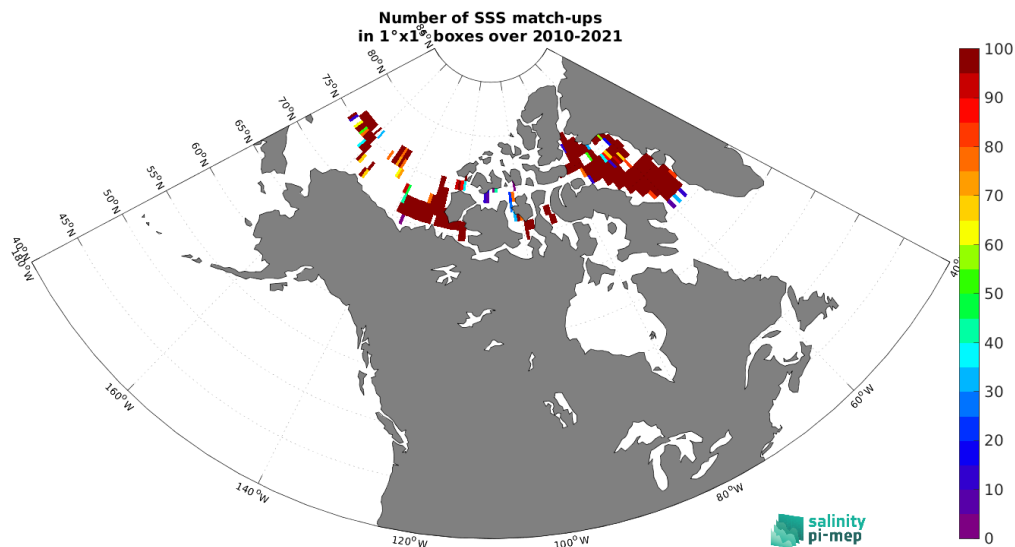
Figure 4: Number of SSS match-ups between TSG (Amundsen) SSS and the SMOS SSS L2 v700 (ESA) SSS product for the Arctic Ocean Pi-MEP region over 1^\circ \times 1^\circ boxes and for the full satellite product period.
