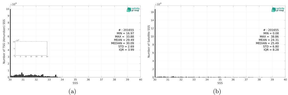
Figure 2: Histograms of SSS from TSG (Amundsen) (a) and SMOS SSS L2 v700 (ESA) (b) considering all match-up pairs per bins of 0.1 over the Arctic Ocean Pi-MEP region and for the full satellite product period.
