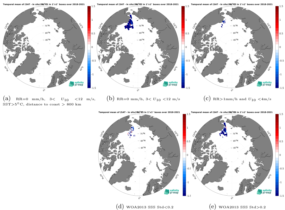
Figure 14: Temporal mean gridded over spatial boxes of size 1^\circ \times 1^\circ of \Delta\text{SSS} (SMOS SSS L2 v700 (ESA) - Sailability) for 5 different subdatasets corresponding to: RR=0 mm/h, 3 < U_{10} < 12 m/s, SST > 5°C, distance to coast > 800 km (a), RR=0 mm/h, 3 < U_{10} < 12 m/s (b), RR > 1mm/h and U_{10} < 4 m/s (c), WOA2013 SSS Std < 0.2 (d), WOA2013 SSS Std > 0.2 (e).
