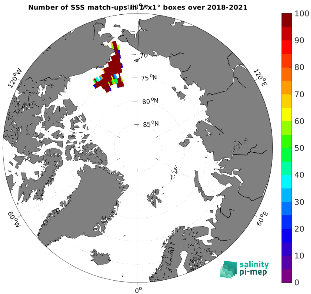
Figure 4: Number of SSS match-ups between Saildrone SSS and the SMOS SSS L2 v700 (ESA) SSS product for the Arctic Ocean Pi-MEP region over 1^\circ \times 1^\circ boxes and for the full satellite product period.
