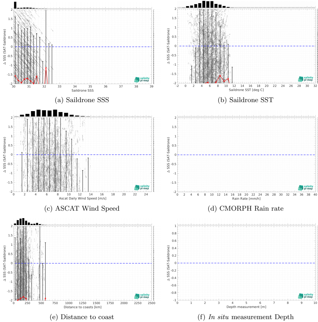
Figure 11: \Delta SSS (Satellite - Sailldrone) sorted as function of Sailldrone SSS values a), Sailldrone SST b), ASCAT Wind speed c), CMORPH rain rate d), distance to coast (e) and in situ measurement depth (f). In all plots the median and Std of \Delta SSS for each bin is indicated by the red curves and black vertical thick bars ( \pm 1 Std)
