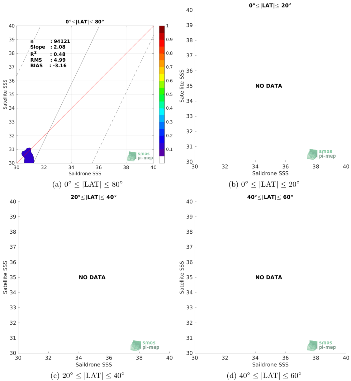
Figure 9: Contour maps of the concentration of SMOS SSS L2 v700 (ESA) SSS (y-axis) versus Sailldrone SSS (x-axis) at match-up pairs for different latitude bands. For each plot, the red line shows x=y . The black thin and dashed lines indicate a linear fit through the data cloud and the \pm 95\% confidence levels, respectively. The number match-up pairs n , the slope and R^2 coefficient of the linear fit, the root mean square (RMS) and the mean bias between satellite and in situ data are indicated for each latitude band in each plots.
