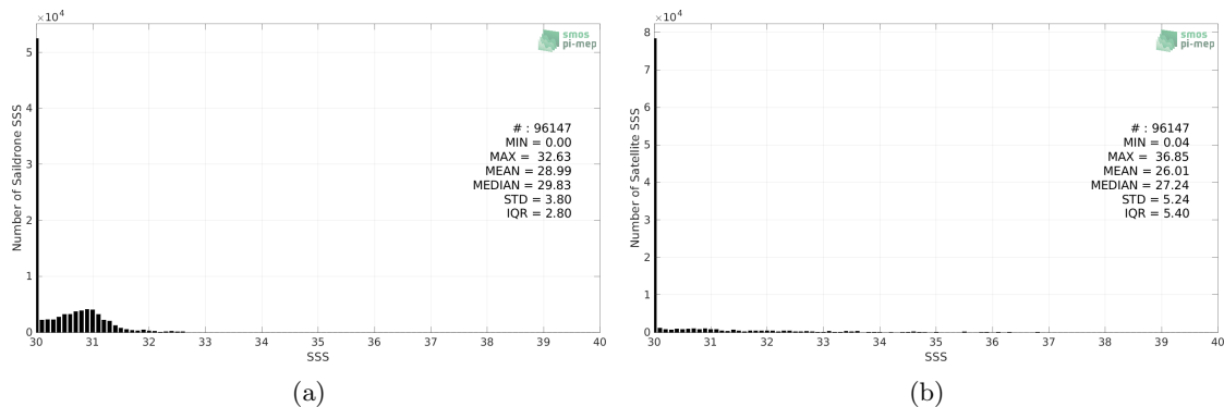
Figure 2: Histograms of SSS from Sairdrone (a) and SMOS SSS L2 v700 (ESA) (b) considering all match-up pairs per bins of 0.1 over the Arctic Ocean Pi-MEP region and for the full satellite product period.
