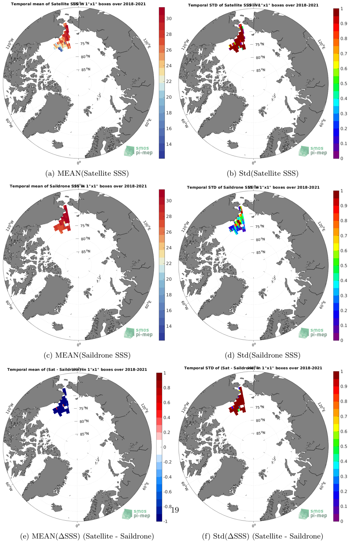
Figure 6: Temporal mean (left) and Std (right) of SSS from SMOS SSS L2 v700 (ESA) (top), Saildrone (middle), and of \Delta SSS (Satellite - Saildrone). Only match-up pairs are used to generate these maps.
