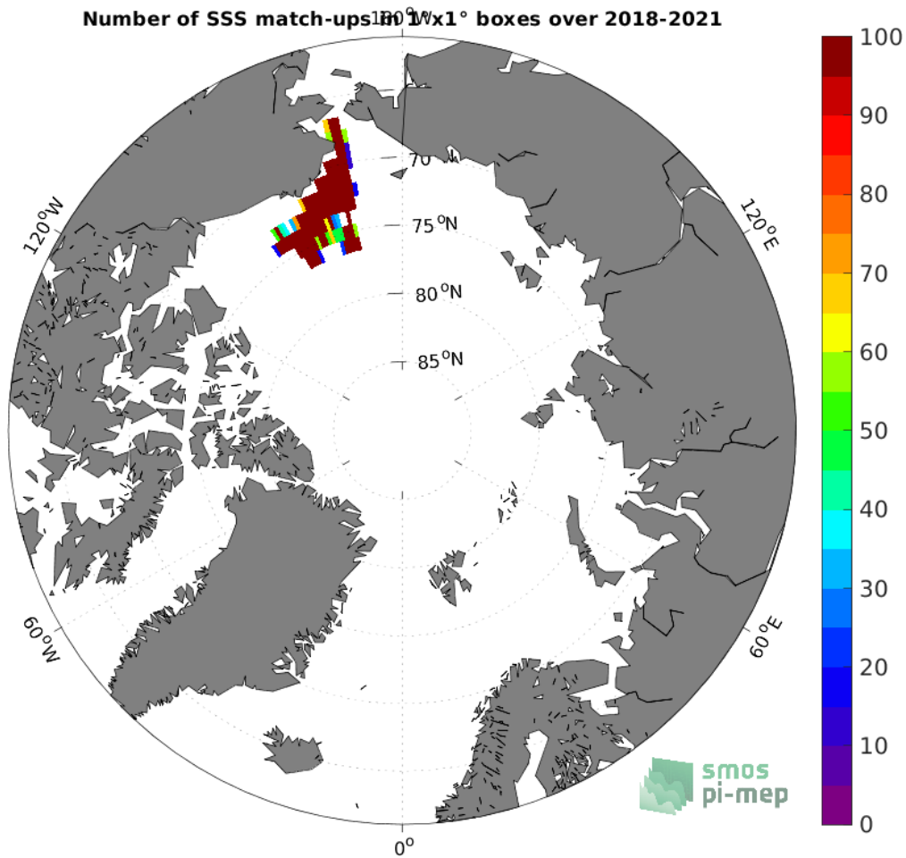
Figure 4: Number of SSS match-ups between Saildrone SSS and the SMOS SSS L2 v700 (ESA) SSS product for the Arctic Ocean Pi-MEP region over 1^{\circ} \times 1^{\circ} boxes and for the full satellite product period.
