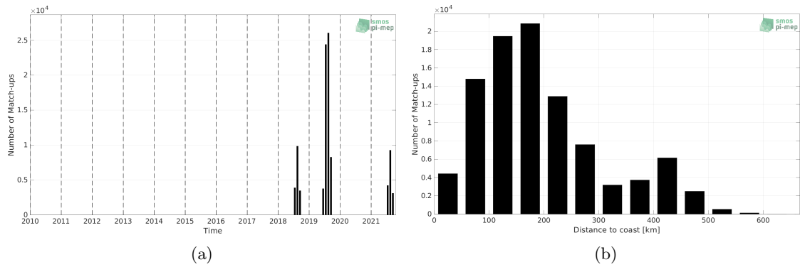
Figure 1: Number of match-ups between Sairdrone and SMOS SSS L2 v700 (ESA) SSS as a function of time (a) and as function of the distance to coast (b) over the Arctic Ocean Pi-MEP region and for the full satellite product period.
