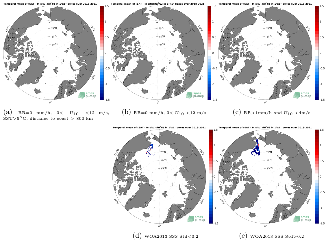
Figure 12: Temporal mean gridded over spatial boxes of size 1^{\circ}\times 1^{\circ} of \Delta\text{SSS} (SMOS SSS L2 v700 (ESA) - Sairdrone) for 5 different subdatasets corresponding to:RR=0 mm/h, 3 < U_{10} < 12 m/s, SST >5^{\circ}\text{C} , distance to coast > 800 km (a), RR=0 mm/h, 3 < U_{10} < 12 m/s (b), RR >1 mm/h and U_{10} < 4 m/s (c), WOA2013 SSS Std <0.2 (d), WOA2013 SSS Std >0.2 (e).
