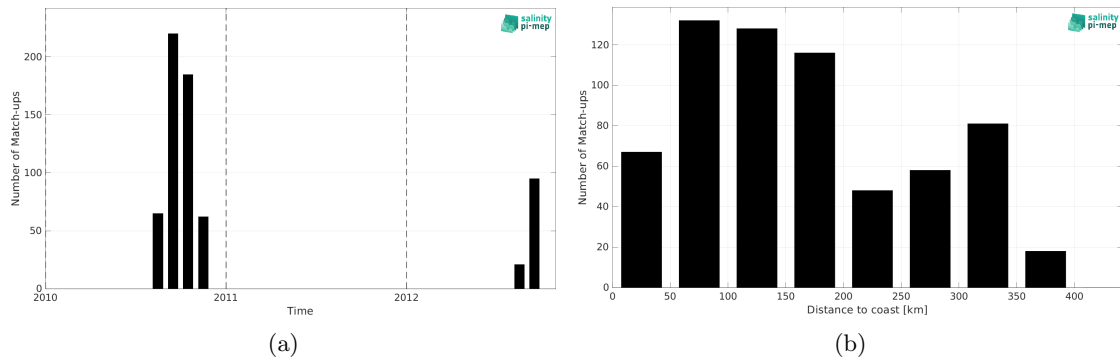
Figure 2: Number of match-ups between Marine mammals and SMOS SSS L2 v700 (ESA) SSS as a function of time (a) and as function of the distance to coast (b) over the Arctic Ocean Pi-MEP region and for the full satellite product period.
