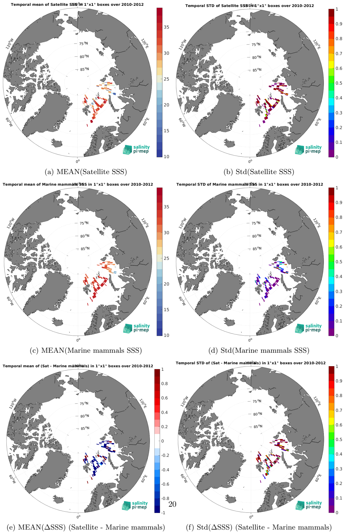
Figure 7: Temporal mean (left) and Std (right) of SSS from SMOS SSS L2 v700 (ESA) (top), Marine mammals (middle), and of \Delta SSS (Satellite - Marine mammals). Only match-up pairs are used to generate these maps.
