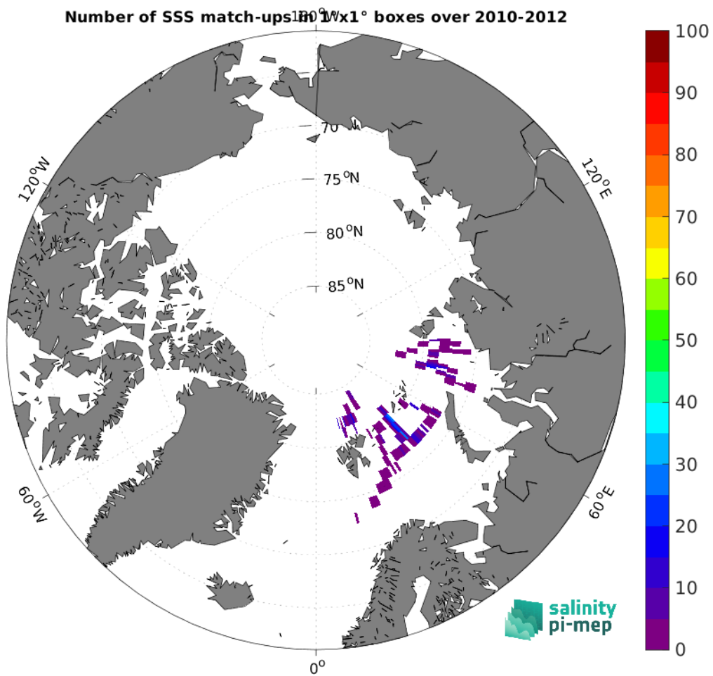
Figure 5: Number of SSS match-ups between Marine mammals SSS and the SMOS SSS L2 v700 (ESA) SSS product for the Arctic Ocean Pi-MEP region over 1^\circ \times 1^\circ boxes and for the full satellite product period.
