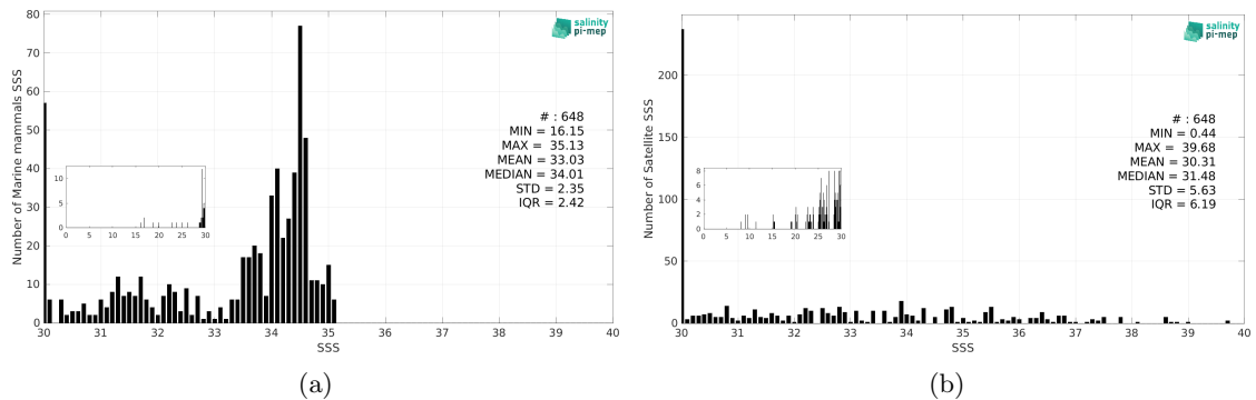
Figure 3: Histograms of SSS from Marine mammals (a) and SMOS SSS L2 v700 (ESA) (b) considering all match-up pairs per bins of 0.1 over the Arctic Ocean Pi-MEP region and for the full satellite product period.
