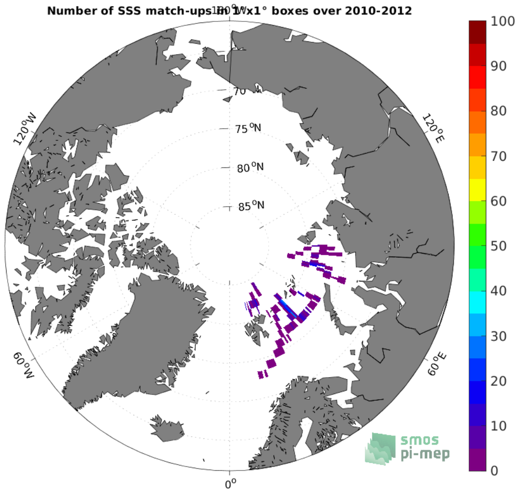
Figure 4: Number of SSS match-ups between Marine mammals SSS and the SMOS SSS L2 v700 (ESA) SSS product for the Arctic Ocean Pi-MEP region over 1^{\circ} \times 1^{\circ} boxes and for the full satellite product period.
