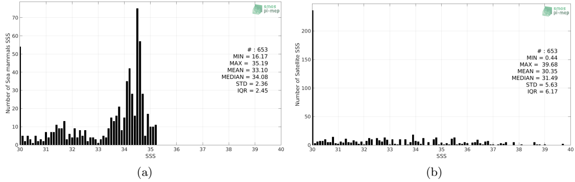
Figure 2: Histograms of SSS from Sea mammals (a) and SMOS SSS L2 v700 (ESA) (b) considering all match-up pairs per bins of 0.1 over the Arctic Ocean Pi-MEP region and for the full satellite product period.
