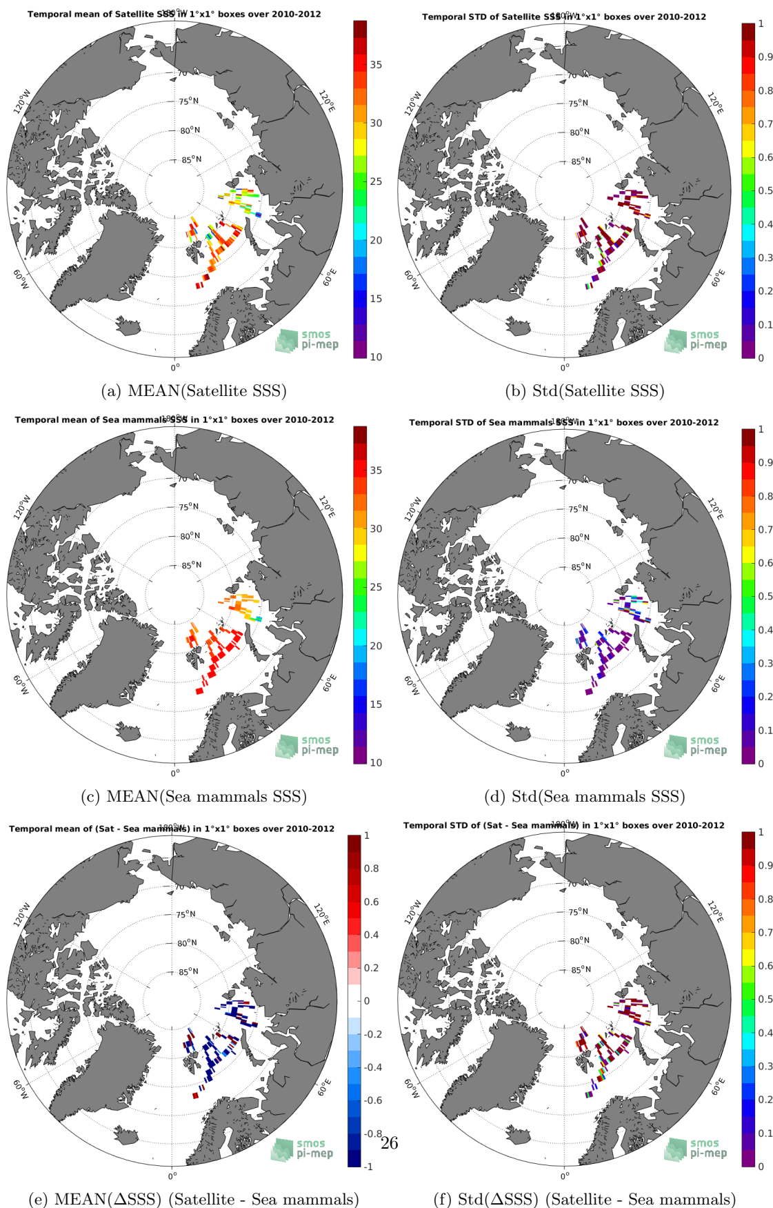
Figure 6: Temporal mean (left) and Std (right) of SSS from SMOS SSS L2 v700 (ESA) (top), Sea mammals (middle), and of \Delta SSS (Satellite - Sea mammals). Only match-up pairs are used to generate these maps.
