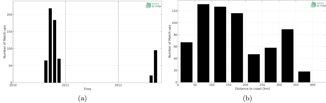
Figure 1: Number of match-ups between Sea mammals and SMOS SSS L2 v700 (ESA) SSS as a function of time (a) and as function of the distance to coast (b) over the Arctic Ocean Pi-MEP region and for the full satellite product period.
