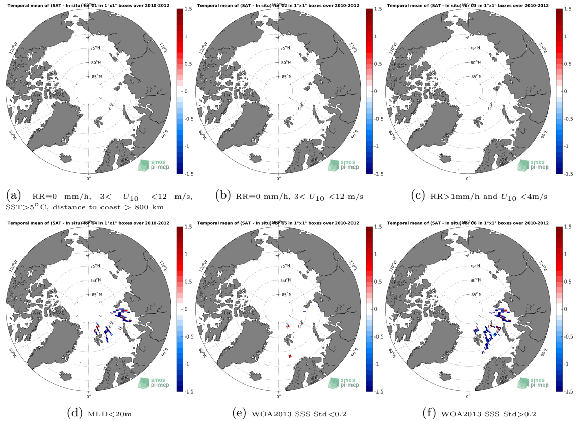
Figure 12: Temporal mean gridded over spatial boxes of size 1^{\circ}\times 1^{\circ} of \Delta\text{SSS} (SMOS SSS L2 v700 (ESA) - Sea mammals) for 6 different subdatasets corresponding to: RR=0 mm/h, 3 < U_{10} < 12 m/s, SST > 5^{\circ}\text{C} , distance to coast > 800 km (a), RR=0 mm/h, 3 < U_{10} < 12 m/s (b), RR > 1 mm/h and U_{10} < 4 m/s (c), MLD < 20\text{m} (d), WOA2013 SSS Std < 0.2 (e), WOA2013 SSS Std > 0.2 (f).
