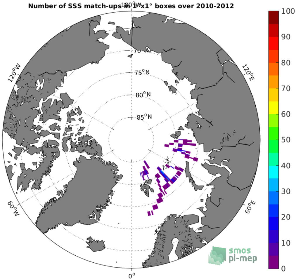
Figure 4: Number of SSS match-ups between Sea mammals SSS and the SMOS SSS L2 v700 (ESA) SSS product for the Arctic Ocean Pi-MEP region over 1°x1° boxes and for the full satellite product period.
