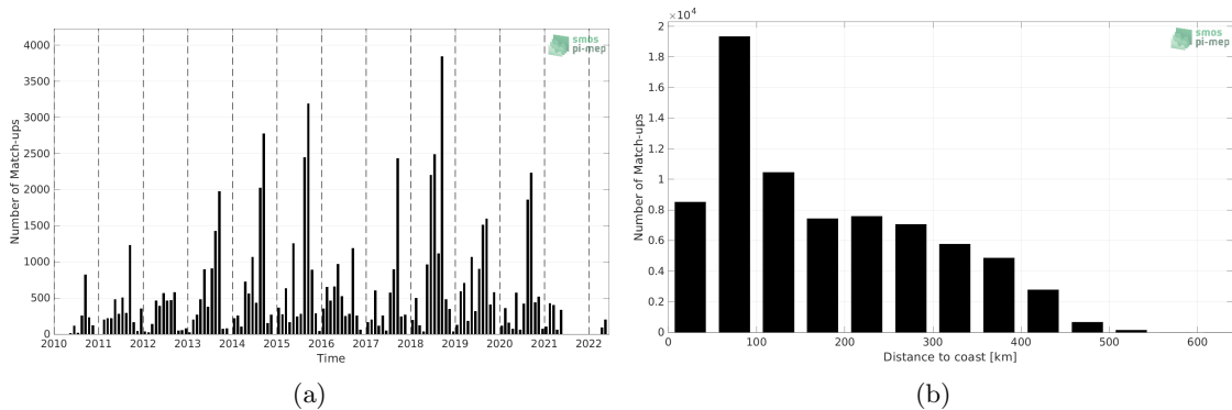
Figure 1: Number of match-ups between ICES and SMOS SSS L2 v700 (ESA) SSS as a function of time (a) and as function of the distance to coast (b) over the Arctic Ocean Pi-MEP region and for the full satellite product period.
