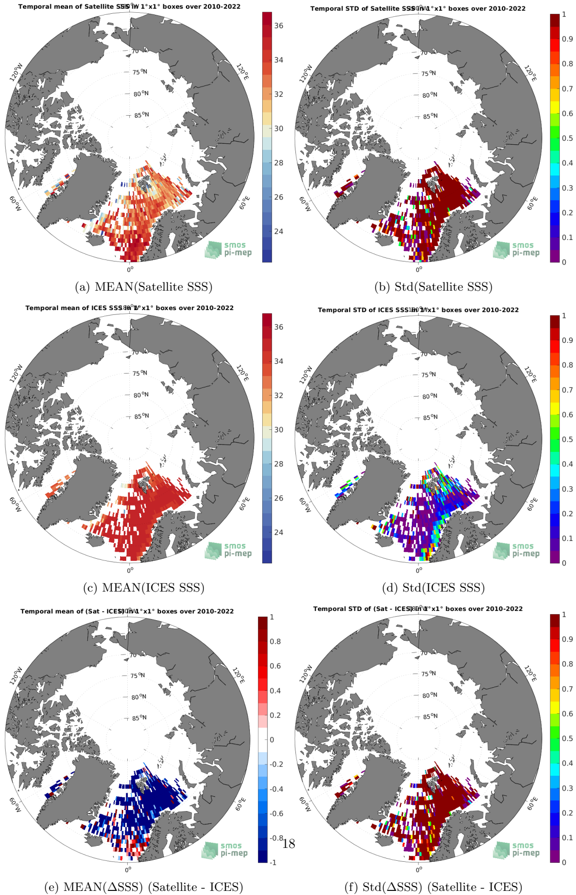
Figure 6: Temporal mean (left) and Std (right) of SSS from SMOS SSS L2 v700 (ESA) (top), ICES (middle), and of \Delta SSS (Satellite - ICES). Only match-up pairs are used to generate these maps.
