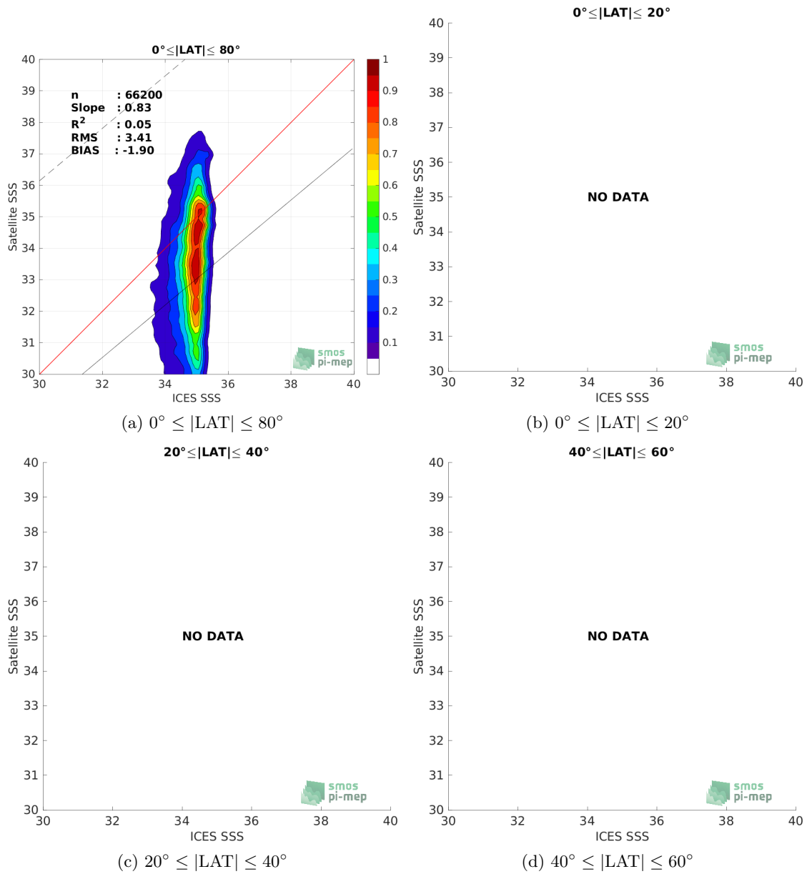
Figure 9: Contour maps of the concentration of SMOS SSS L2 v700 (ESA) SSS (y-axis) versus ICES SSS (x-axis) at match-up pairs for different latitude bands. For each plot, the red line shows x=y . The black thin and dashed lines indicate a linear fit through the data cloud and the \pm 95\% confidence levels, respectively. The number match-up pairs n , the slope and R^2 coefficient of the linear fit, the root mean square (RMS) and the mean bias between satellite and in situ data are indicated for each latitude band in each plots.
