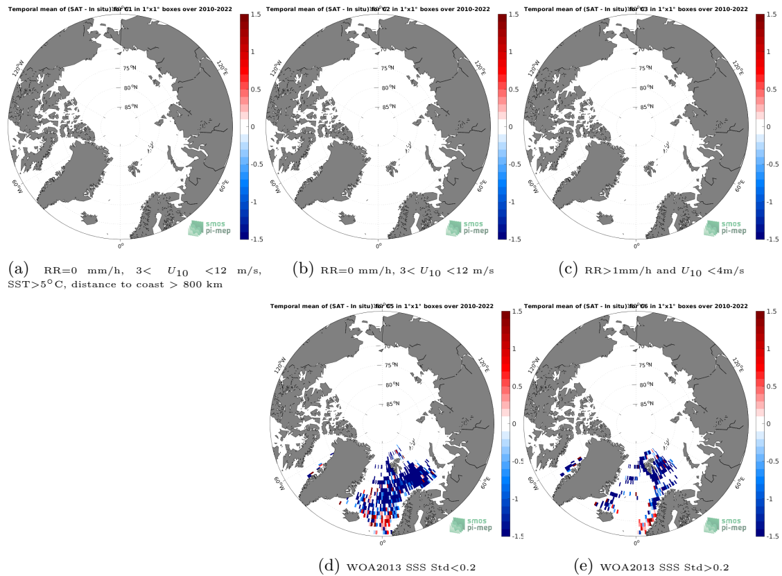
Figure 12: Temporal mean gridded over spatial boxes of size 1^{\circ}\times 1^{\circ} of \Delta\text{SSS} (SMOS SSS L2 v700 (ESA) - ICES) for 5 different subdatasets corresponding to: RR=0 mm/h, 3 < U_{10} < 12 m/s, SST > 5^{\circ}\text{C} , distance to coast > 800 km (a), RR=0 mm/h, 3 < U_{10} < 12 m/s (b), RR > 1 mm/h and U_{10} < 4 m/s (c), WOA2013 SSS Std < 0.2 (d), WOA2013 SSS Std > 0.2 (e).
