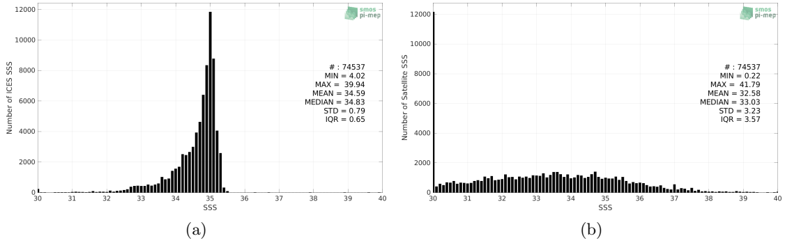
Figure 2: Histograms of SSS from ICES (a) and SMOS SSS L2 v700 (ESA) (b) considering all match-up pairs per bins of 0.1 over the Arctic Ocean Pi-MEP region and for the full satellite product period.
