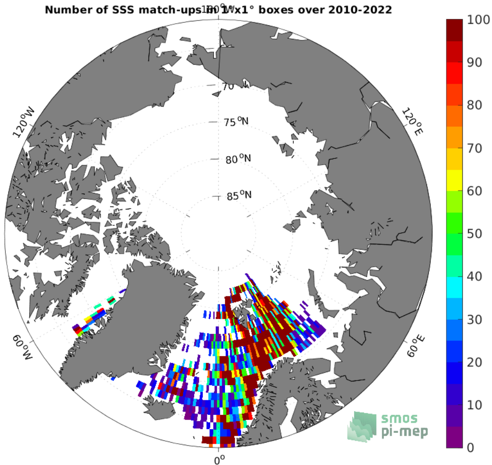
Figure 4: Number of SSS match-ups between ICES SSS and the SMOS SSS L2 v700 (ESA) SSS product for the Arctic Ocean Pi-MEP region over 1^\circ \times 1^\circ boxes and for the full satellite product period.
