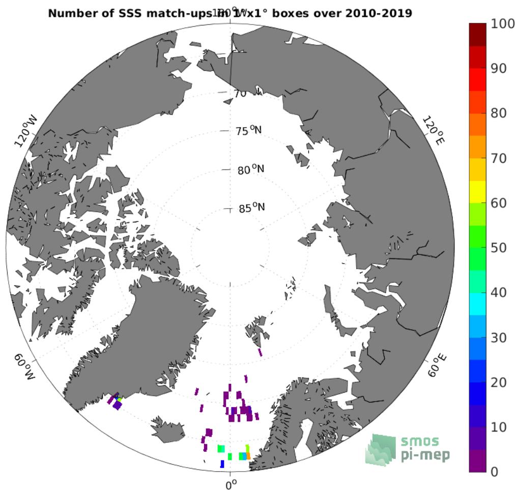
Figure 3: Number of SSS match-ups between Surface drifters SSS and the SMOS SSS L2 v700 (ESA) SSS product for the Arctic Ocean Pi-MEP region over 1^{\circ} \times 1^{\circ} boxes and for the full satellite product period.
