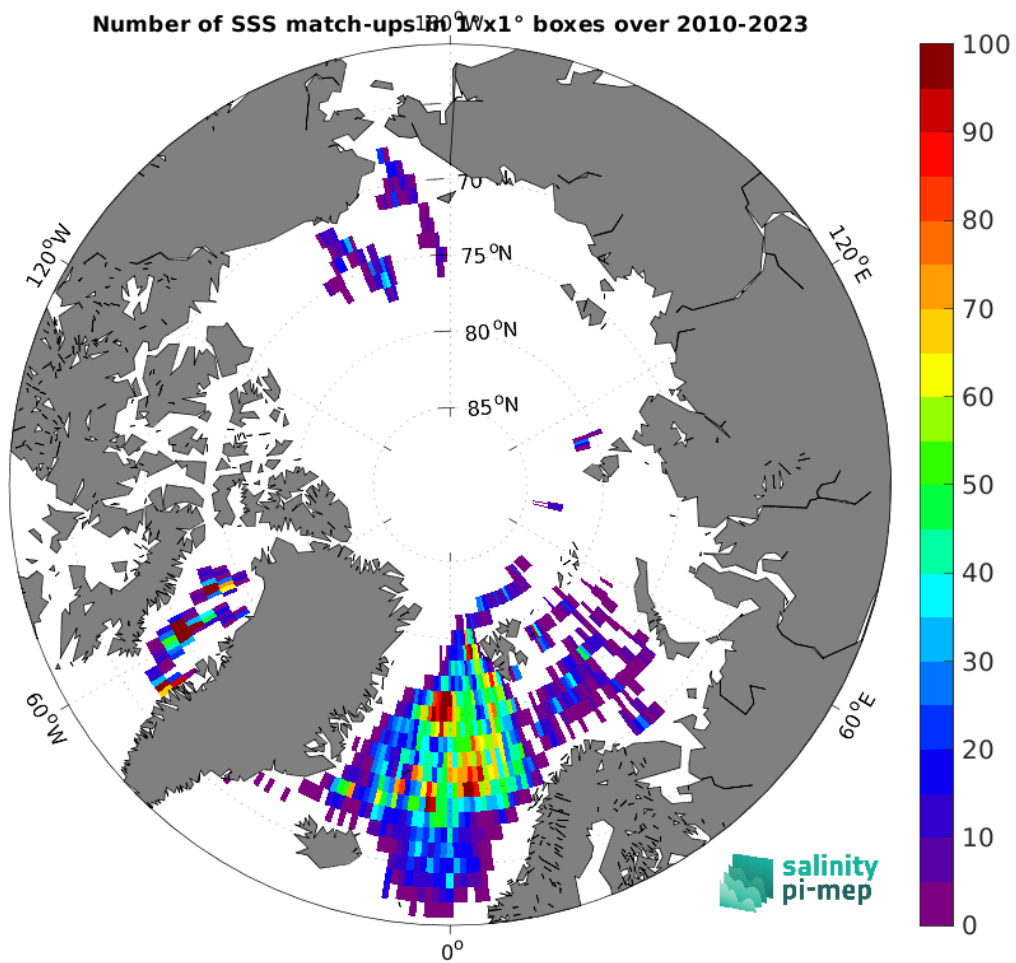
Figure 4: Number of SSS match-ups between Argo SSS and the SMOS SSS L2 v700 (ESA) SSS product for the Arctic Ocean Pi-MEP region over 1^\circ \times 1^\circ boxes and for the full satellite product period.
