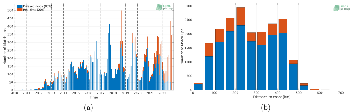
Figure 1: Number of match-ups between Argo and SMOS SSS L2 v700 (ESA) SSS as a function of time (a) and as function of the distance to coast (b) over the Arctic Ocean Pi-MEP region and for the full satellite product period.
