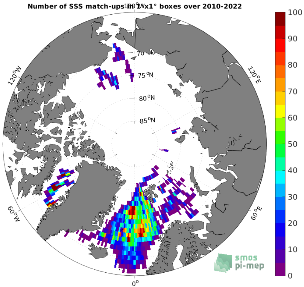
Figure 4: Number of SSS match-ups between Argo SSS and the SMOS SSS L2 v700 (ESA) SSS product for the Arctic Ocean Pi-MEP region over 1^{\circ} \times 1^{\circ} boxes and for the full satellite product period.
