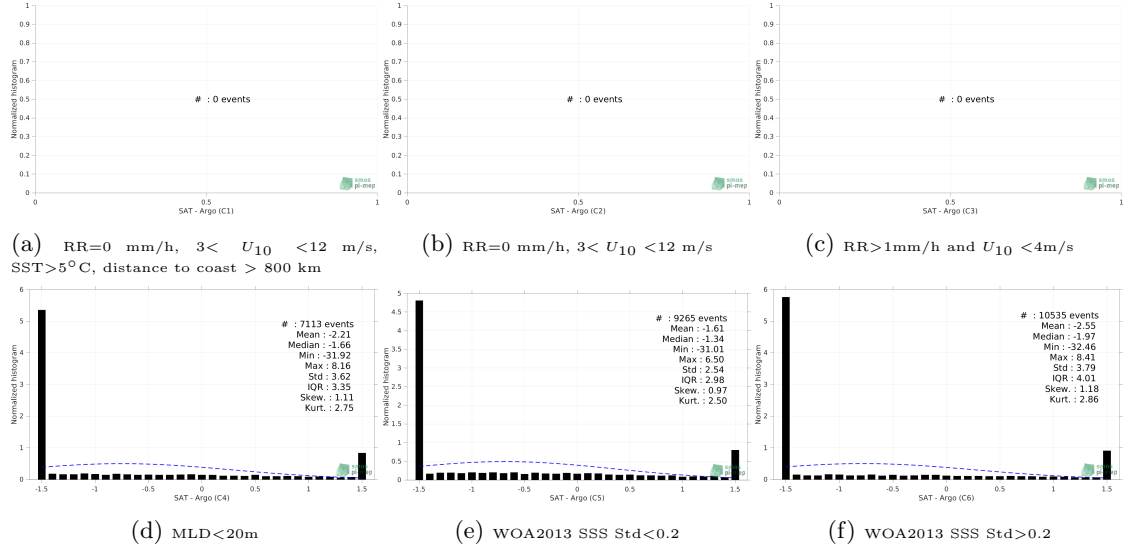
Figure 13: Normalized histogram of \Delta SSS (SMOS SSS L2 v700 (ESA) - Argo) for 6 different subdatasets corresponding to: RR=0 mm/h, 3 < U_{10} < 12 m/s, SST > 5°C, distance to coast > 800 km (a), RR=0 mm/h, 3 < U_{10} < 12 m/s (b), RR > 1mm/h and U_{10} < 4 m/s (c), MLD < 20m (d), WOA2013 SSS Std < 0.2 (e), WOA2013 SSS Std > 0.2 (f).
