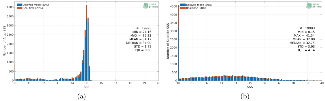
Figure 2: Histograms of SSS from Argo (a) and SMOS SSS L2 v700 (ESA) (b) considering all match-up pairs per bins of 0.1 over the Arctic Ocean Pi-MEP region and for the full satellite product period.
