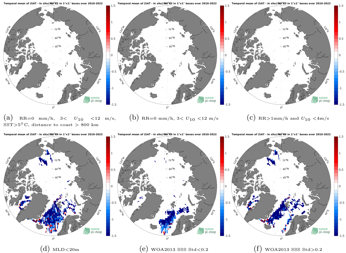
Figure 12: Temporal mean gridded over spatial boxes of size 1^{\circ}\times 1^{\circ} of \Delta\text{SSS} (SMOS SSS L2 v700 (ESA) - Argo) for 6 different subdatasets corresponding to:RR=0 mm/h, 3 < U_{10} < 12 m/s, SST > 5^{\circ}\text{C} , distance to coast > 800 km (a), RR=0 mm/h, 3 < U_{10} < 12 m/s (b), RR > 1\text{mm/h} and U_{10} < 4\text{m/s} (c),MLD < 20\text{m} (d),WOA2013 SSS Std < 0.2 (e),WOA2013 SSS Std > 0.2 (f).
