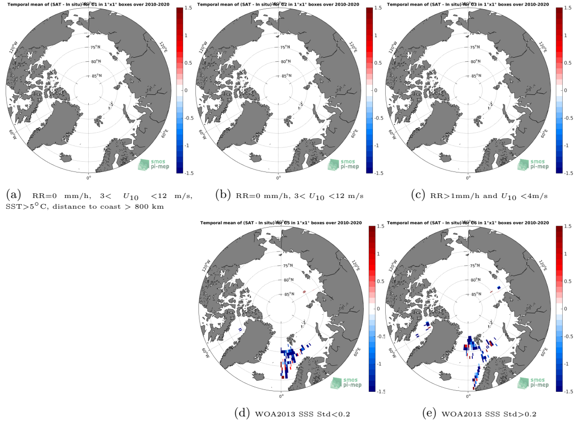
Figure 12: Temporal mean gridded over spatial boxes of size 1^{\circ}\times 1^{\circ} of \Delta\text{SSS} (SMOS SSS L2 v662 (ESA) - TSG (Polarstern)) for 5 different subdatasets corresponding to: RR=0 mm/h, 3 < U_{10} < 12 m/s, SST > 5^{\circ}\text{C} , distance to coast > 800 km (a), RR=0 mm/h, 3 < U_{10} < 12 m/s (b), RR > 1 mm/h and U_{10} < 4 m/s (c), WOA2013 SSS Std < 0.2 (d), WOA2013 SSS Std > 0.2 (e).
