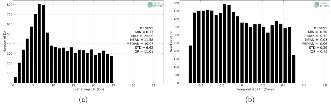
Figure 5: Histograms of the spatial (a) and temporal (b) lags between the location/time of the TSG (Polarstern) measurement and the date of the corresponding SMOS SSS L2 v662 (ESA) SSS pixel.
