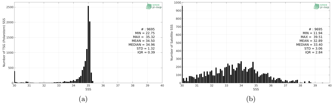
Figure 2: Histograms of SSS from TSG (Polarstern) (a) and SMOS SSS L2 v662 (ESA) (b) considering all match-up pairs per bins of 0.1 over the Arctic Ocean Pi-MEP region and for the full satellite product period.
