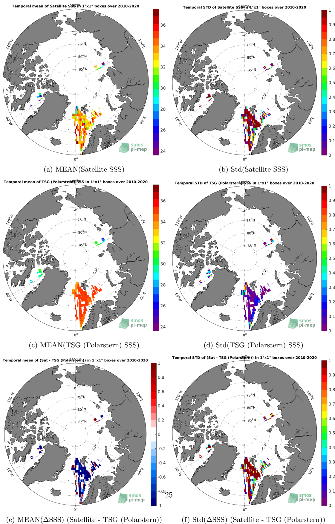
Figure 6: Temporal mean (left) and Std (right) of SSS from SMOS SSS L2 v662 (ESA) (top), TSG (Polarstern) (middle), and of \Delta SSS (Satellite - TSG (Polarstern)). Only match-up pairs are used to generate these maps.
