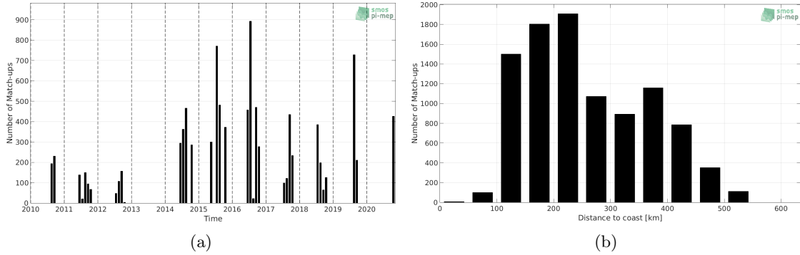
Figure 1: Number of match-ups between TSG (Polarstern) and SMOS SSS L2 v662 (ESA) SSS as a function of time (a) and as function of the distance to coast (b) over the Arctic Ocean Pi-MEP region and for the full satellite product period.
