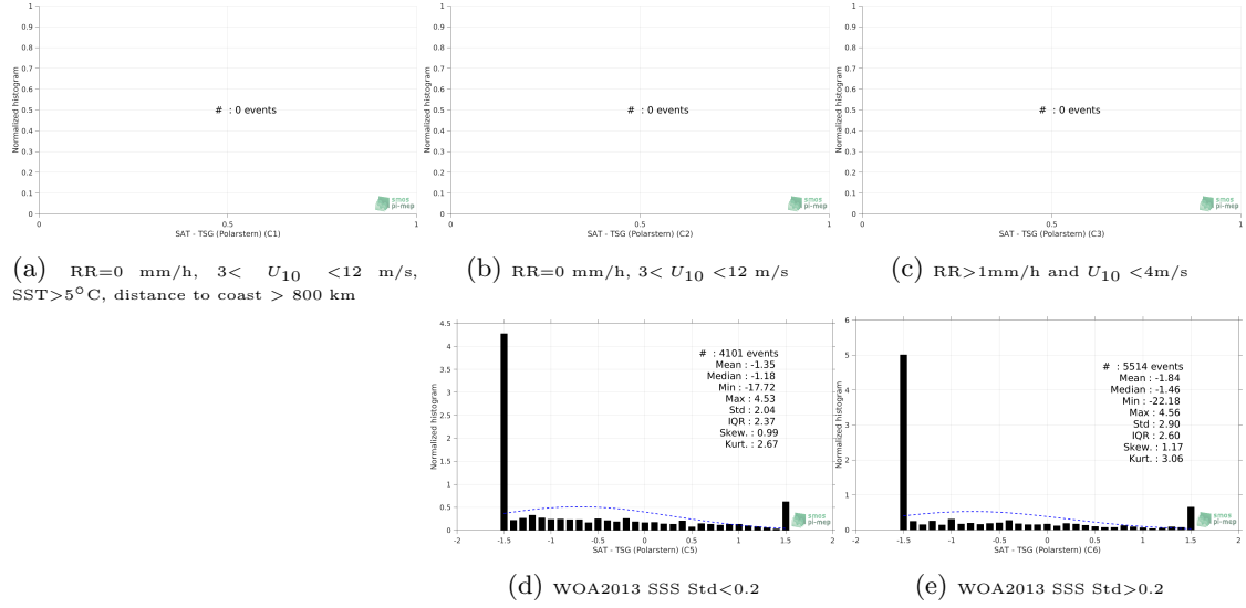
Figure 13: Normalized histogram of \Delta\text{SSS} (SMOS SSS L2 v662 (ESA) - TSG (Polarstern)) for 5 different subdatasets corresponding to: RR=0 mm/h, 3 < U_{10} < 12 m/s, SST > 5^\circ\text{C} , distance to coast > 800 km (a), RR=0 mm/h, 3 < U_{10} < 12 m/s (b), RR > 1 mm/h and U_{10} < 4 m/s (c), WOA2013 SSS Std < 0.2 (d), WOA2013 SSS Std > 0.2 (e).
