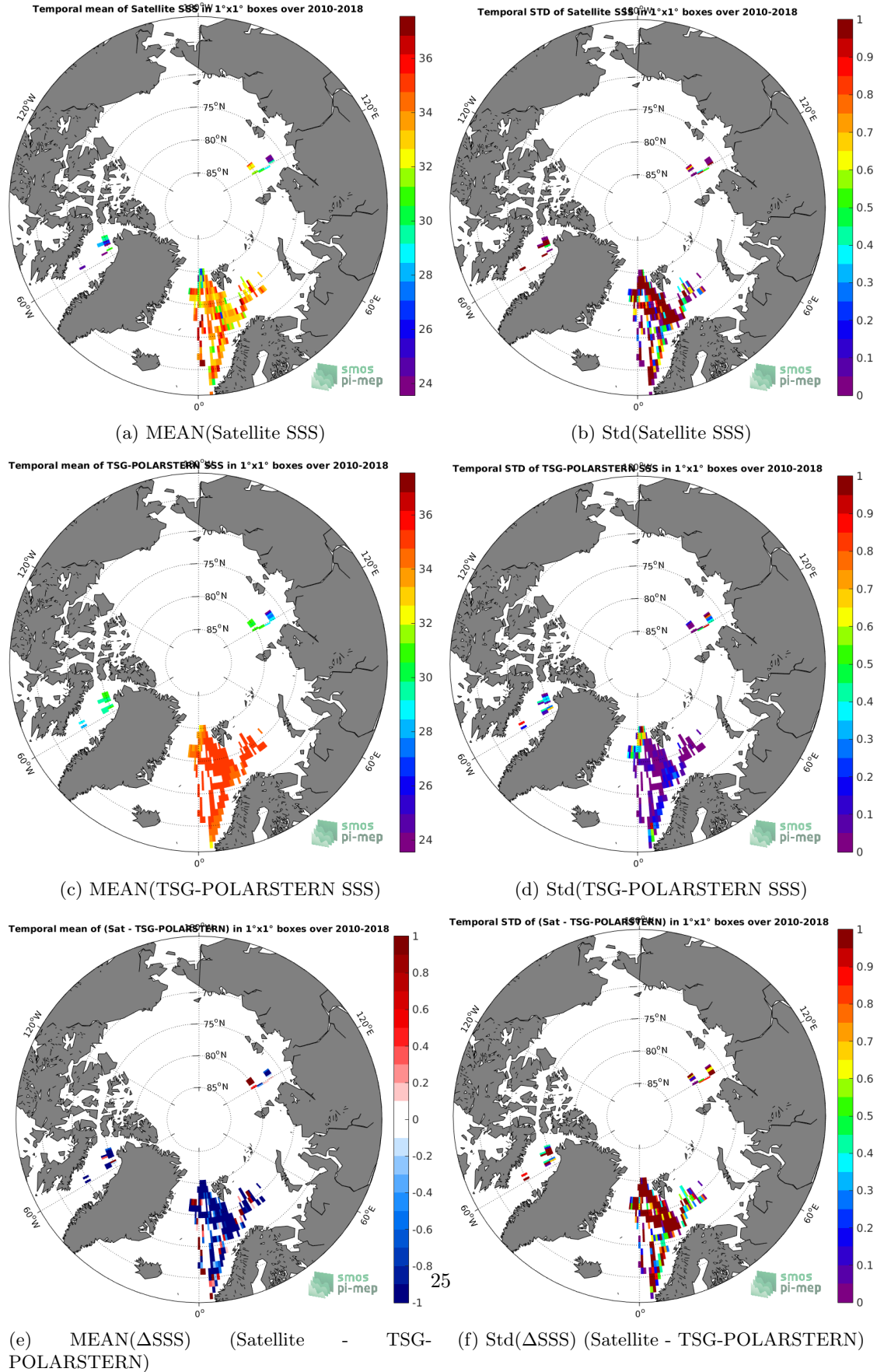
Figure 6: Temporal mean (left) and Std (right) of SSS from SMOS L2 v662 (ESA) (top), TSG-POLARSTERN (middle), and of \Delta SSS (Satellite - TSG-POLARSTERN). Only match-up pairs are used to generate these maps.
