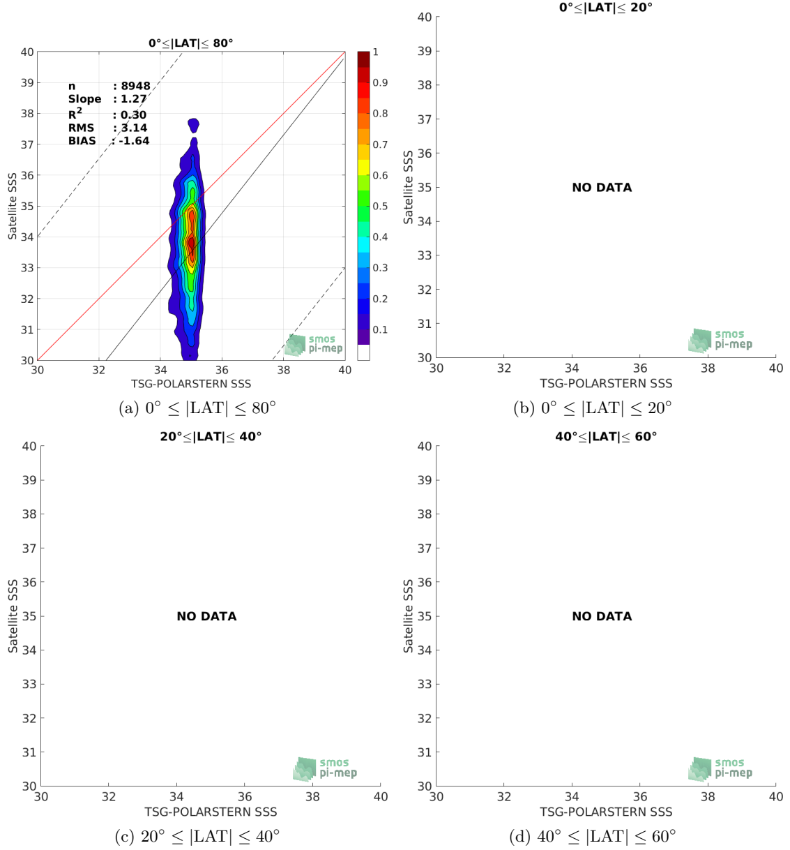
Figure 9: Contour maps of the concentration of SMOS L2 v662 (ESA) SSS (y-axis) versus TSG-POLARSTERN SSS (x-axis) at match-up pairs for different latitude bands. For each plot, the red line shows x=y . The black thin and dashed lines indicate a linear fit through the data cloud and the \pm 95\% confidence levels, respectively. The number match-up pairs n , the slope and R^2 coefficient of the linear fit, the root mean square (RMS) and the mean bias between satellite and in situ data are indicated for each latitude band in each plots.
