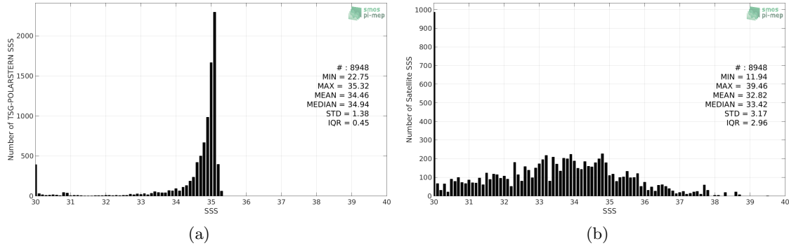
Figure 2: Histograms of SSS from TSG-POLARSTERN (a) and SMOS L2 v662 (ESA) (b) considering all match-up pairs per bins of 0.1 over the Arctic Ocean Pi-MEP region and for the full satellite product period.
