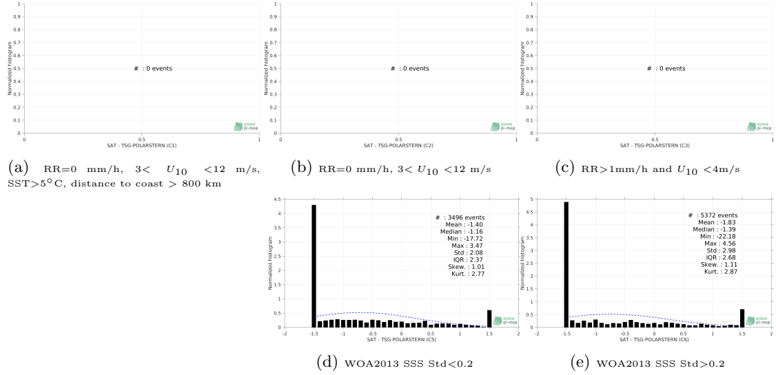
Figure 13: Normalized histogram of \Delta\text{SSS} (SMOS L2 v662 (ESA) - TSG-POLARSTERN) for 5 different subdatasets corresponding to: RR=0 mm/h, 3 < U_{10} < 12 m/s, SST > 5^\circ\text{C} , distance to coast > 800 km (a), RR=0 mm/h, 3 < U_{10} < 12 m/s (b), RR > 1 mm/h and U_{10} < 4 m/s (c), WOA2013 SSS Std < 0.2 (d), WOA2013 SSS Std > 0.2 (e).
