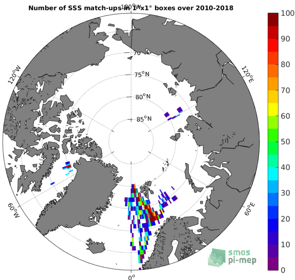
Figure 4: Number of SSS match-ups between TSG-POLARSTERN SSS and the SMOS L2 v662 (ESA) SSS product for the Arctic Ocean Pi-MEP region over 1°x1° boxes and for the full satellite product period.
