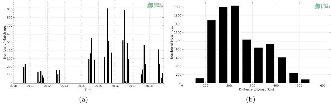
Figure 1: Number of match-ups between TSG-POLARSTERN and SMOS L2 v662 (ESA) SSS as a function of time (a) and as function of the distance to coast (b) over the Arctic Ocean Pi-MEP region and for the full satellite product period.
