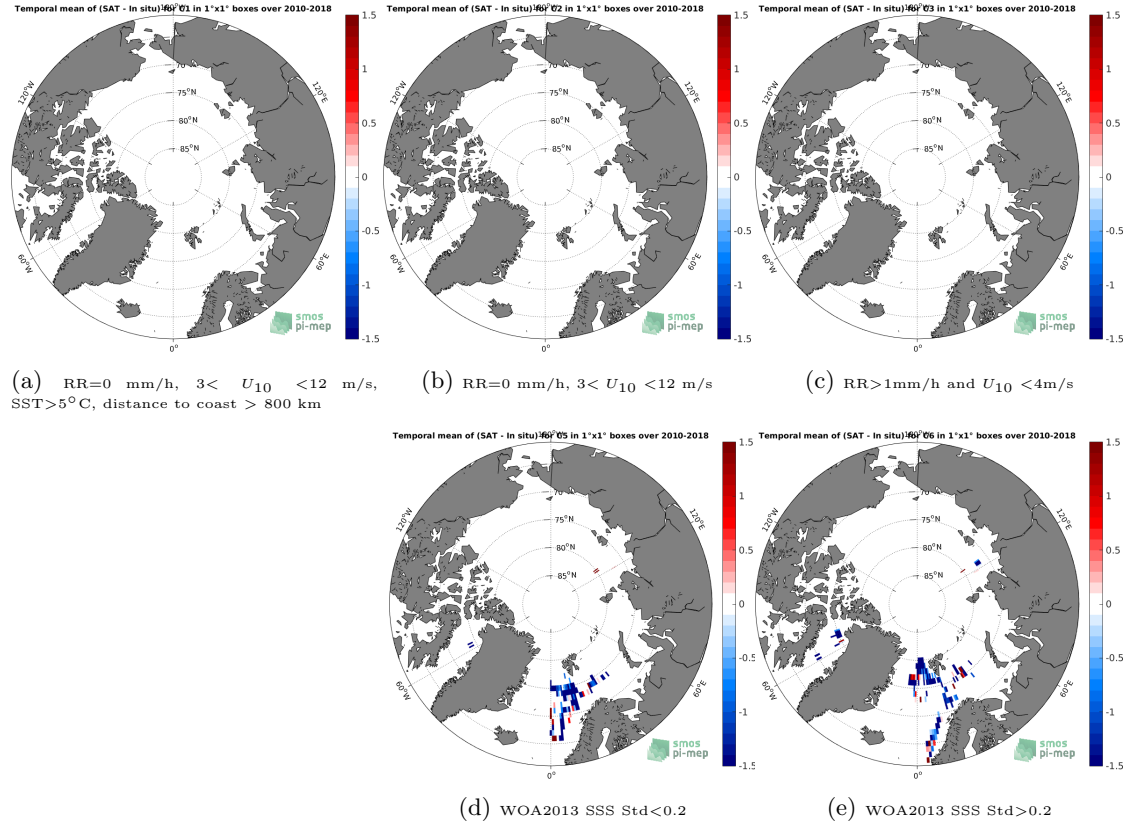
Figure 12: Temporal mean gridded over spatial boxes of size 1^{\circ}\times 1^{\circ} of \Delta\text{SSS} (SMOS L2 v662 (ESA) - TSG-POLARSTERN) for 5 different subdatasets corresponding to: RR=0 mm/h, 3 < U_{10} < 12 m/s, SST > 5^{\circ}\text{C} , distance to coast > 800 km (a), RR=0 mm/h, 3 < U_{10} < 12 m/s (b), RR > 1 mm/h and U_{10} < 4 m/s (c), WOA2013 SSS Std < 0.2 (d), WOA2013 SSS Std > 0.2 (e).
