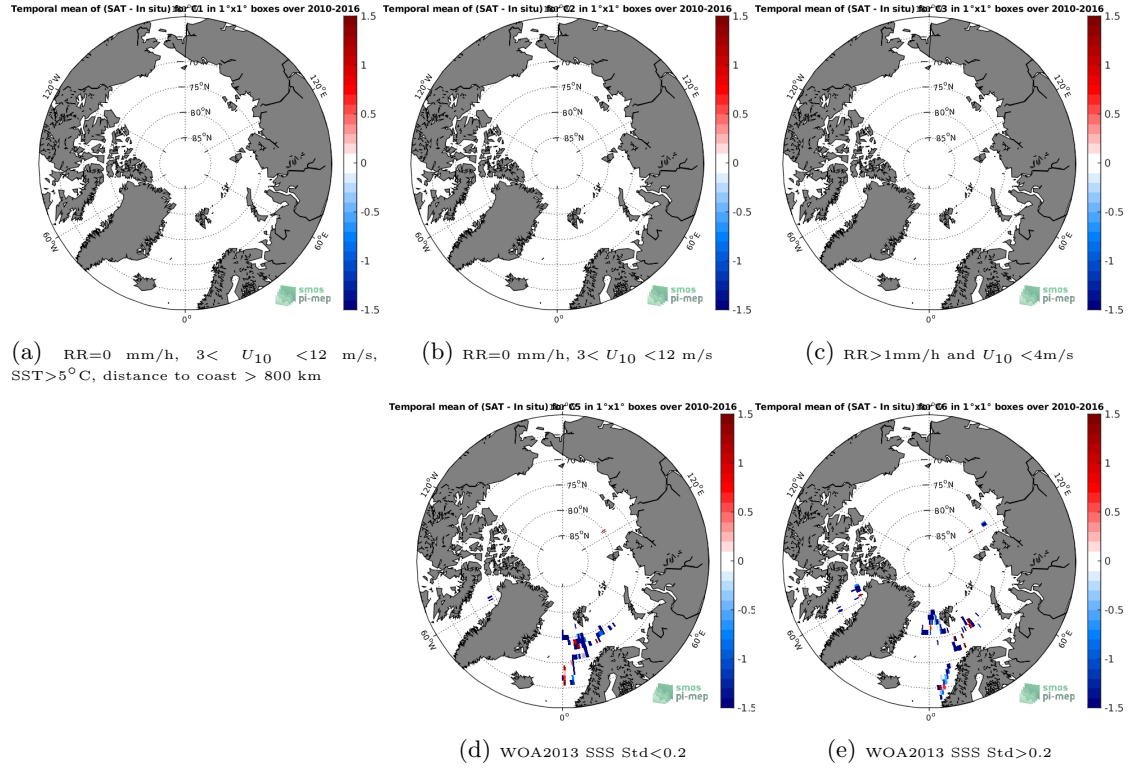
Figure 12: Temporal mean gridded over spatial boxes of size 1^\circ \times 1^\circ of \Delta SSS (SMOS-L2-DPGS-v662 - TSG-POLARSTERN) for 5 different subdatasets corresponding to:RR=0 mm/h, 3 < U_{10} < 12 m/s, SST >5^\circ C, distance to coast > 800 km (a), RR=0 mm/h, 3 < U_{10} < 12 m/s (b), RR >1 mm/h and U_{10} < 4 m/s (c), WOA2013 SSS Std <0.2 (d), WOA2013 SSS Std >0.2 (e).
