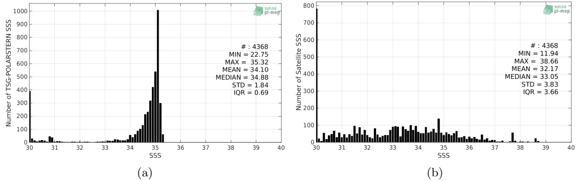
Figure 2: Histograms of SSS from TSG-POLARSTERN (a) and SMOS-L2-DPGS-v662 (b) considering all match-up pairs per bins of 0.1 over the Arctic Ocean Pi-MEP region and for the full satellite product period.
