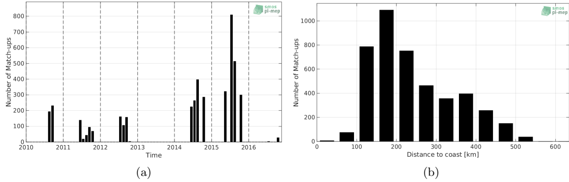
Figure 1: Number of match-ups between TSG-POLARSTERN and SMOS-L2-DPGS-v662 SSS as a function of time (a) and as function of the distance to coast (b) over the Arctic Ocean Pi-MEP region and for the full satellite product period.
