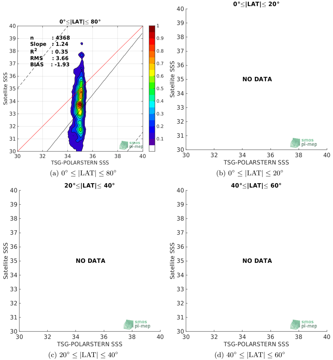
Figure 9: Contour maps of the concentration of SMOS-L2-DPGS-v662 SSS (y-axis) versus TSG-POLARSTERN SSS (x-axis) at match-up pairs for different latitude bands. For each plot, the red line shows x=y . The black thin and dashed lines indicate a linear fit through the data cloud and the \pm 95\% confidence levels, respectively. The number match-up pairs n , the slope and R^2 coefficient of the linear fit, the root mean square (RMS) and the mean bias between satellite and in situ data are indicated for each latitude band in each plots.
