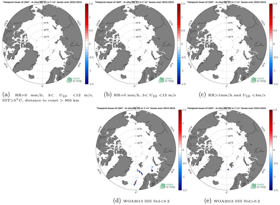
Figure 12: Temporal mean gridded over spatial boxes of size 1°x1° of \Delta SSS (SMOS SSS L2 v662 (ESA) - TSG (GOSUD-Sailing-ship)) for 5 different subdatasets corresponding to: RR=0 mm/h, 3 < U_{10} < 12 m/s, SST>5°C, distance to coast > 800 km (a), RR=0 mm/h, 3 < U_{10} < 12 m/s (b), RR>1mm/h and U_{10} < 4 m/s (c), WOA2013 SSS Std<0.2 (d), WOA2013 SSS Std>0.2 (e).
