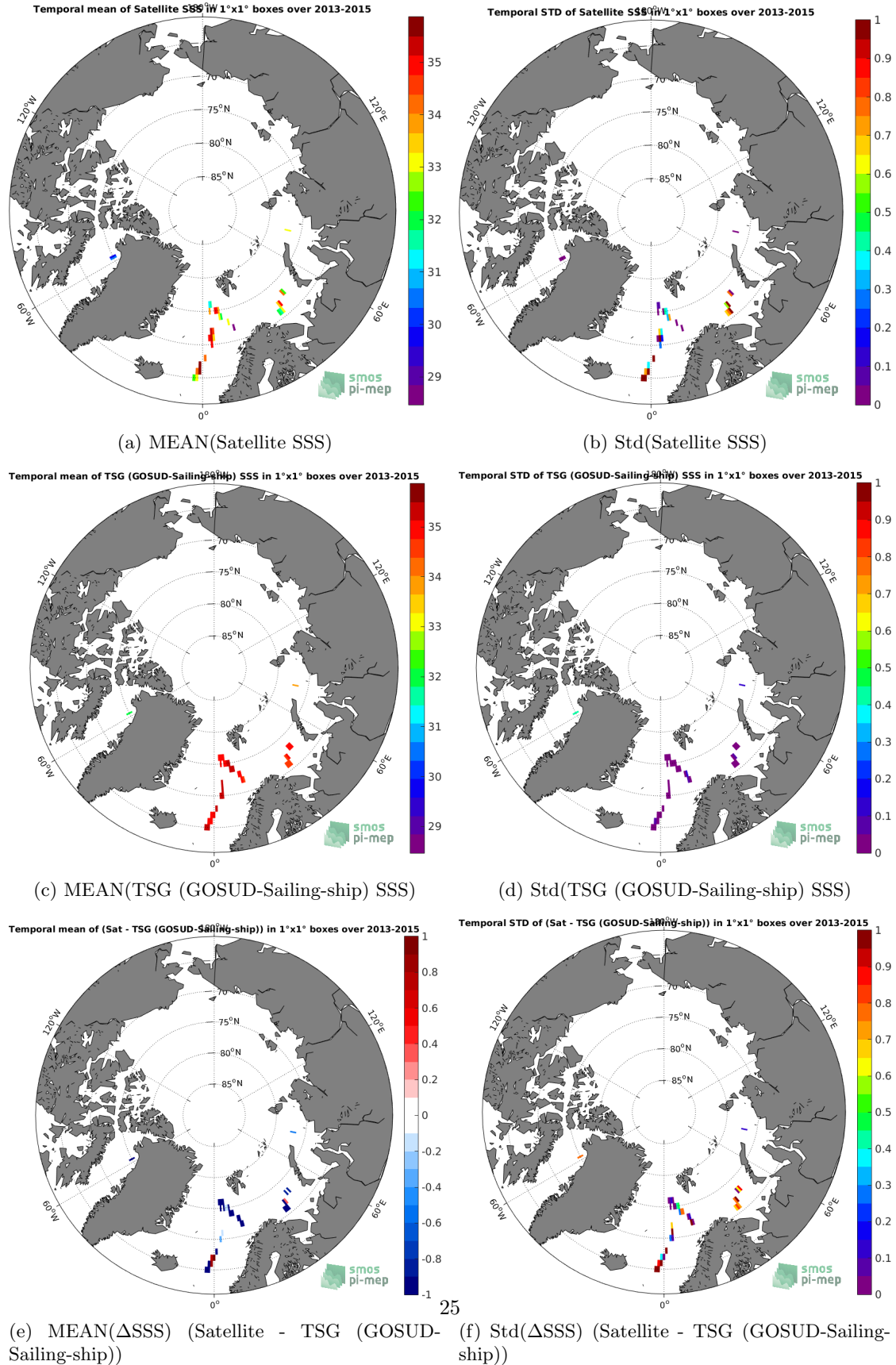
Figure 6: Temporal mean (left) and Std (right) of SSS from SMOS SSS L2 v662 (ESA) (top), TSG (GOSUD-Sailing-ship) (middle), and of \Delta SSS (Satellite - TSG (GOSUD-Sailing-ship)). Only match-up pairs are used to generate these maps.
