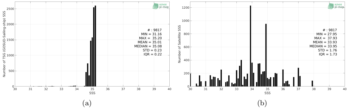
Figure 2: Histograms of SSS from TSG (GOSUD-Sailing-ship) (a) and SMOS SSS L2 v662 (ESA) (b) considering all match-up pairs per bins of 0.1 over the Arctic Ocean Pi-MEP region and for the full satellite product period.
