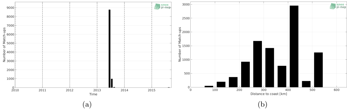
Figure 1: Number of match-ups between TSG (GOSUD-Sailing-ship) and SMOS SSS L2 v662 (ESA) SSS as a function of time (a) and as function of the distance to coast (b) over the Arctic Ocean Pi-MEP region and for the full satellite product period.
