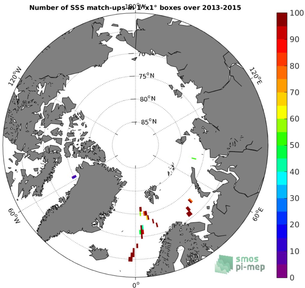
Figure 4: Number of SSS match-ups between TSG (GOSUD-Sailing-ship) SSS and the SMOS SSS L2 v662 (ESA) SSS product for the Arctic Ocean Pi-MEP region over 1°x1° boxes and for the full satellite product period.
