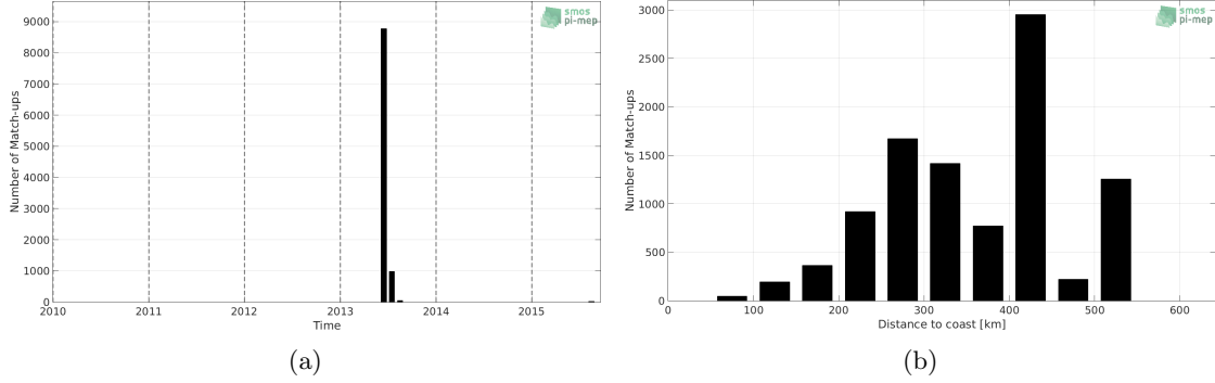
Figure 1: Number of match-ups between TSG-GOSUD-Sailing-ship and SMOS L2 v662 (ESA) SSS as a function of time (a) and as function of the distance to coast (b) over the Arctic Ocean Pi-MEP region and for the full satellite product period.
