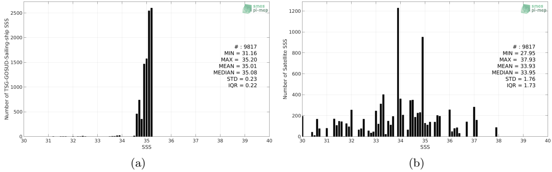
Figure 2: Histograms of SSS from TSG-GOSUD-Sailing-ship (a) and SMOS L2 v662 (ESA) (b) considering all match-up pairs per bins of 0.1 over the Arctic Ocean Pi-MEP region and for the full satellite product period.
