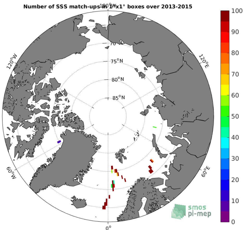
Figure 4: Number of SSS match-ups between TSG-GOSUD-Sailing-ship SSS and the SMOS L2 v662 (ESA) SSS product for the Arctic Ocean Pi-MEP region over 1^\circ \times 1^\circ boxes and for the full satellite product period.
