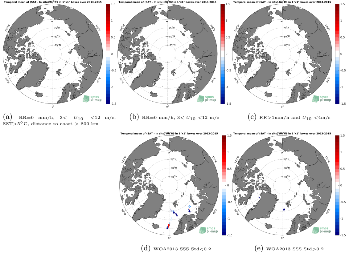
Figure 12: Temporal mean gridded over spatial boxes of size 1^{\circ} \times 1^{\circ} of \Delta\text{SSS} (SMOS L2 v662 (ESA) - TSG-GOSUD-Sailing-ship) for 5 different subdatasets corresponding to: RR=0 mm/h, 3 < U_{10} < 12 m/s, SST > 5^{\circ}\text{C} , distance to coast > 800 km (a), RR=0 mm/h, 3 < U_{10} < 12 m/s (b), RR > 1\text{mm/h} and U_{10} < 4\text{m/s} (c), WOA2013 SSS Std < 0.2 (d), WOA2013 SSS Std > 0.2 (e).
