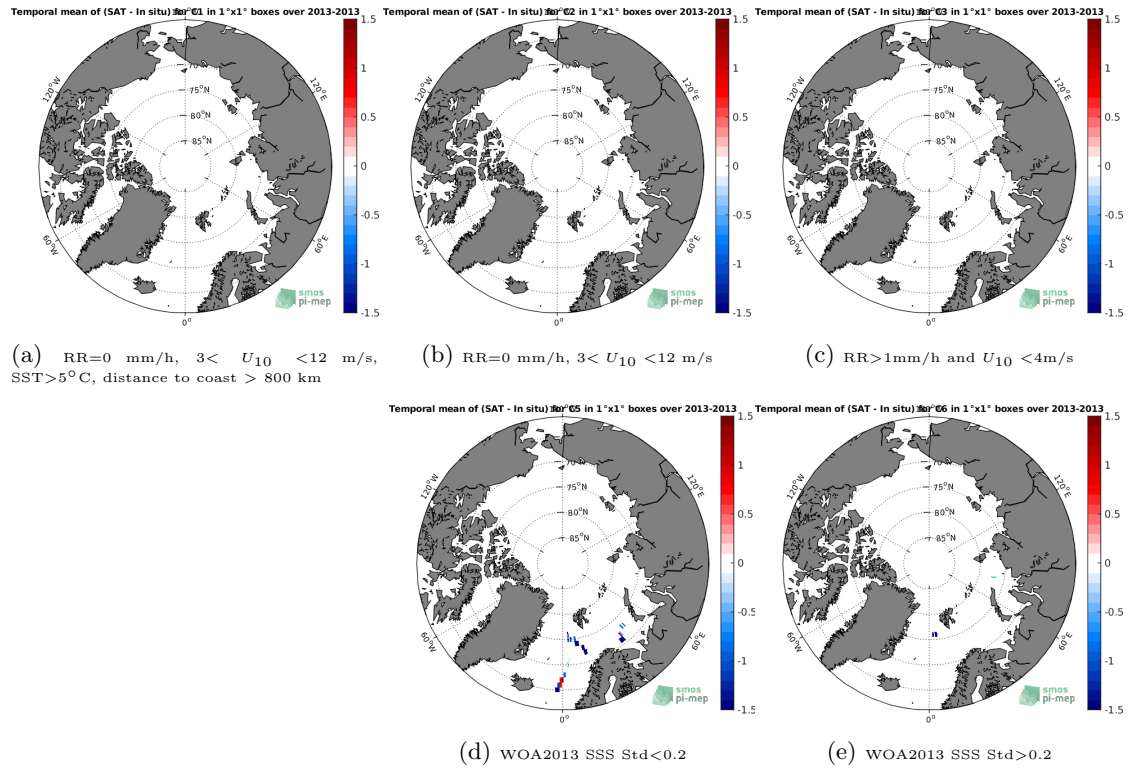
Figure 12: Temporal mean gridded over spatial boxes of size 1^\circ \times 1^\circ of \Delta SSS (SMOS-L2-DPGS-v662 - TSG-GOSUD-Sailing-ship) for 5 different subdatasets corresponding to:RR=0 mm/h, 3 < U_{10} < 12 m/s, SST >5^\circ\text{C} , distance to coast > 800 km (a), RR=0 mm/h, 3 < U_{10} < 12 m/s (b), RR >1 mm/h and U_{10} < 4 m/s (c), WOA2013 SSS Std <0.2 (d), WOA2013 SSS Std >0.2 (e).
