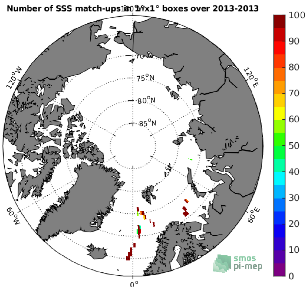
Figure 4: Number of SSS match-ups between TSG-GOSUD-Sailing-ship SSS and the SMOS-L2-DPGS-v662 SSS product for the Arctic Ocean Pi-MEP region over 1°x1° boxes and for the full satellite product period.
