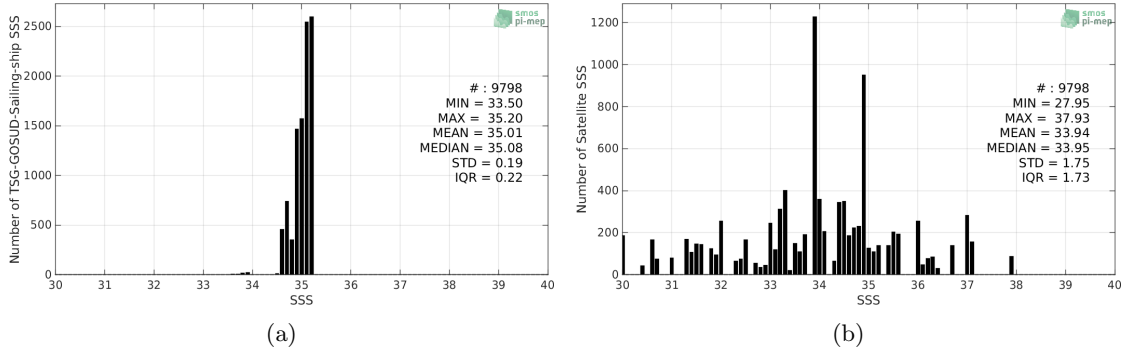
Figure 2: Histograms of SSS from TSG-GOSUD-Sailing-ship (a) and SMOS-L2-DPGS-v662 (b) considering all match-up pairs per bins of 0.1 over the Arctic Ocean Pi-MEP region and for the full satellite product period.
