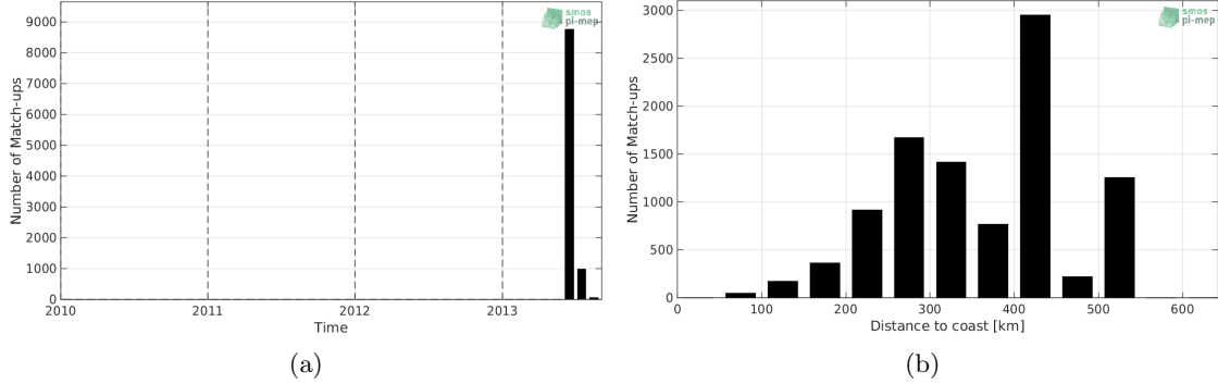
Figure 1: Number of match-ups between TSG-GOSUD-Sailing-ship and SMOS-L2-DPGS-v662 SSS as a function of time (a) and as function of the distance to coast (b) over the Arctic Ocean Pi-MEP region and for the full satellite product period.
