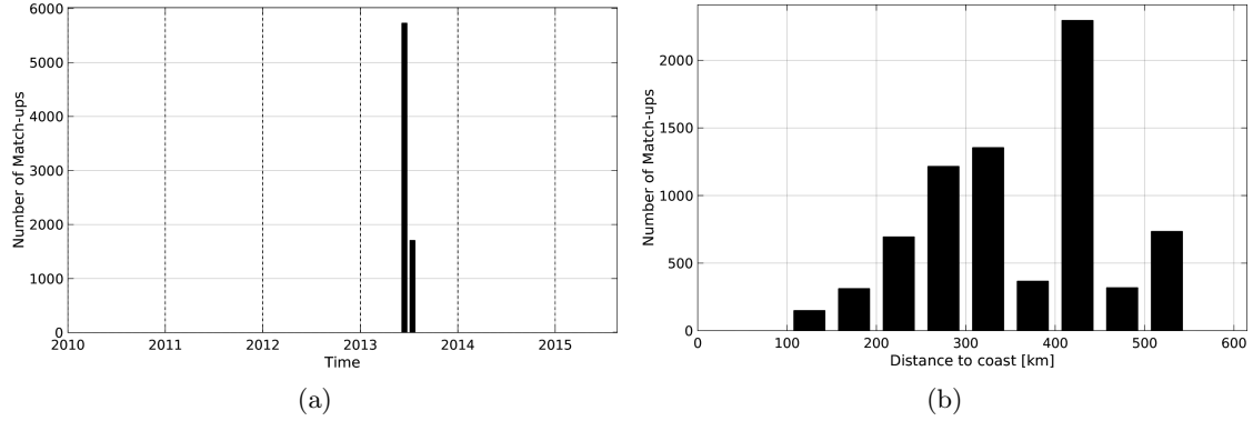
Figure 1: Number of match-ups between TSG-GOSUD-Sailing-ship and SMOS-L2-DPGS-v662 SSS as a function of time (a) and as function of the distance to coast (b) over the Arctic Ocean Pi-MEP region and for the full satellite product period.
