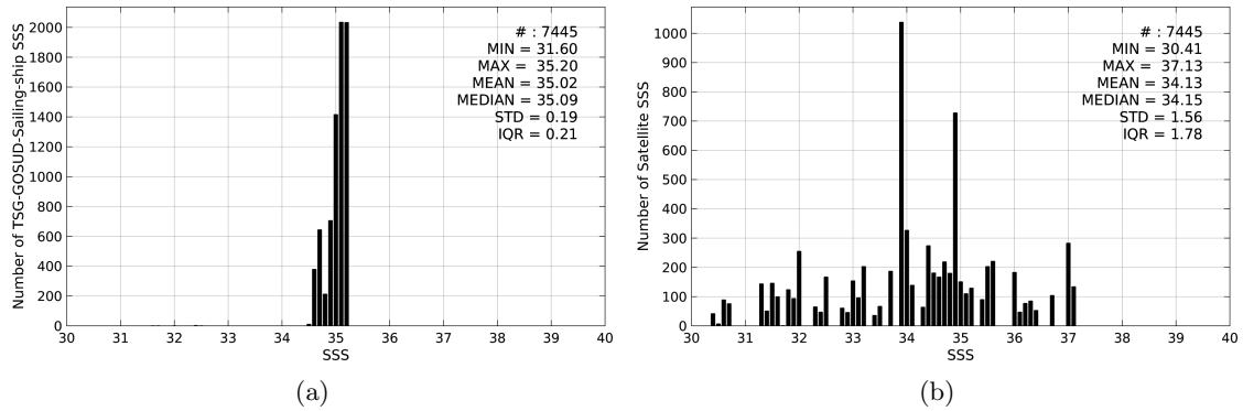
Figure 2: Histograms of SSS from TSG-GOSUD-Sailing-ship (a) and SMOS-L2-DPGS-v662 (b) considering all match-up pairs per bins of 0.1 over the Arctic Ocean Pi-MEP region and for the full satellite product period.
