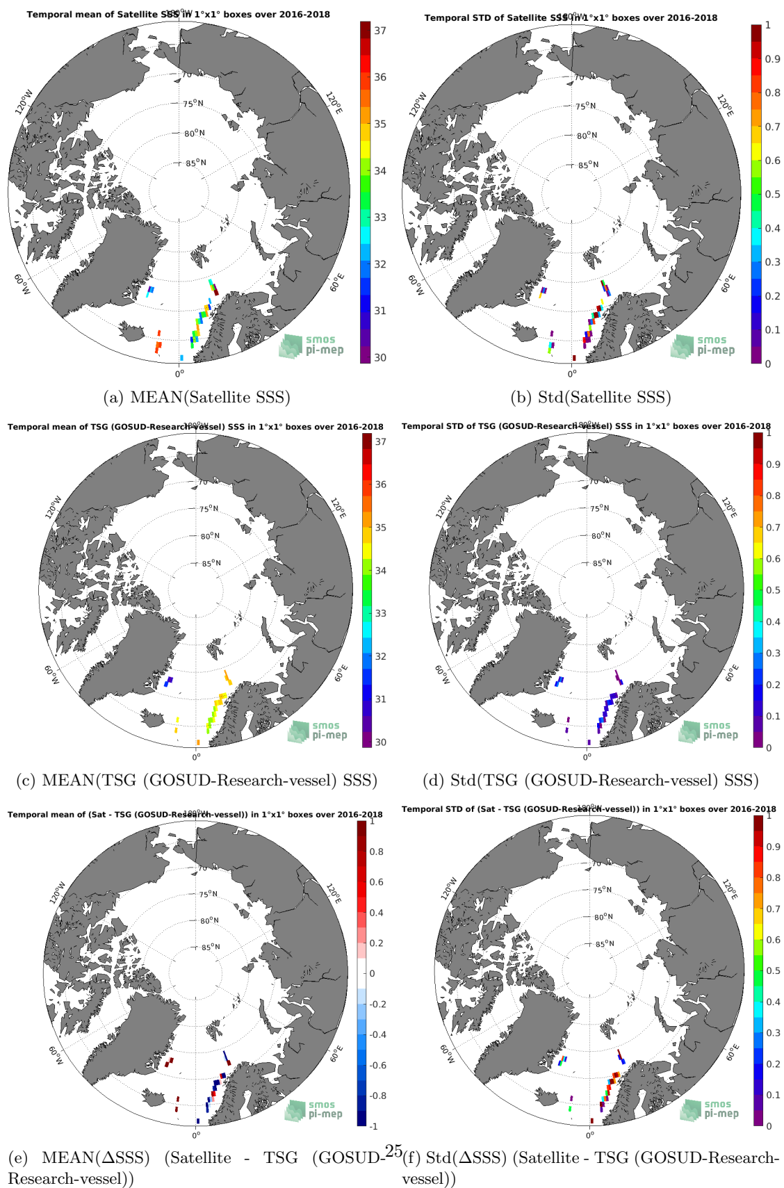
Figure 6: Temporal mean (left) and Std (right) of SSS from SMOS SSS L2 v662 (ESA) (top), TSG (GOSUD-Research-vessel) (middle), and of \Delta SSS (Satellite - TSG (GOSUD-Research-vessel)). Only match-up pairs are used to generate these maps.
