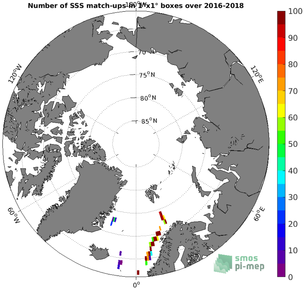
Figure 4: Number of SSS match-ups between TSG (GOSUD-Research-vessel) SSS and the SMOS SSS L2 v662 (ESA) SSS product for the Arctic Ocean Pi-MEP region over 1^\circ \times 1^\circ boxes and for the full satellite product period.
