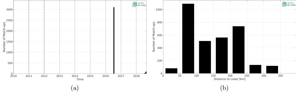
Figure 1: Number of match-ups between TSG (GOSUD-Research-vessel) and SMOS SSS L2 v662 (ESA) SSS as a function of time (a) and as function of the distance to coast (b) over the Arctic Ocean Pi-MEP region and for the full satellite product period.
