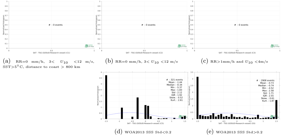
Figure 13: Normalized histogram of \Delta\text{SSS} (SMOS SSS L2 v662 (ESA) - TSG (GOSUD-Research-vessel)) for 5 different subdatasets corresponding to: RR=0 mm/h, 3 < U_{10} < 12 m/s, SST > 5^\circ\text{C} , distance to coast > 800 km (a), RR=0 mm/h, 3 < U_{10} < 12 m/s (b), RR > 1\text{mm/h} and U_{10} < 4\text{m/s} (c), WOA2013 SSS Std<0.2 (d), WOA2013 SSS Std>0.2 (e).
