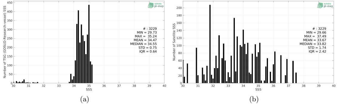
Figure 2: Histograms of SSS from TSG (GOSUD-Research-vessel) (a) and SMOS SSS L2 v662 (ESA) (b) considering all match-up pairs per bins of 0.1 over the Arctic Ocean Pi-MEP region and for the full satellite product period.
