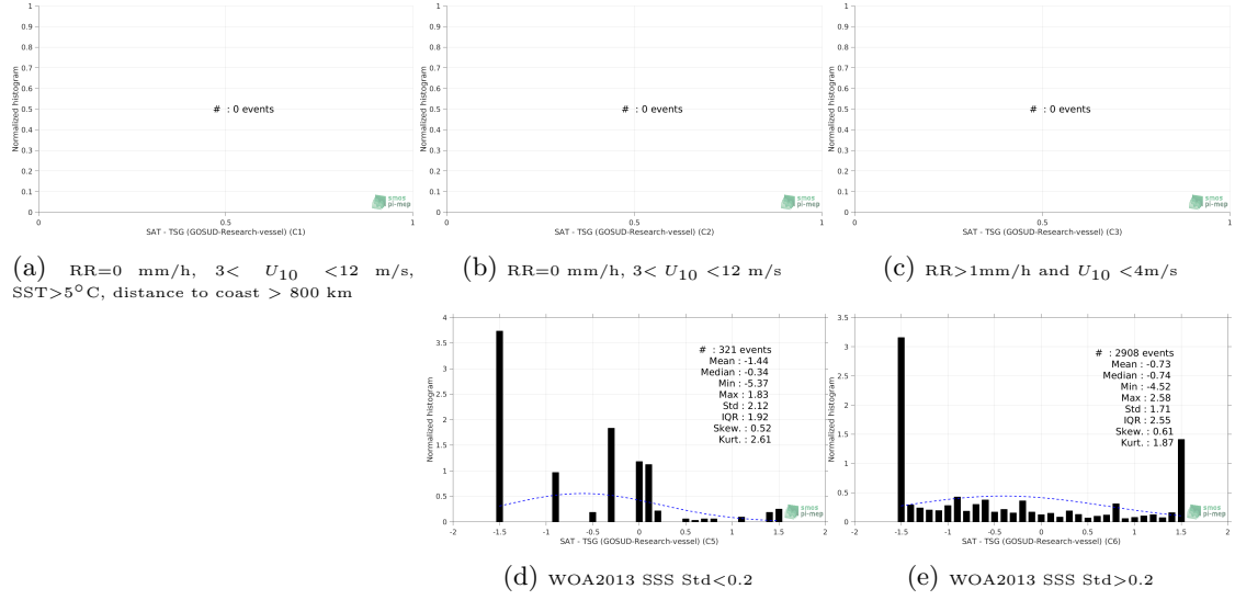
Figure 13: Normalized histogram of \Delta\text{SSS} (SMOS SSS L2 v662 (ESA) - TSG (GOSUD-Research-vessel)) for 5 different subdatasets corresponding to: RR=0 mm/h, 3 < U_{10} < 12 m/s, SST > 5^\circ\text{C} , distance to coast > 800 km (a), RR=0 mm/h, 3 < U_{10} < 12 m/s (b), RR > 1\text{mm/h} and U_{10} < 4\text{m/s} (c), WOA2013 SSS Std<0.2 (d), WOA2013 SSS Std>0.2 (e).
