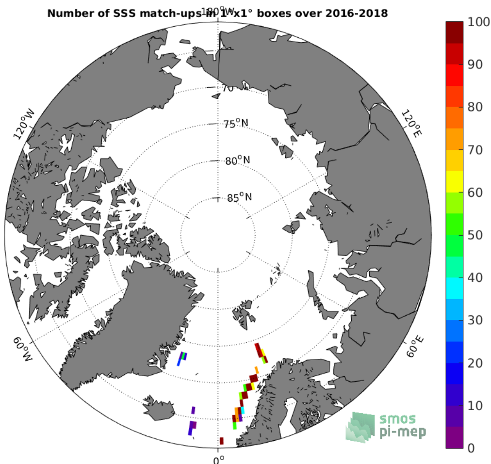
Figure 4: Number of SSS match-ups between TSG (GOSUD-Research-vessel) SSS and the SMOS SSS L2 v662 (ESA) SSS product for the Arctic Ocean Pi-MEP region over 1°x1° boxes and for the full satellite product period.
