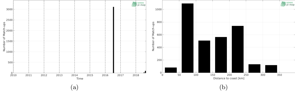
Figure 1: Number of match-ups between TSG-GOSUD-Research-vessel and SMOS L2 v662 (ESA) SSS as a function of time (a) and as function of the distance to coast (b) over the Arctic Ocean Pi-MEP region and for the full satellite product period.
