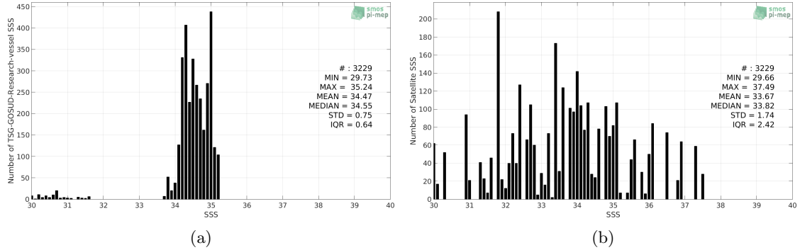
Figure 2: Histograms of SSS from TSG-GOSUD-Research-vessel (a) and SMOS L2 v662 (ESA) (b) considering all match-up pairs per bins of 0.1 over the Arctic Ocean Pi-MEP region and for the full satellite product period.
