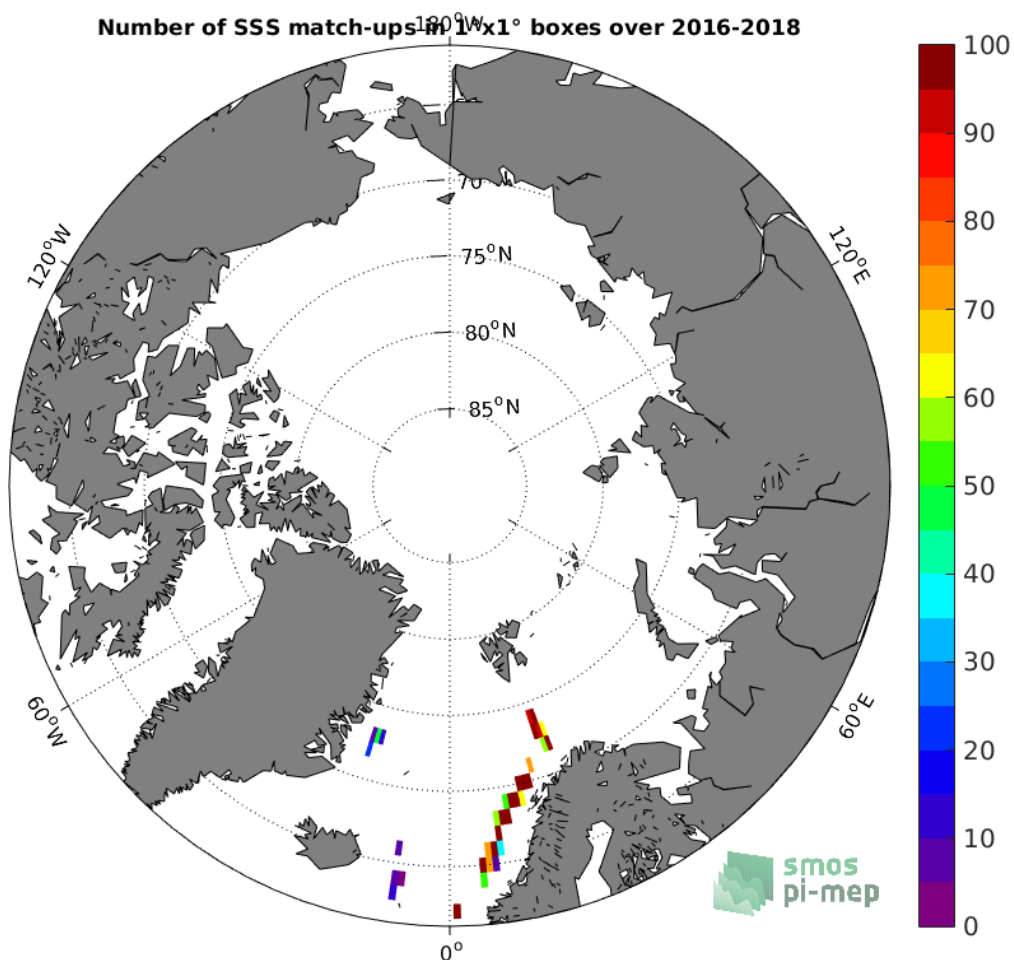
Figure 4: Number of SSS match-ups between TSG-GOSUD-Research-vessel SSS and the SMOS L2 v662 (ESA) SSS product for the Arctic Ocean Pi-MEP region over 1°x1° boxes and for the full satellite product period.
