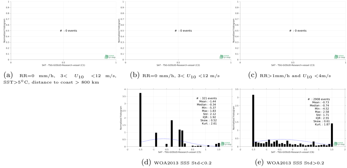
Figure 13: Normalized histogram of \Delta\text{SSS} (SMOS L2 v662 (ESA) - TSG-GOSUD-Research-vessel) for 5 different subdatasets corresponding to: RR=0 mm/h, 3 < U_{10} < 12 m/s, SST > 5^\circ\text{C} , distance to coast > 800 km (a), RR=0 mm/h, 3 < U_{10} < 12 m/s (b), RR > 1\text{mm/h} and U_{10} < 4\text{m/s} (c), WOA2013 SSS Std<0.2 (d), WOA2013 SSS Std>0.2 (e).
