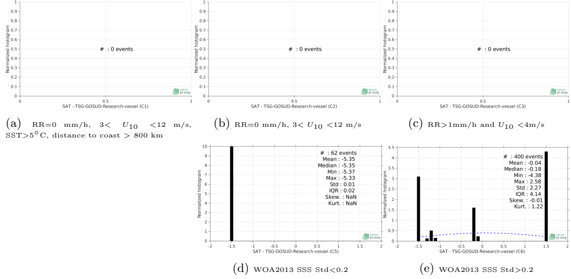
Figure 13: Normalized histogram of \Delta\text{SSS} (SMOS-L2-DPGS-v662 - TSG-GOSUD-Research-vessel) for 5 different subdatasets corresponding to: RR=0 mm/h, 3 < U_{10} < 12 m/s, SST > 5^{\circ}\text{C} , distance to coast > 800 km (a), RR=0 mm/h, 3 < U_{10} < 12 m/s (b), RR > 1 mm/h and U_{10} < 4 m/s (c), WOA2013 SSS Std < 0.2 (d), WOA2013 SSS Std > 0.2 (e).
