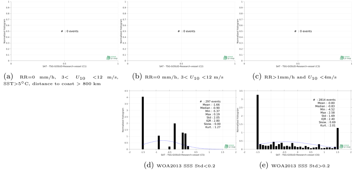
Figure 13: Normalized histogram of \Delta\text{SSS} (SMOS-L2-DPGS-v662 - TSG-GOSUD-Research-vessel) for 5 different subdatasets corresponding to: RR=0 mm/h, 3 < U_{10} < 12 m/s, SST >5^{\circ}\text{C} , distance to coast > 800 km (a), RR=0 mm/h, 3 < U_{10} < 12 m/s (b), RR>1\text{mm/h} and U_{10} < 4\text{m/s} (c), WOA2013 SSS Std <0.2 (d), WOA2013 SSS Std >0.2 (e).
