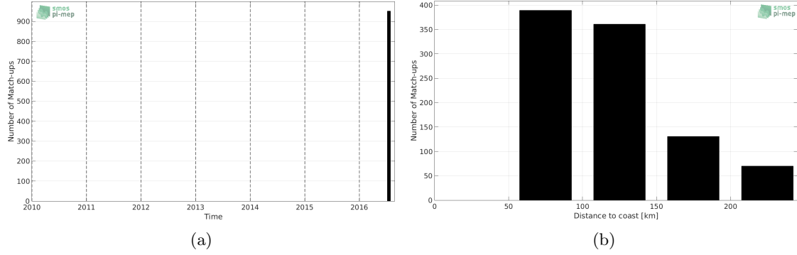
Figure 1: Number of match-ups between TSG-GOSUD-Research-vessel and SMOS-L2-DPGS-v662 SSS as a function of time (a) and as function of the distance to coast (b) over the Arctic Ocean Pi-MEP region and for the full satellite product period.
