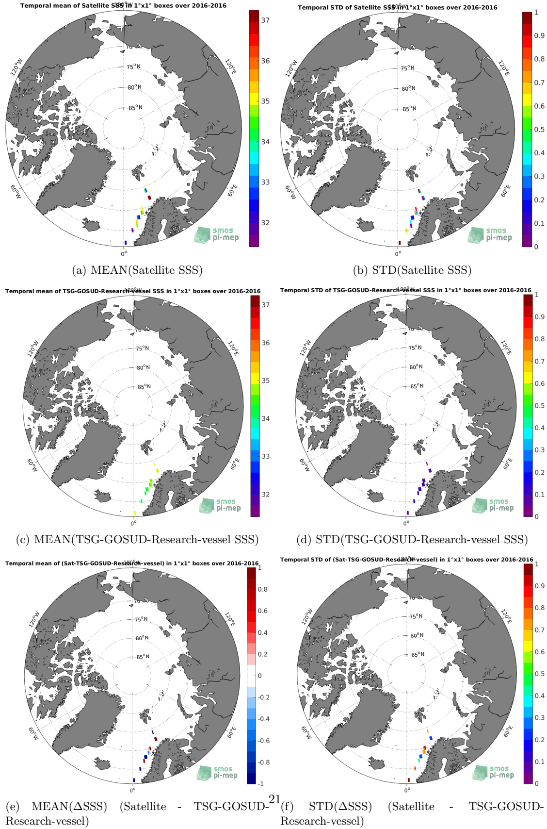
Figure 6: Temporal mean (left) and STD (right) of SSS from SMOS-L2-DPGS-v662 (top), TSG-GOSUD-Research-vessel (middle), and of \Delta SSS (Satellite - TSG-GOSUD-Research-vessel). Only match-up pairs are used to generate these maps.
