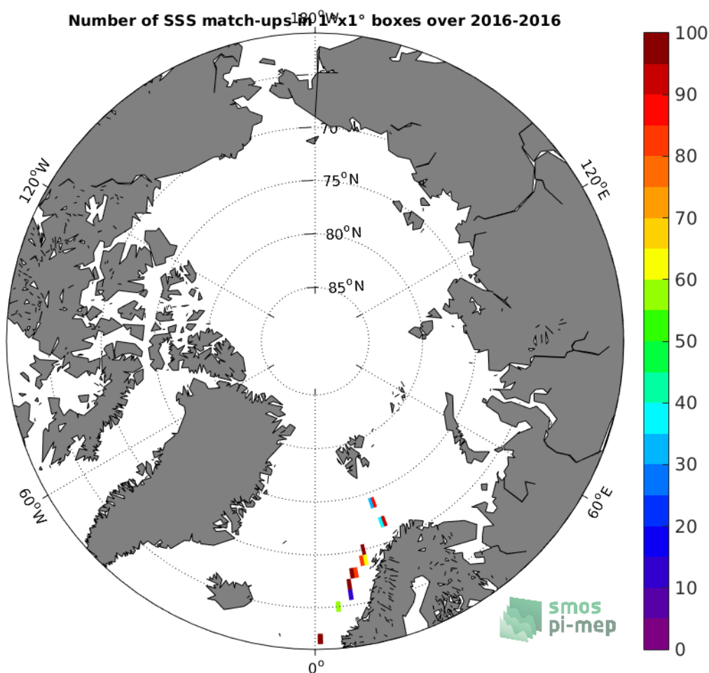
Figure 4: Number of SSS match-ups between TSG-GOSUD-Research-vessel SSS and the SMOS-L2-DPGS-v662 SSS product for the Arctic Ocean Pi-MEP region over 1°x1° boxes and for the full satellite product period.
