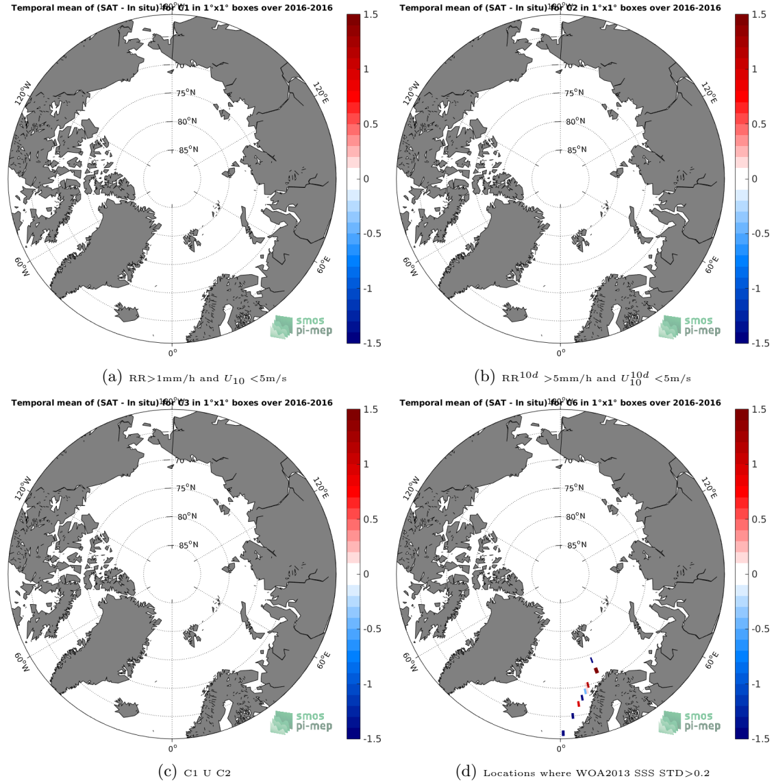
Figure 12: Temporal mean gridded over spatial boxes of size 1^\circ \times 1^\circ of \Delta SSS (SMOS-L2-DPGS-v662 - TSG-GOSUD-Research-vessel) for 4 different subdatasets corresponding to: RR > 1\text{mm/h} and U_{10} < 5\text{m/s} (a), RR^{10d} > 5\text{mm/h} and U_{10}^{10d} < 5\text{m/s} (b), C1 U C2 (c), Locations where WOA2013 SSS STD > 0.2 (d).
