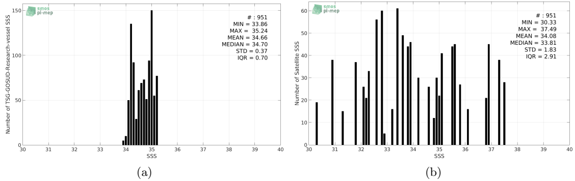
Figure 2: Histograms of SSS from TSG-GOSUD-Research-vessel (a) and SMOS-L2-DPGS-v662 (b) considering all match-up pairs per bins of 0.1 over the Arctic Ocean Pi-MEP region and for the full satellite product period.
