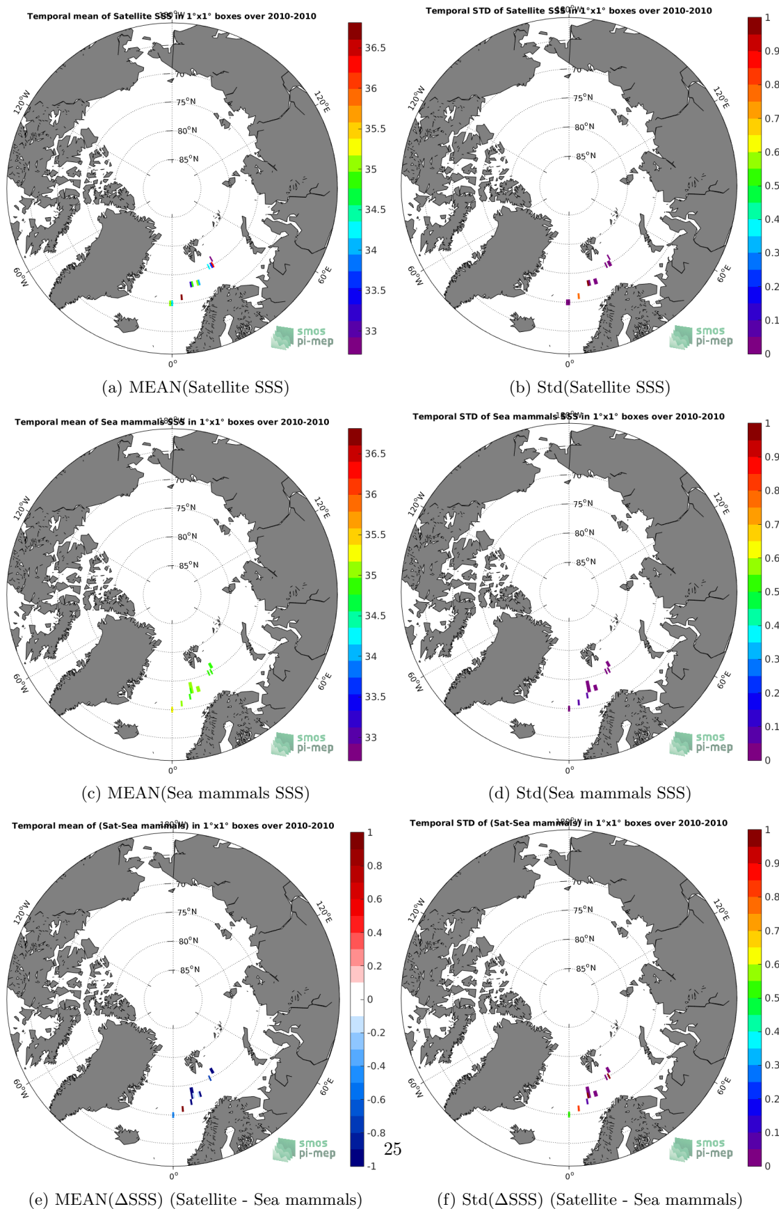
Figure 6: Temporal mean (left) and Std (right) of SSS from SMOS-L2-DPGS-v662 (top), Sea mammals (middle), and of \Delta SSS (Satellite - Sea mammals). Only match-up pairs are used to generate these maps.
