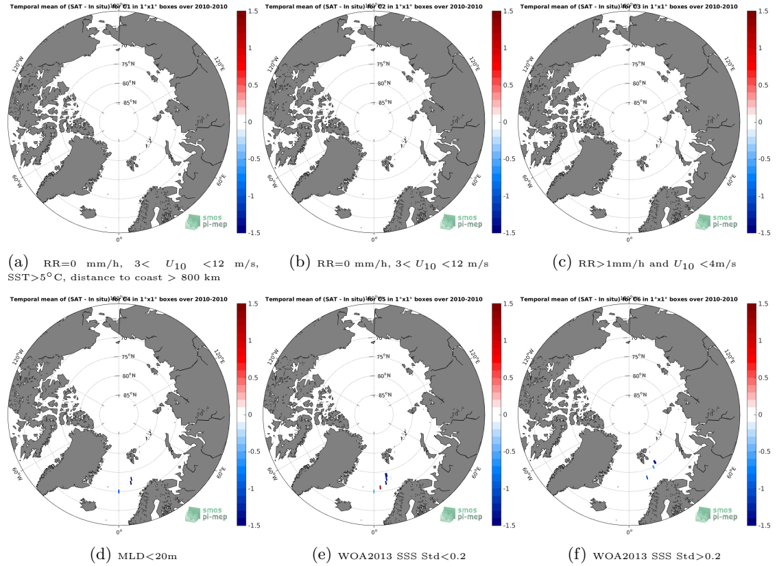
Figure 12: Temporal mean gridded over spatial boxes of size 1^\circ \times 1^\circ of \Delta SSS (SMOS-L2-DPGS-v662 - Sea mammals) for 6 different subdatasets corresponding to: RR=0 mm/h, 3 < U_{10} < 12 m/s, SST > 5^\circ C , distance to coast > 800 km (a), RR=0 mm/h, 3 < U_{10} < 12 m/s (b), RR > 1 mm/h and U_{10} < 4 m/s (c), MLD < 20 m (d), WOA2013 SSS Std < 0.2 (e), WOA2013 SSS Std > 0.2 (f).
