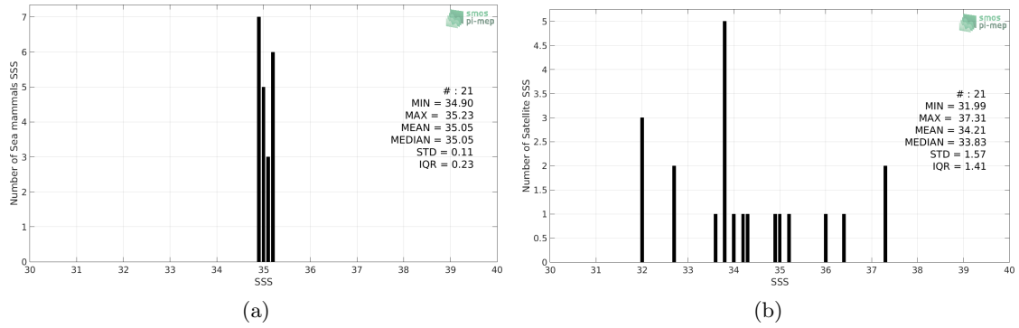
Figure 2: Histograms of SSS from Sea mammals (a) and SMOS-L2-DPGS-v662 (b) considering all match-up pairs per bins of 0.1 over the Arctic Ocean Pi-MEP region and for the full satellite product period.
