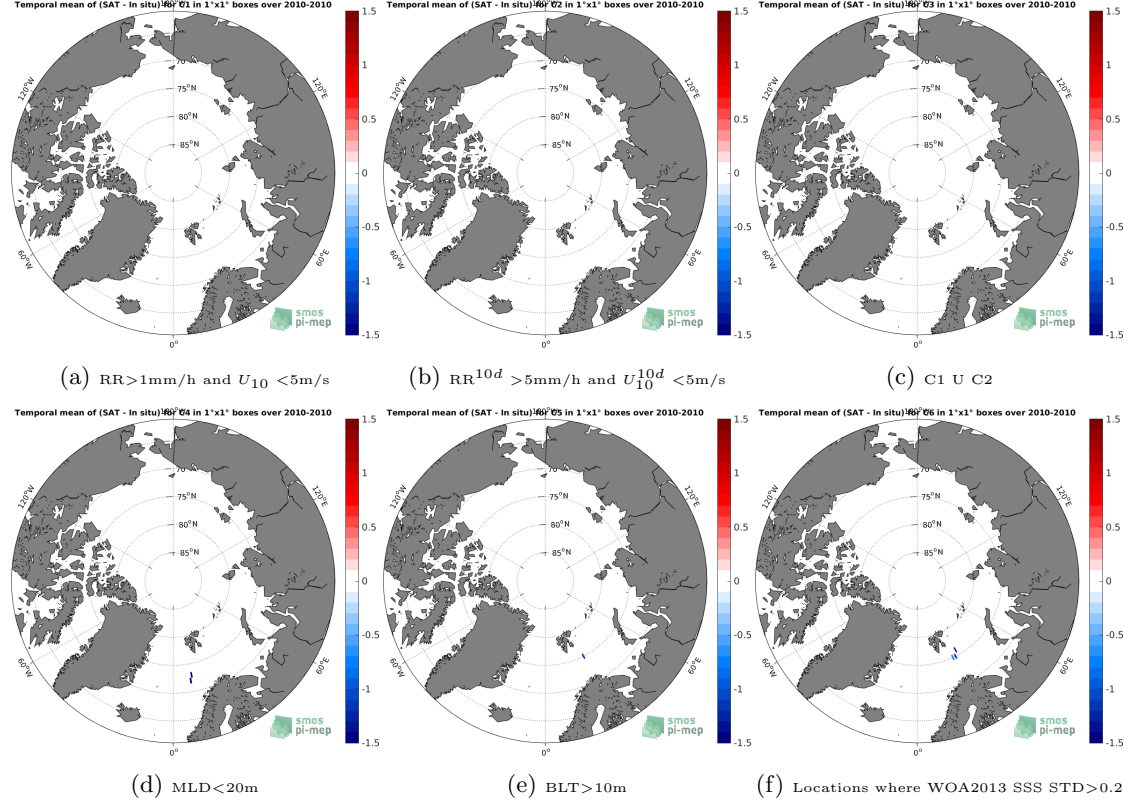
Figure 12: Temporal mean gridded over spatial boxes of size 1^\circ \times 1^\circ of \Delta\text{SSS} (SMOS-L2-DPGS-v662 - Sea mammals) for 6 different subdatasets corresponding to: \text{RR} > 1\text{mm/h} and U_{10} < 5\text{m/s} (a), \text{RR}^{10d} > 5\text{mm/h} and U_{10}^{10d} < 5\text{m/s} (b), C1 U C2 (c), \text{MLD} < 20\text{m} (d), \text{BLT} > 10\text{m} (e), Locations where WOA2013 SSS STD > 0.2 (f).
