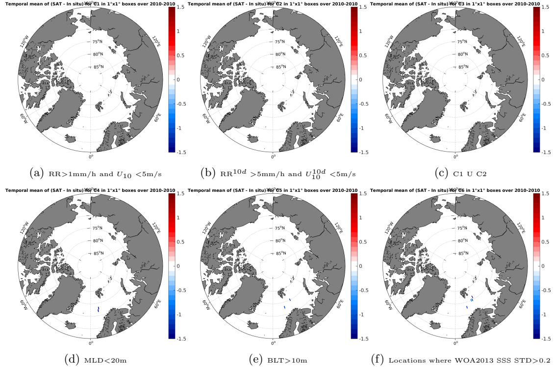
Figure 12: Temporal mean gridded over spatial boxes of size 1^\circ \times 1^\circ of \Delta SSS (SMOS-L2-DPGS-v662 - Sea mammals) for 6 different subdatasets corresponding to: RR > 1\text{mm/h} and U_{10} < 5\text{m/s} (a), RR^{10d} > 5\text{mm/h} and U_{10}^{10d} < 5\text{m/s} (b), C1 U C2 (c), MLD < 20\text{m} (d), BLT > 10\text{m} (e), Locations where WOA2013 SSS STD > 0.2 (f).
