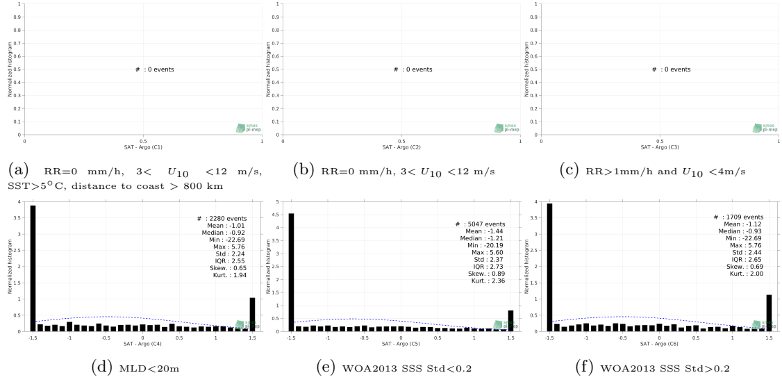
Figure 13: Normalized histogram of \Delta SSS (SMOS SSS L2 v662 (ESA) - Argo) for 6 different subdatasets corresponding to: RR=0 mm/h, 3 < U_{10} < 12 m/s, SST > 5°C, distance to coast > 800 km (a), RR=0 mm/h, 3 < U_{10} < 12 m/s (b), RR > 1mm/h and U_{10} < 4 m/s (c), MLD < 20m (d), WOA2013 SSS Std < 0.2 (e), WOA2013 SSS Std > 0.2 (f).
