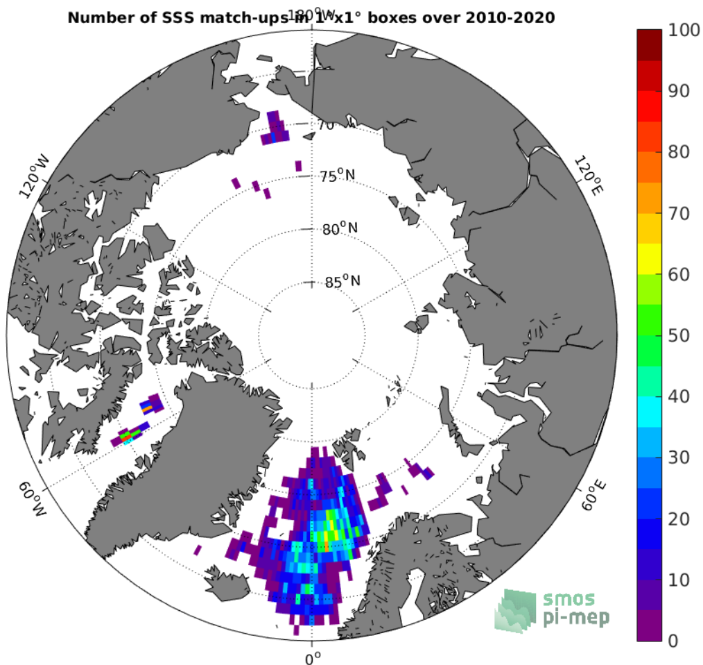
Figure 4: Number of SSS match-ups between Argo SSS and the SMOS SSS L2 v662 (ESA) SSS product for the Arctic Ocean Pi-MEP region over 1^\circ \times 1^\circ boxes and for the full satellite product period.
