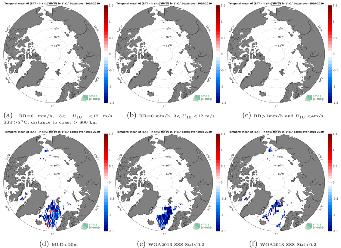
Figure 12: Temporal mean gridded over spatial boxes of size 1^{\circ}\times 1^{\circ} of \Delta\text{SSS} (SMOS SSS L2 v662 (ESA) - Argo) for 6 different subdatasets corresponding to:RR=0 mm/h, 3 < U_{10} < 12 m/s, SST >5^{\circ}\text{C} , distance to coast > 800 km (a), RR=0 mm/h, 3 < U_{10} < 12 m/s (b), RR >1 mm/h and U_{10} < 4 m/s (c),MLD <20 m (d),WOA2013 SSS Std <0.2 (e),WOA2013 SSS Std >0.2 (f).
