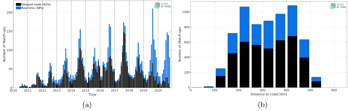
Figure 1: Number of match-ups between Argo and SMOS SSS L2 v662 (ESA) SSS as a function of time (a) and as function of the distance to coast (b) over the Arctic Ocean Pi-MEP region and for the full satellite product period.
