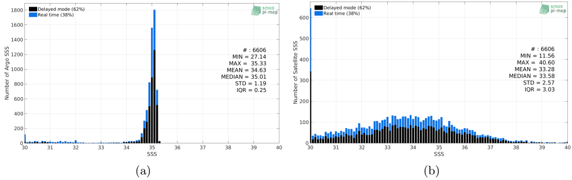
Figure 2: Histograms of SSS from Argo (a) and SMOS SSS L2 v662 (ESA) (b) considering all match-up pairs per bins of 0.1 over the Arctic Ocean Pi-MEP region and for the full satellite product period.
