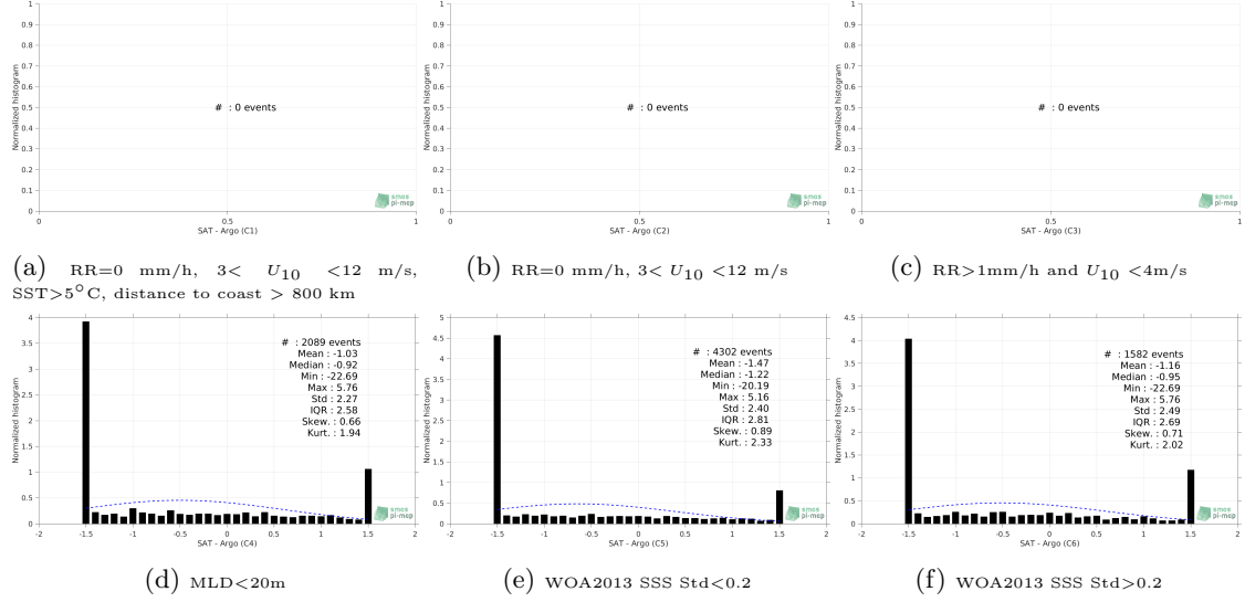
Figure 13: Normalized histogram of \Delta SSS (SMOS L2 v662 (ESA) - Argo) for 6 different sub-datasets corresponding to: RR=0 mm/h, 3 < U_{10} < 12 m/s, SST > 5^\circ\text{C} , distance to coast > 800 km (a), RR=0 mm/h, 3 < U_{10} < 12 m/s (b), RR > 1 mm/h and U_{10} < 4 m/s (c), MLD < 20 m (d), WOA2013 SSS Std < 0.2 (e), WOA2013 SSS Std > 0.2 (f).
