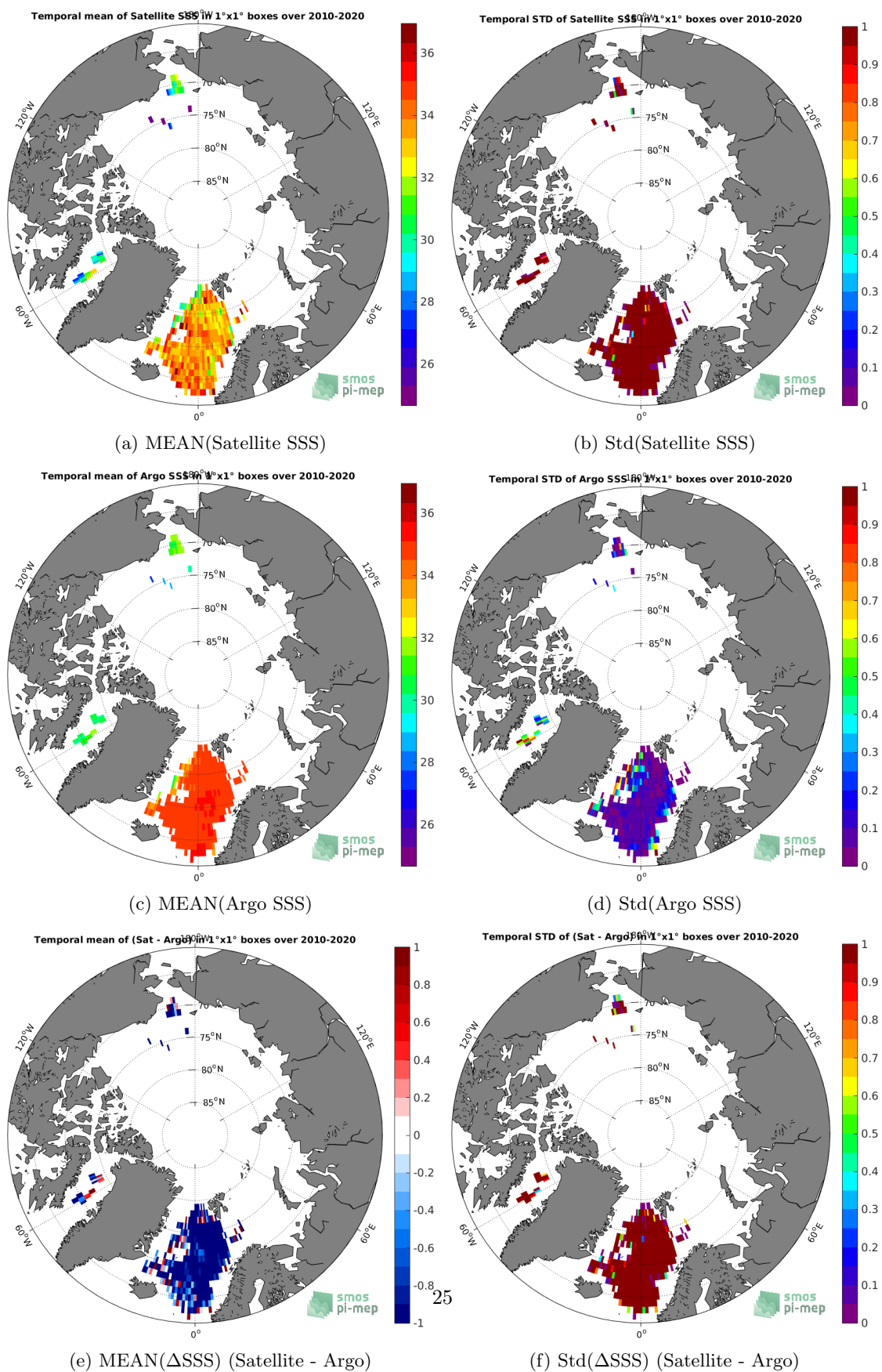
Figure 6: Temporal mean (left) and Std (right) of SSS from SMOS L2 v662 (ESA) (top), Argo (middle), and of \Delta SSS (Satellite - Argo). Only match-up pairs are used to generate these maps.
