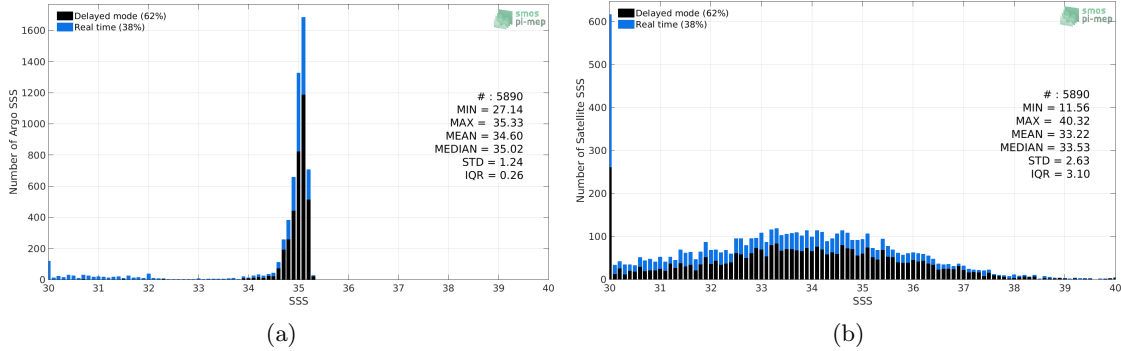
Figure 2: Histograms of SSS from Argo (a) and SMOS L2 v662 (ESA) (b) considering all match-up pairs per bins of 0.1 over the Arctic Ocean Pi-MEP region and for the full satellite product period.
