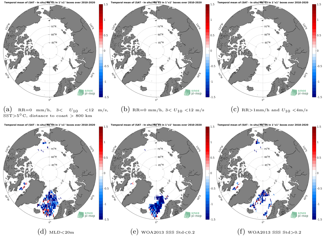
Figure 12: Temporal mean gridded over spatial boxes of size 1^{\circ}\times 1^{\circ} of \Delta\text{SSS} (SMOS L2 v662 (ESA) - Argo) for 6 different subdatasets corresponding to: RR=0 mm/h, 3 < U_{10} < 12 m/s, SST > 5^{\circ}\text{C} , distance to coast > 800 km (a), RR=0 mm/h, 3 < U_{10} < 12 m/s (b), RR > 1 mm/h and U_{10} < 4 m/s (c), MLD < 20\text{m} (d), WOA2013 SSS Std < 0.2 (e), WOA2013 SSS Std > 0.2 (f).
