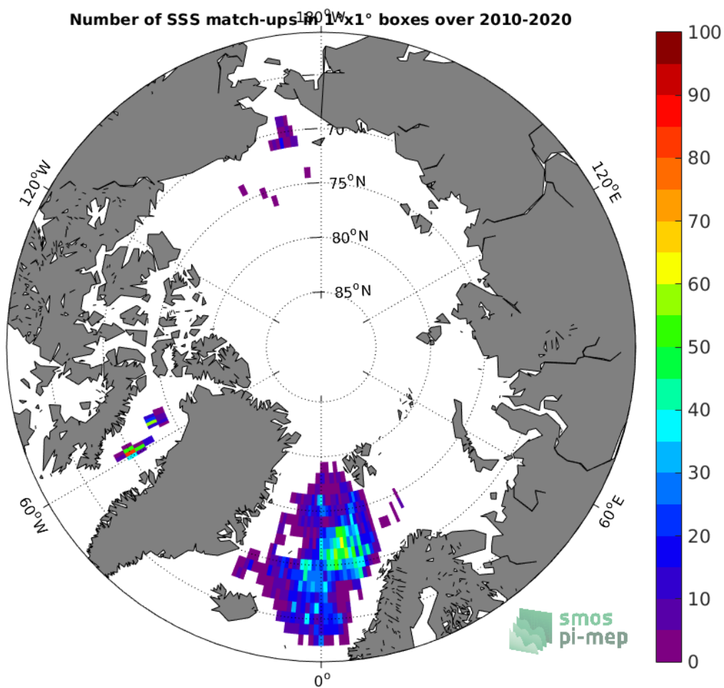
Figure 4: Number of SSS match-ups between Argo SSS and the SMOS L2 v662 (ESA) SSS product for the Arctic Ocean Pi-MEP region over 1^\circ \times 1^\circ boxes and for the full satellite product period.
