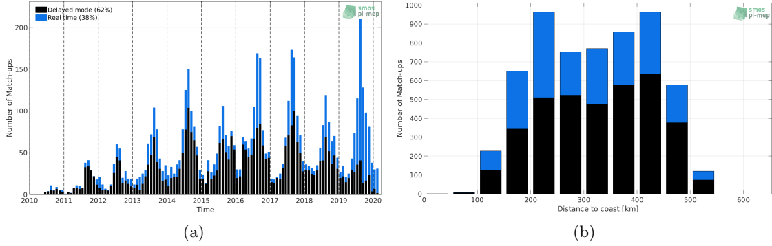
Figure 1: Number of match-ups between Argo and SMOS L2 v662 (ESA) SSS as a function of time (a) and as function of the distance to coast (b) over the Arctic Ocean Pi-MEP region and for the full satellite product period.
