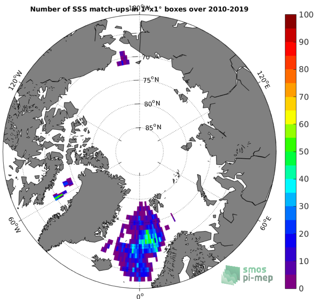
Figure 4: Number of SSS match-ups between Argo SSS and the SMOS-L2-DPGS-v662 SSS product for the Arctic Ocean Pi-MEP region over 1^\circ \times 1^\circ boxes and for the full satellite product period.
