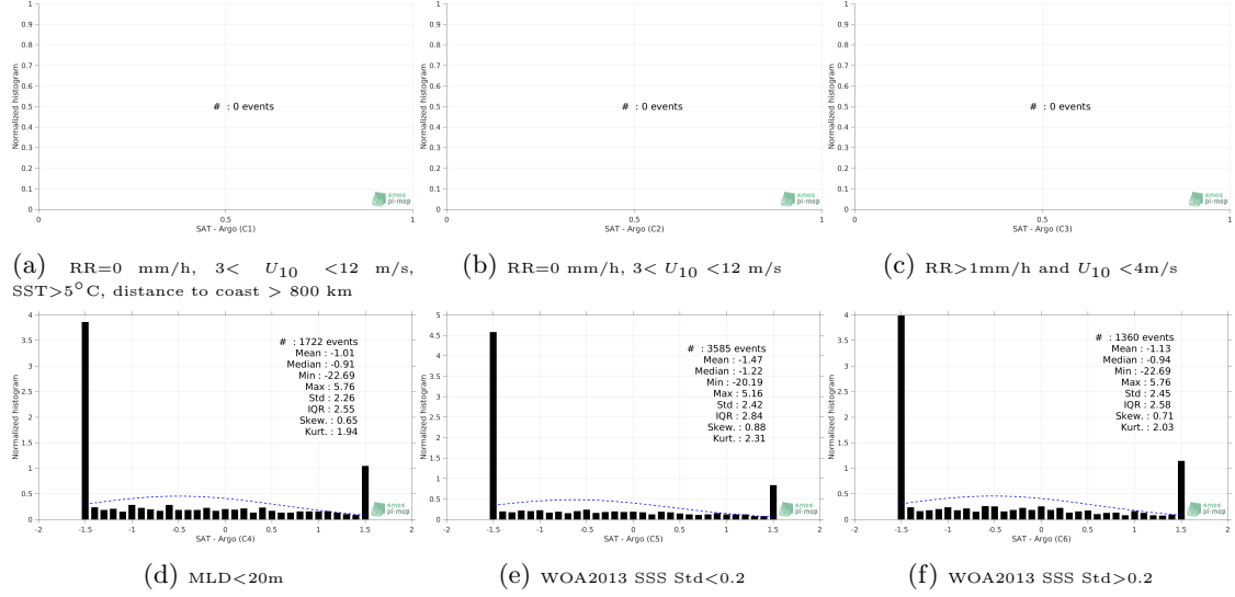
Figure 13: Normalized histogram of \Delta\text{SSS} (SMOS-L2-DPGS-v662 - Argo) for 6 different sub-datasets corresponding to: RR=0 mm/h, 3 < U_{10} < 12 m/s, SST > 5^\circ\text{C} , distance to coast > 800 km (a), RR=0 mm/h, 3 < U_{10} < 12 m/s (b), RR > 1\text{mm/h} and U_{10} < 4\text{m/s} (c), MLD < 20\text{m} (d), WOA2013 SSS Std < 0.2 (e), WOA2013 SSS Std > 0.2 (f).
