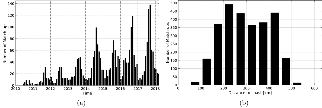
Figure 1: Number of match-ups between Argo and SMOS-L2-DPGS-v662 SSS as a function of time (a) and as function of the distance to coast (b) over the Arctic Ocean Pi-MEP region and for the full satellite product period.
