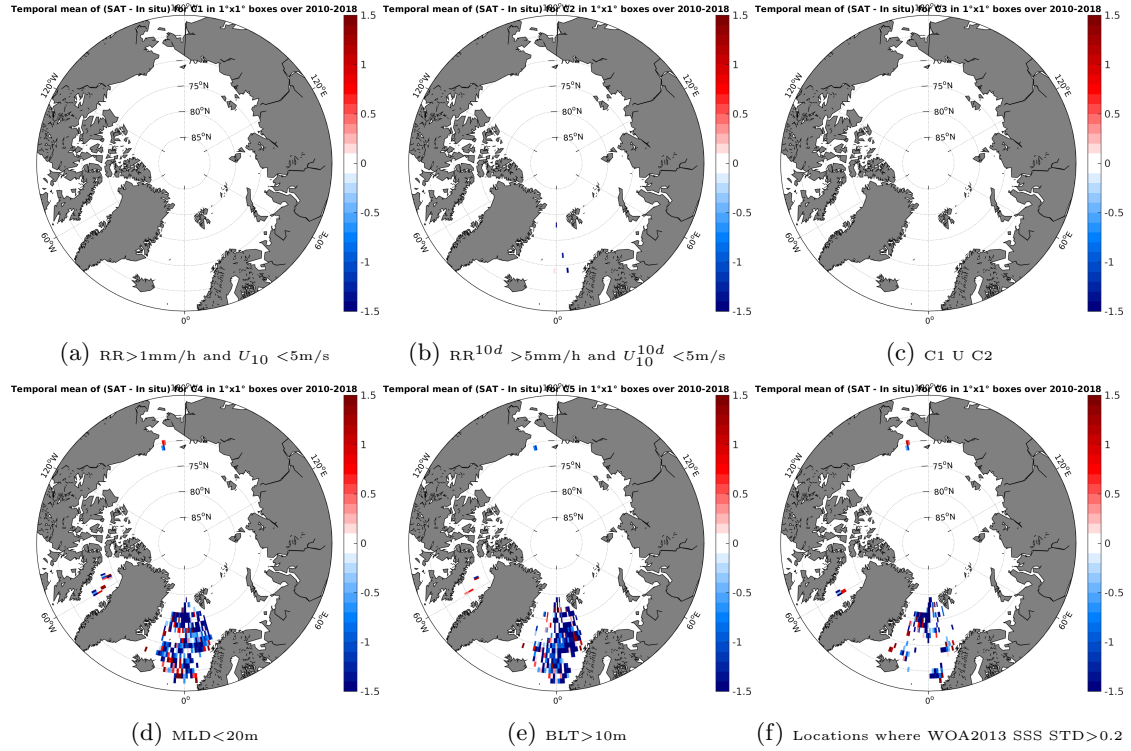
Figure 12: Temporal mean gridded over spatial boxes of size 1^\circ \times 1^\circ of \Delta\text{SSS} (SMOS-L2-DPGS-v662 - Argo) for 6 different subdatasets corresponding to: \text{RR} > 1\text{mm/h} and U_{10} < 5\text{m/s} (a), \text{RR}^{10d} > 5\text{mm/h} and U_{10}^{10d} < 5\text{m/s} (b), C1 U C2 (c), \text{MLD} < 20\text{m} (d), \text{BLT} > 10\text{m} (e), Locations where WOA2013 SSS STD > 0.2 (f).
