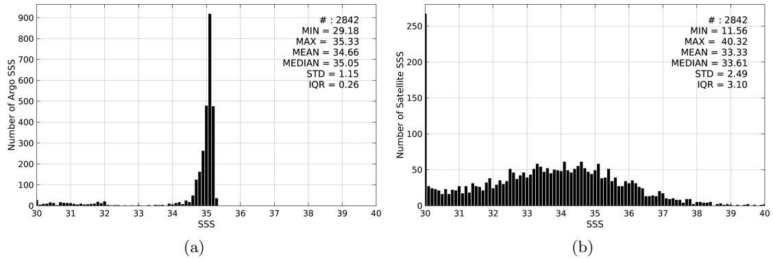
Figure 2: Histograms of SSS from Argo (a) and SMOS-L2-DPGS-v662 (b) considering all match-up pairs per bins of 0.1 over the Arctic Ocean Pi-MEP region and for the full satellite product period.
